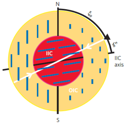
Figure 13: Equatorial anisotropy of the Earth’s inner core 47
