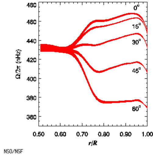
Figure 38: Sun rotation rates 106
