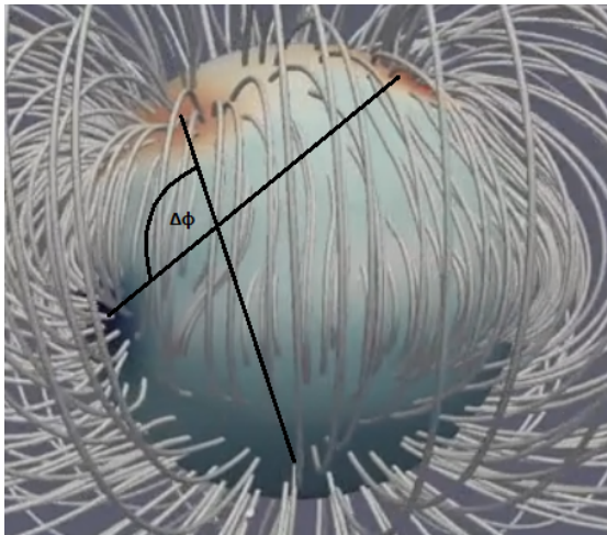
Figure 14: Magnetic field of Jupiter 48
