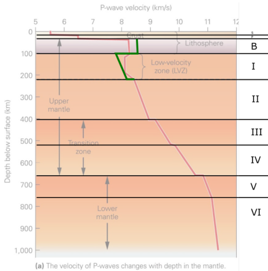
Figure 17: Layers of Earth’s brain, superimposed on seismic velocities 58
