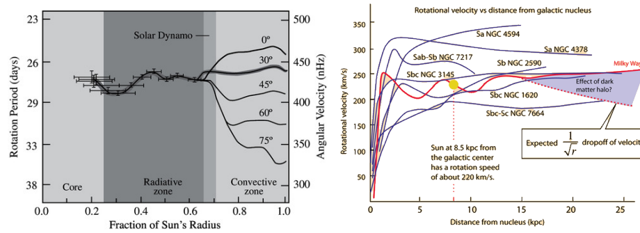
Figure 7: left) internal rotation of the Sun 29 , right) rotation of spiral galaxies 30
