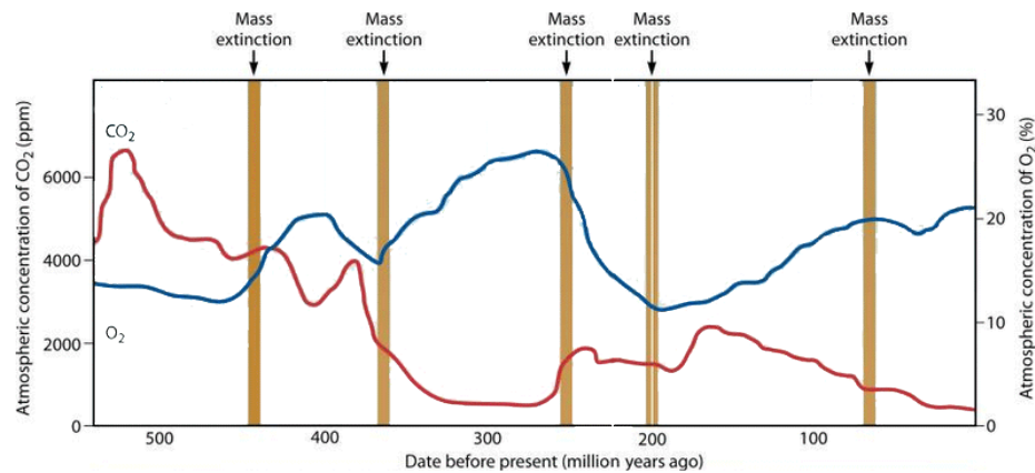
Figure 18: The history of atmospheric CO 2 concentration 61
