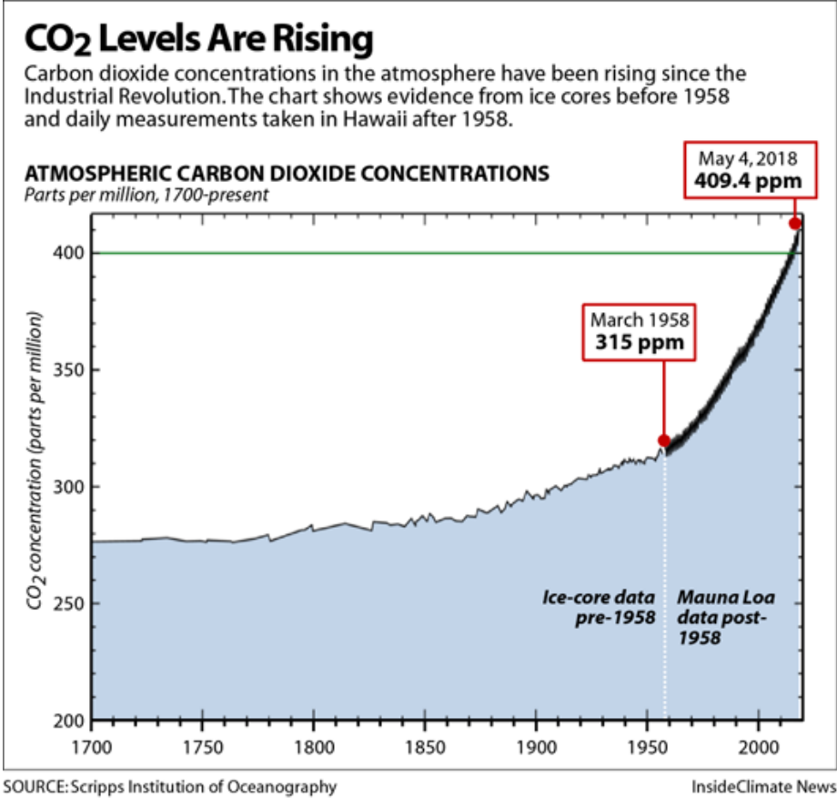
Figure 20: Recent history of CO 2 concentration 66
