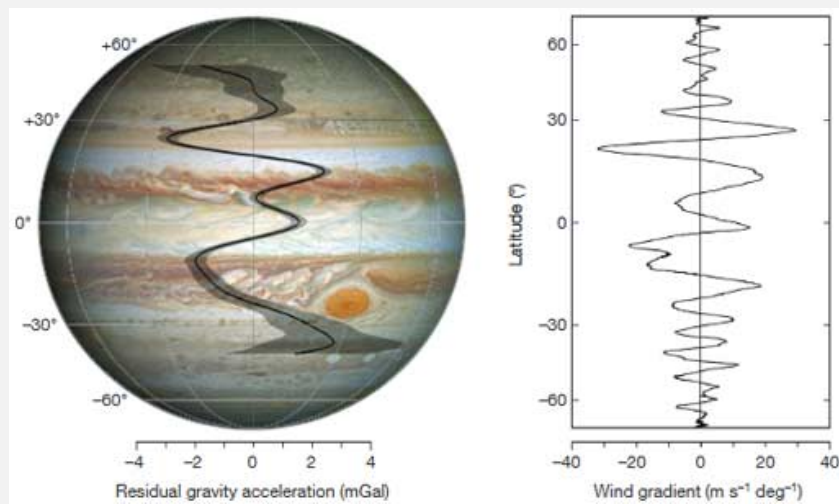
Figure 29: Jupiter gravity disturbances and wind gradient 92
