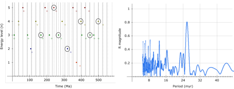
Figure 25: Extinctions (left), spectral analysis (right)
