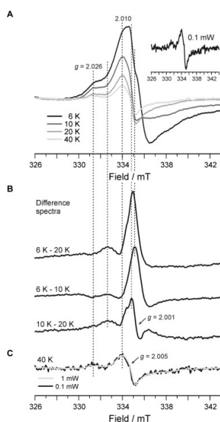
Figure 3. Temperature dependency of the organic radical formed in Dictyostelium DyPA after addition of \text{H}_2\text{O}_2 . (A) Temperature dependency of the g \approx 2.00 signal originating from the organic radicals observed in Dictyostelium DyPA after reaction with \text{H}_2\text{O}_2 . The right inset shows the spectrum recorded at 40 K under non-saturating conditions (microwave power = 0.1 mW, modulation amplitude = 0.1 mT, 15 averages) from the same sample. (B) Difference spectra from the temperature dependency data shown in panel A after correction for temperature effects only on signal amplitude (due to temperature effects on the Boltzmann distribution of spin states). The (6 K – 20 K) difference spectrum contains all components stable at T < 20 K, and the (6 K – 10 K) difference spectrum the components stable only at T < 10 K. The (10 K – 20 K) difference spectrum shown at the bottom consequently displays those components still present at 10 K but being absent at 20 K. (C) Overlay of the 40 K spectra recorded with microwave powers of 1 mW (from panel A) and 0.1 mW (from inset in panel A). The 1 mW 40 K spectrum resembles the 20 K spectrum besides its lower amplitude. The small signal at g = 1.974 ( B \approx 340 mT) observed in the spectra recorded at 40 K is not further addressed here due to its very low intensity. Vertical lines (dashed) are drawn to guide the eye.
