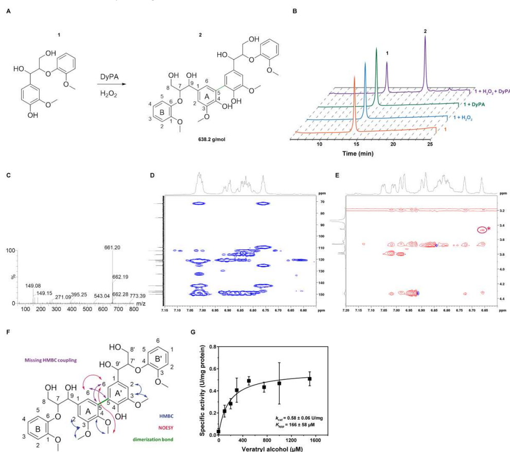
Figure 5. Oxidation of lignin model substrate (GGBGE) by Dictyostelium DyPA. (A) Structure of the \beta -aryl ether lignin model substrate ( 1 ) and the proposed dimeric product ( 2 ). (B) Reverse HPLC profiles monitoring substrate turnover in the absence and presence of DyPA and \text{H}_2\text{O}_2 . The absorbance of substrate and product was detected at 254 nm. (C) ESI-MS of 2 nd HPLC peak with an experimental m/z value for the Na adduct of 661.20. The calculated value corresponds to 661.2261. (D) The structure of the catalyzed dimerization of GGBGE by DyPA is demonstrated by a 2D HMBC experiment. This spectrum shows the proposed structure, in particular the coupling of H15 (= 6.77 ppm) to A5 (= 125.9 ppm). However, due to the fact that it is a symmetrical molecule, the two distinguished ring systems A and A' cannot be clearly distinguished. (E) The structural elucidation of the asymmetric methoxy derivative is based on NOE spectroscopy. The spectrum shows the introduced interaction between the methoxy group ( d = 3.45 ppm) and C15'-H ( d = 6.66 ppm), marked with a star. (F) The coupling scheme of GGBGE of the HMBC (blue arrows) and NOESY (red arrows) experiments. The green bond indicates the dimerization bond as the result of the Dictyostelium DyPA mediated dimerization. The blue methoxy group is introduced by derivatization to create the asymmetry, the NOE-signal of this asymmetry is indicated by a red star. The purple arrows indicate missing HMBC couplings for the methoxy derivative. (G) Oxidation of veratryl alcohol by Dictyostelium DyPA. Data are average values of 3–6 independent measurements and error bars represent the standard deviations.
