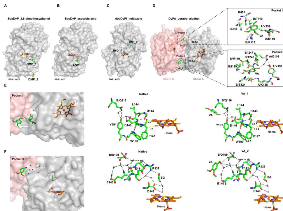
Figure 8. Overview of veratryl alcohol binding sites on Dictyostelium DyPA. (A) DMP binding sites in BadDyP :DMP (PDB: 3VXJ) complex structure. (B) Ascorbic acid binding site in BadDyP :ASC (PDB: 3VXI) complex structure. (C) Imidazole binding sites in AauDyPI :IMD (PDB: 4UZI) complex structure. (D) Veratryl alcohol binding sites in Dictyostelium DyPA:VA complex structure. The distance between the iron atom of heme moiety and the oxygen atom of the veratryl alcohol hydroxyl group is indicated by a dashed line. The lower inset shows a superimposition of substrate-free and veratryl alcohol bound Dictyostelium DyPA structures for the binding site I, while the upper inset shows binding site II. Carbon atoms in the substrate-free structure are represented in white and carbon atoms in the Dictyostelium DyPA:VA complex are shown in green. (E-F) Proposed long-range electron transfer pathways from veratryl alcohol binding sites I and II to the heme moiety of Dictyostelium DyPA. Position of the Dictyostelium DyPA veratryl alcohol binding site I/II relative to the heme cofactor
