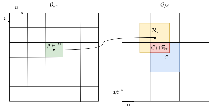
Figure 3. Mapping of measurements with assigned object label from image to u-disparity/-depth grid.
