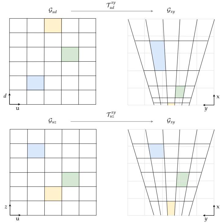
Figure 5. In the cartesian grid on the right-hand side, the grid cells are influenced by the distorted overlaid areas based on the corresponding u-disparity or u-depth grid cell respectively.
