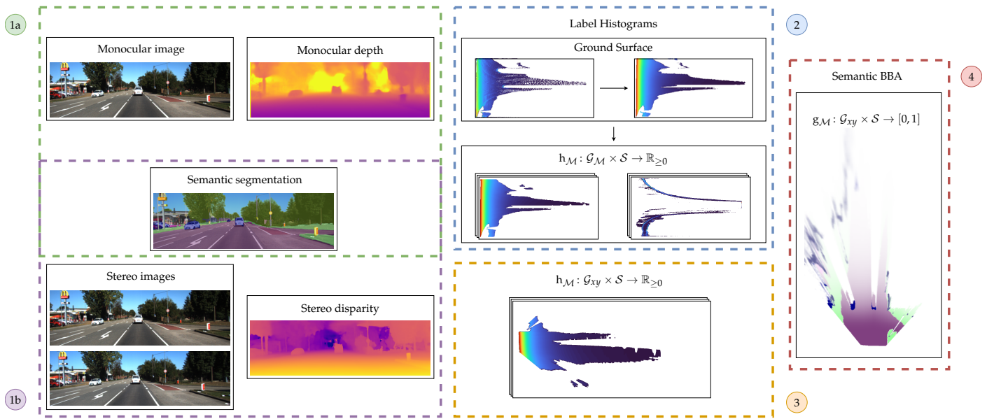
Figure 1. Overview of the described grid mapping framework. On the front end either monocular images are processed to obtain depth maps (1a) or stereo images are used to estimate a disparity map (1b). Either of them is accompanied by a pixelwise semantic segmentation image. The images are used as input for a label histogram calculation in a setup-dependant grid in the second step (2). This label histogram is transformed into a cartesian grid (3) and finally transformed into a semantic evidential grid map (4).
