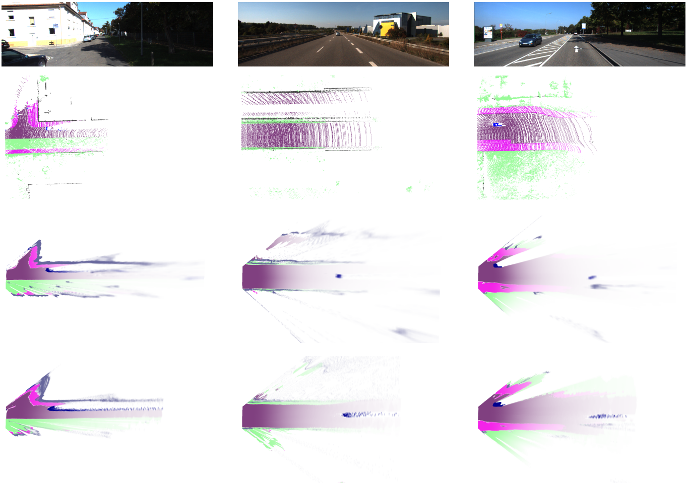
Figure 8. The resulting BBA for stereo and mono images. Each column corresponds to one frame in the Kitti odometry benchmark depicted in the image in the first row. The second row shows the ground truth, the third row results for stereo vision and the last row for mono vision.
