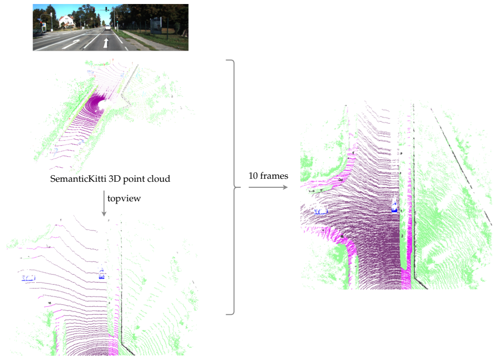
Figure 7. The generation of the ground truth used for the quantitative evaluation. 3D semantic point clouds from ten frames are merged and mapped into a top-view grid.
