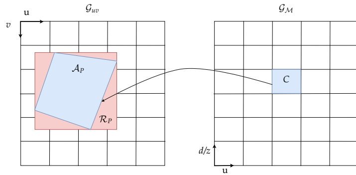
Figure 4. Mapping of measurements with assigned ground label from image to u-disparity/-depth grid.
