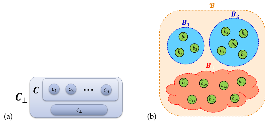
Figure 2. Model of classical digital computational states (at some particular time t = \tau_\ell \in \mathbb{R} ). (a) Abstract computational states of a physical computer system \mathfrak{G} with n distinct states. The “catch-all” state c_\perp represents the condition that the physical state of \mathfrak{G} is such that the computational state is not otherwise well-defined. (b) Basis sets B_i corresponding to the computational states c_i , where i \in \{\perp, 1, \dots, n\} . Here, n = 2 . These basis sets partition the complete proto-computational basis \mathcal{B} .
