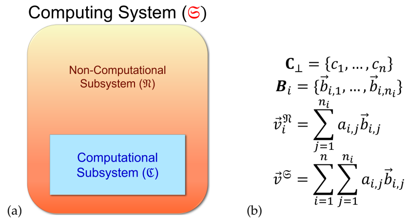
Figure 3. (a) Breakdown of the computing system \mathfrak{S} into computational ( \mathfrak{C} ) and non-computational ( \mathfrak{N} ) subsystems. The Hilbert space of \mathfrak{S} can be expressed as either a product \mathcal{H}^{\mathfrak{S}} = \mathcal{H}^{\mathfrak{C}} \otimes \mathcal{H}^{\mathfrak{N}} of subsystem subspaces, or more generally as a subspace sum \mathcal{H}^{\mathfrak{S}} = \bigoplus_{c \in \mathbf{C}_\perp} \mathcal{H}_c^{\mathfrak{N}} . (b) A general vector \vec{v}^{\mathfrak{S}} in a system Hilbert space \mathcal{H}^{\mathfrak{S}} that is defined as a sum of the non-computational Hilbert spaces \mathcal{H}_i^{\mathfrak{N}} corresponding to the n individual computational states c_i \in \mathbf{C}_\perp can be obtained by simply summing general vectors \vec{v}_i^{\mathfrak{N}} within the individual subspaces \mathcal{H}_c^{\mathfrak{N}} , treating the basis vectors \vec{b}_{i,j} across all n subspaces as mutually orthogonal. Note that the dimensionalities n_i of the component subspaces do not all have to be the same in general.
