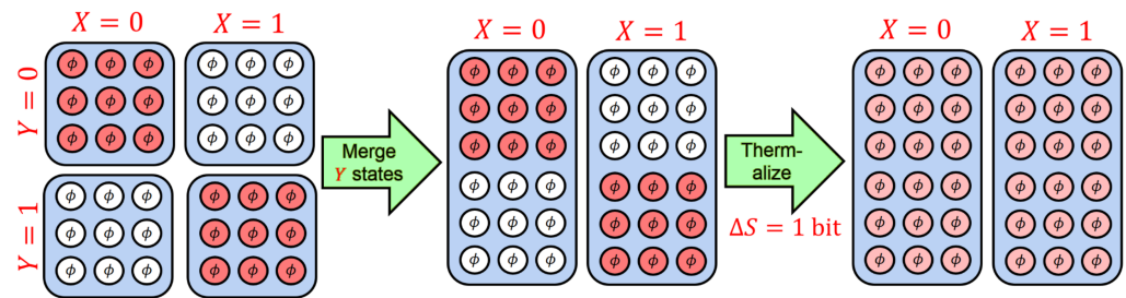
Figure 11. Landauer's Principle as entropy increase from thermalization of mutual information. Red shading denotes probability density. (Left) Two perfectly-correlated computational bit-systems \mathcal{X} and \mathcal{Y} ; their states could have been prepared by computing \mathcal{Y} 's value y deterministically from x , e.g., using y := x . (Middle) When the variable Y (for the computational state of \mathcal{Y} ) is obliviously erased, this amounts to merging the two computational states in each column; we can say that now Y = 0 (say) in each merged state. Note that now, there briefly exists a correlation between X and the non-computational part of the physical state. (Right) Very quickly (over a thermalization timescale), we lose track of the probabilities of the different physical states making up each computational state, thus losing this correlation information. This is where the absolute increase of total entropy from Landauer's Principle necessarily occurs. We cannot, of course, then undo this entropy increase by simply reversing the first step (un-merging the Y states), because the correlation information between X and Y has already been irrevocably lost by this point.
