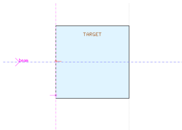
Figure 2 Physical model x-z section of air sample and Virion Particles
