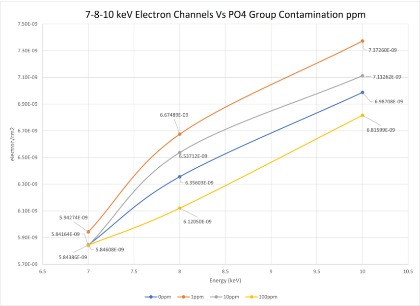
Figure 16 Low Band Electron Spectrum - Air Sample Vs Contamination
