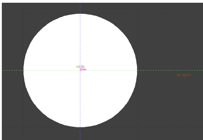
Figure 4 Geometry Region Modelling -Target, Void, Black hole
