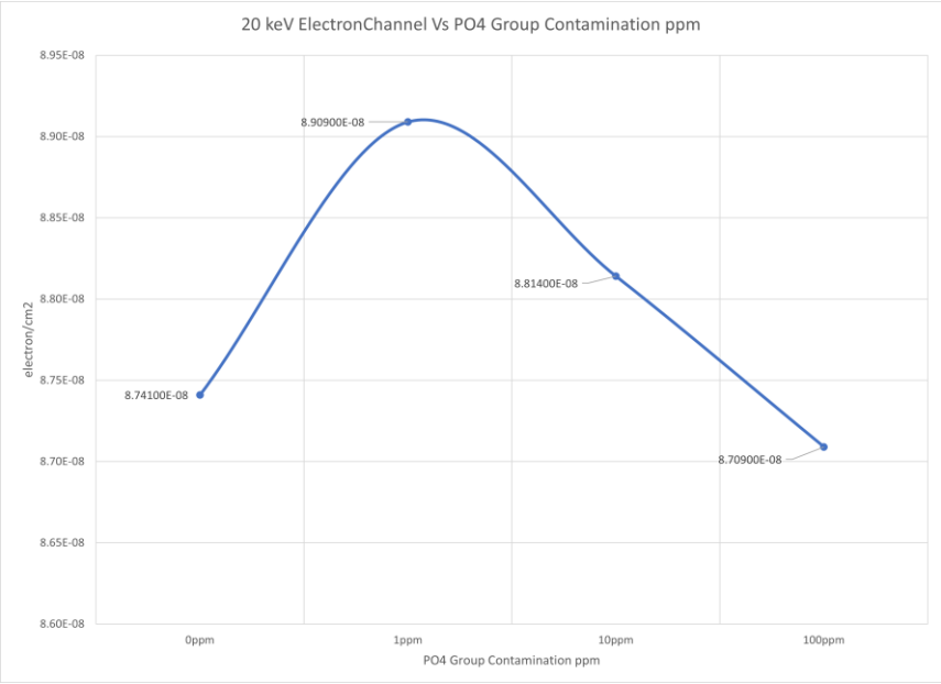
Figure 17 Electron 20 keV Channel - Air Sample Vs Contamination
