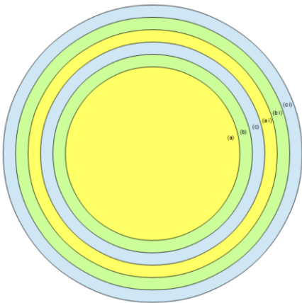
Figure 8 Virion Cluster, x-z section model
