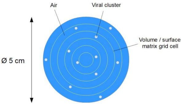
Figure 5 Geometrical model x-z section
