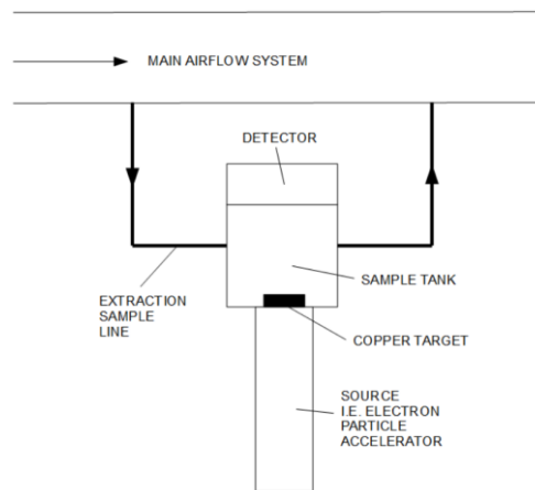
Figure 22 Detection - Design and set-up
