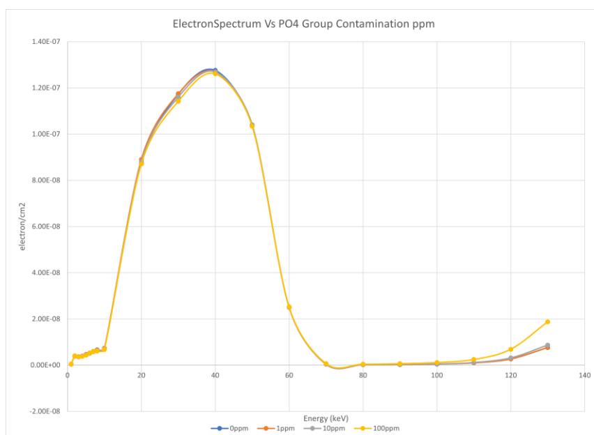
Figure 18 Electron Spectrum - Air Sample Vs Contamination
