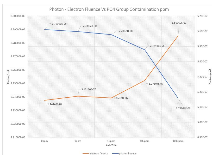
Figure 9 Fluences - Photon and Electron Vs Contamination
