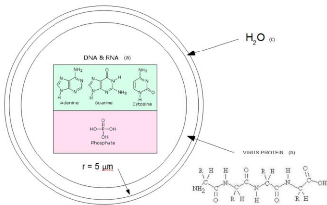
Figure 1 Virion Particle Modelling
