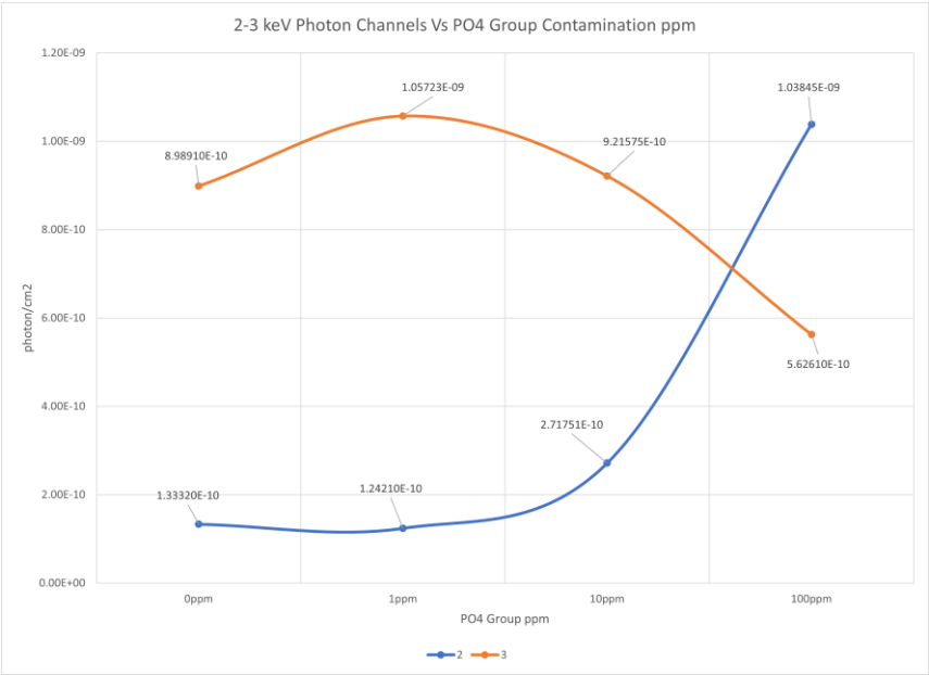
Figure 12 Photon Channel 2-3 keV Vs Contamination
