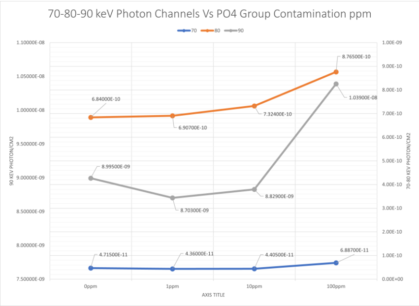
Figure 14 High Band Photon Spectrum B1 - Air Sample Vs Contamination
