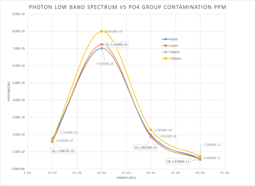
Figure 11 Low Band Photon Spectrum B - Air Sample Vs Contamination
