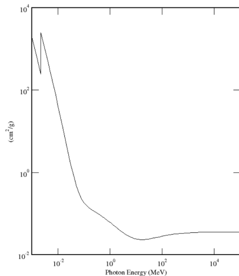
Figure 21 Phosphorus Photon Cross Section
