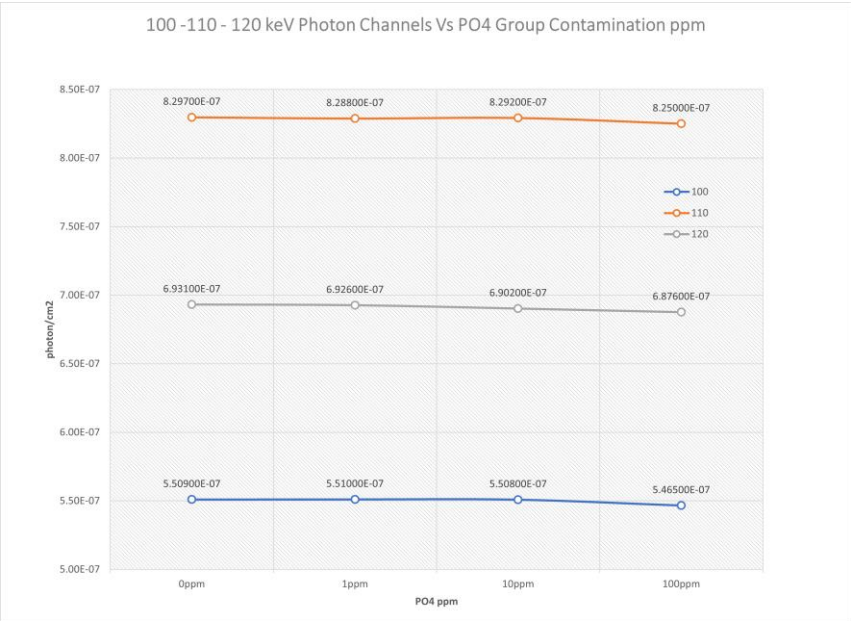
Figure 15 High Band Photon Spectrum B2 - Air Sample Vs Contamination
