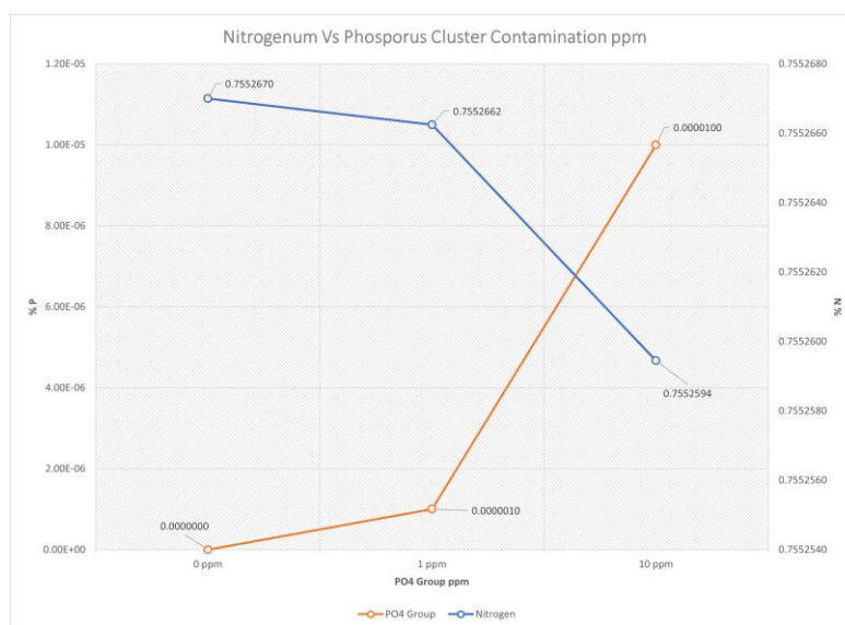
Figure 19 N Vs P Cluster Contamination 0-10 ppm
