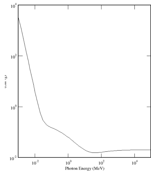
Figure 20 Nitrogen Photon Cross Section
