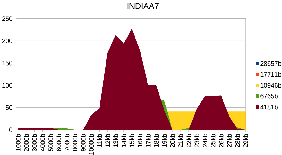
Figure 8 - INDIAA7 genome metastructures.
