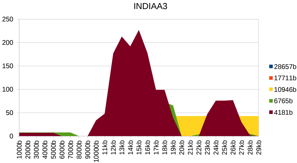
Figure 4 - INDIAA3 genome metastructures.
