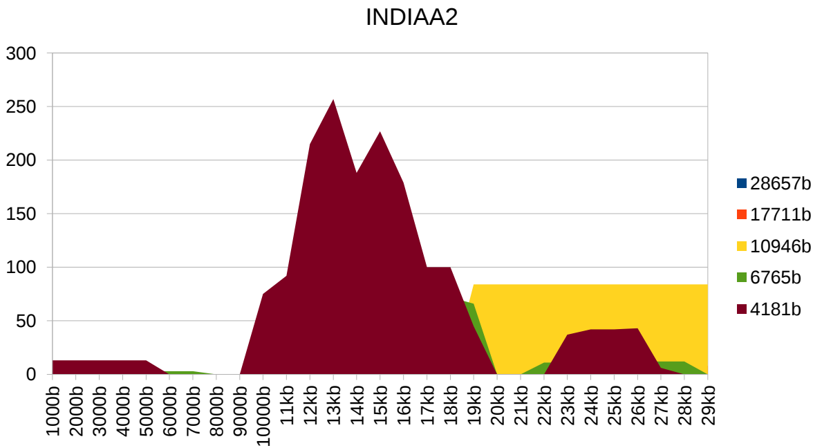
Figure 3 - INDIAA2 genome metastructures.
