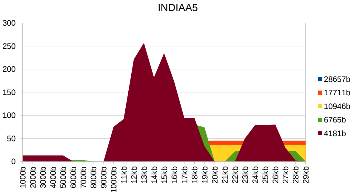
Figure 6 - INDIAA5 genome metastructures.
