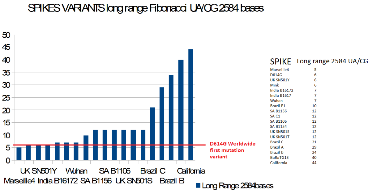
Figure 17 - Comparing 19 Spikes from 19 variants for long range 2584 UA/CG and 1597 UA/CG Balancing/Unbalancing « Podium » like metastructures.
