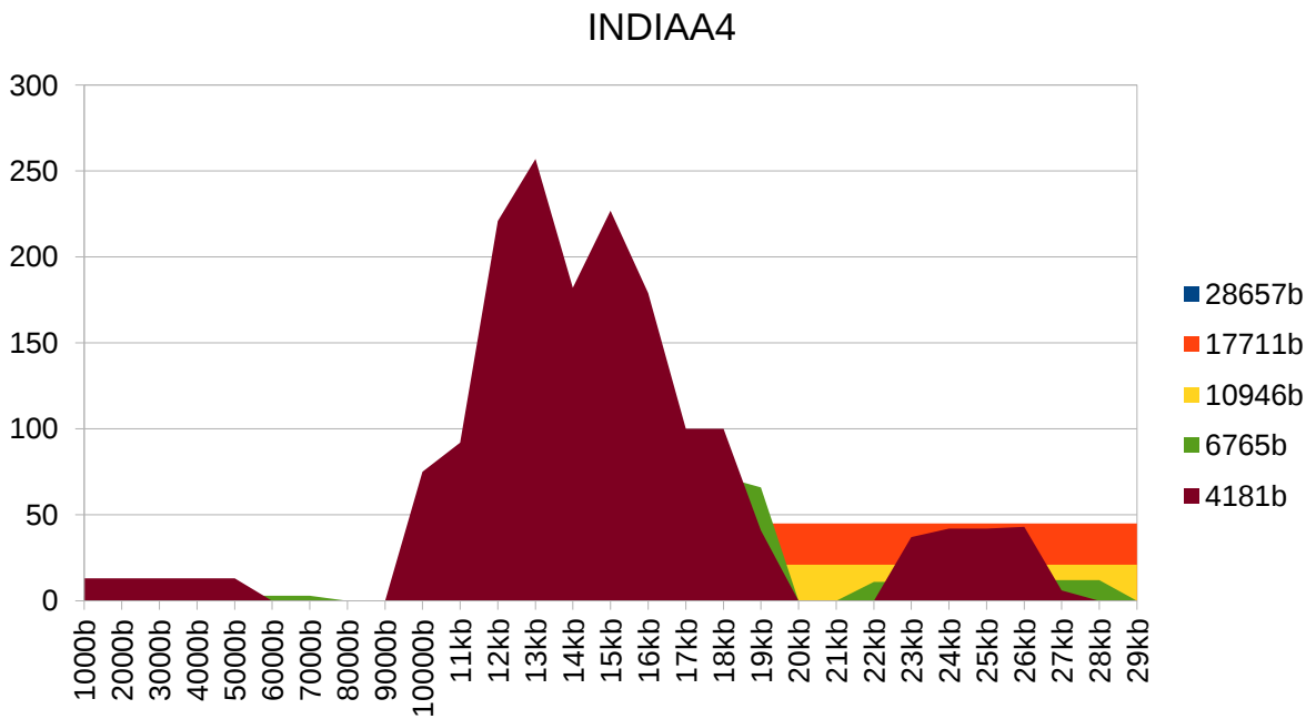
Figure 5 - INDIAA4 genome metastructures.
