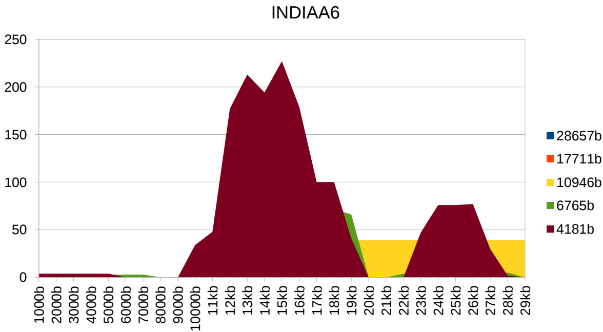
Figure 7 - INDIAA6 genome metastructures.
