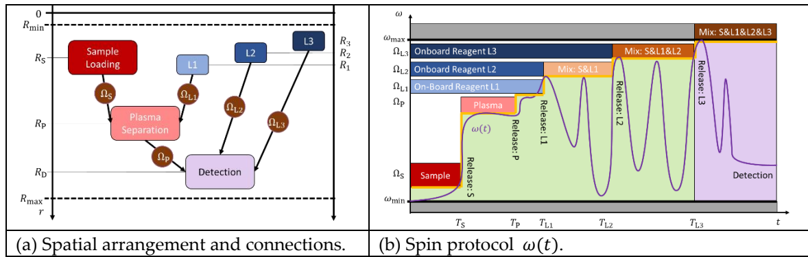
Figure 6 Exemplary bioassay implementing the loading of blood sample, plasma separation, and mixing with three prestored liquid reagents \{L_i\} . Flow is controlled by five high-pass valves with release rates \omega_{\min} < \Omega_i < \omega_{\max} located at R_{\min} < R_i < R_{\max} and opening for \omega > \Omega_i at points in time T_i . (a) Plasma (P) is extracted from the sample (S) in a peripheral position R_P at high field strength f_\omega \propto R_P \cdot \omega^2 (1). While, owing to the unidirectional nature of the centrifugal field f_\omega (1), the course of the assay requires R_S < R_P < R_D and R_{L1} < R_P , a radially inbound staggering R_{L1} > R_{L2} > R_{L3} (Figure 5b) has been chosen for the serial release of \{L_i\} through their high-pass valves opening at \Omega_{L1} < \Omega_{L2} < \Omega_{L3} . (b) A blood sample S is loaded and released at \Omega_S < \omega < \Omega_P . Separation of plasma P proceeds at \Omega_P < \omega < \Omega_{L1} . Onboard liquid reagent L1 is then forwarded at \Omega_{L1} < \omega < \Omega_{L2} into the separation chamber where it is mixed with the plasma P within \omega_{\min} < \omega < \Omega_{L2} . The mixture P&L1 then progresses to the final detection chamber for \Omega_P < \omega < \Omega_{L2} , followed by addition of and mixing with L2 within \Omega_2 < \omega < \Omega_3 and \omega_{\min} < \omega < \Omega_{L3} , respectively. Finally, L3 is added at \Omega_3 < \omega < \omega_{\max} and blended to obtain S&L1&L2 within \omega_{\min} < \omega < \omega_{\max} . The green background marks the allowed frequency corridor at each point in time t = T_i , with its upper limit expanding according to \omega_{\min} < \Omega_S < \Omega_P < \Omega_{L1} < \Omega_{L2} < \Omega_{L3} < \omega_{\max} . Note that, for the sake of simplicity, the frequency thresholds \{\Omega_i\} are meant to refer to their associated bands \Omega_i \pm M \cdot \Delta\Omega_i .
