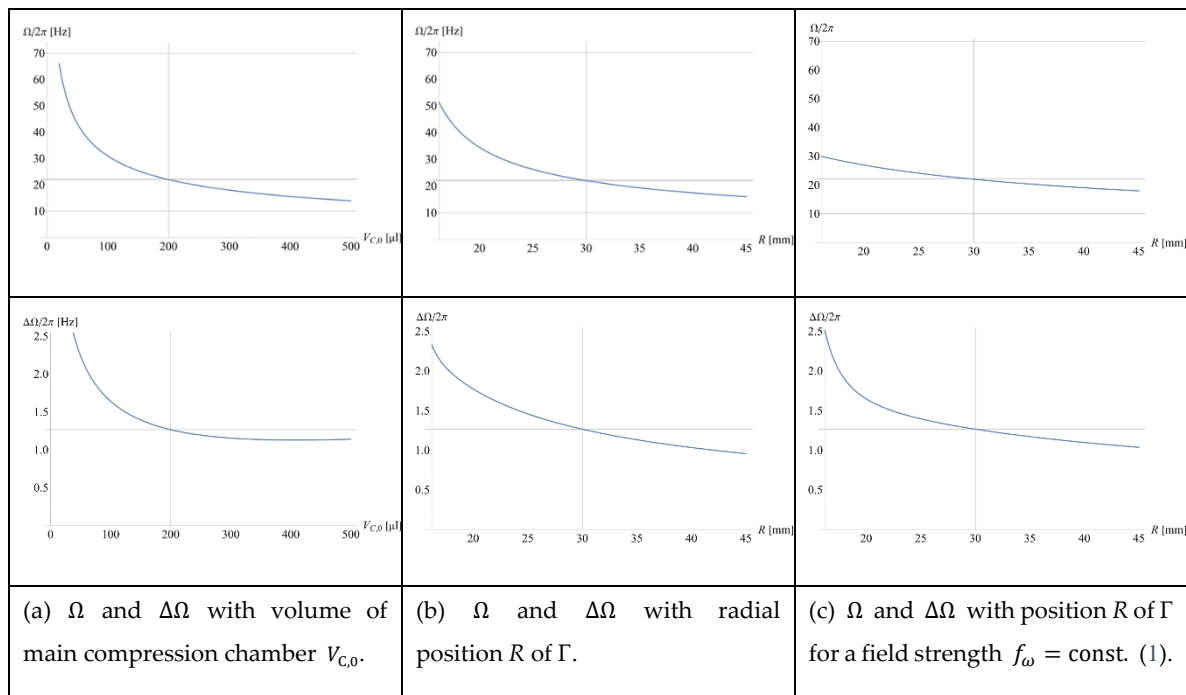
Figure 2 Variation of retention rate \Omega (11) and its standard deviation \Delta\Omega (20) with (a) the volume of the main, permanently gas filled compartment of the compression chamber V_{C,0} and (b) the radial position R while leaving (the remainder of) the structure \Gamma unchanged. The retention rate \Omega sharply increases towards shrinking compression volumes V_{C,0} and central placements R ; this comes at the expense of widening the tolerance \Delta\Omega . The gridlines represent the default volume V_{C,0} = 200 \mu\text{l} , at a radial position R = 30 \text{ mm} and retention rate \Omega/2\pi \approx 22 \text{ Hz} . (c) \Omega and \Delta\Omega vs R while maintaining the field strength f_\omega (1), originally evaluated for its default geometry \Gamma (Table A1), critical spin rate \Omega/2\pi = 30 \text{ Hz} , \rho = 1000 \text{ kg m}^{-3} and R = 3 \text{ cm} , while varying the radial position R .
