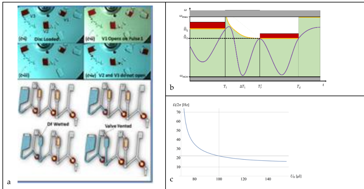
Figure 10. Pulse-actuated CP-DF valving (adopted from [86]). (a) Photo and concept of the fluidic structure. (b) Spin protocol \omega(t) and (c) decrease of the retention frequency \Omega(U_0) with the arrival of the liquid volume U_0(t) . In conventional CP-DF siphon valving (Figure 1), a group of liquids is sequentially released through stepping up the spin rate \omega across their critical burst frequencies \{\Omega_i\} . Digital pulse actuation considers the time \Delta T_i it takes a liquid volume U_0 to advance through the outlet channel between valve opening at the burst frequency \Omega_i , and its arrival at the following valve featuring \Omega_{i+1} . During this interval \Delta T_i , which is primarily determined by the centrifugally induced pressure head p_\omega (2), the flow resistance of the connecting channel on the viscosity of the liquid, and the dissolution time of the DF, the subsequent valve i + 1 is only partially loaded, so its effective retention rate \Omega_{i+1}(T_i < t < T_{i+1}) is transiently be lifted above \Omega_{i+1}(U_0) that is nominally calculated after the arrival of the full volume U_0 (c). The spin rate \omega(t) can thus be spiked well above \Omega_{i+1}(U_0) during this interval \Delta T_i , and also allow \Omega_{i+1} < \Omega_i to squash the requirement of steadily growing retention rates \Omega_{i+1} > \Omega_i for the high-pass valves along the serial assay protocol \omega(t) .
