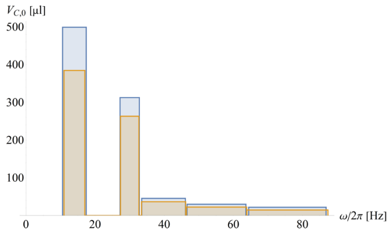
Figure 7 Rotational automation of an exemplary bioassay featuring sequential release of sample and separated plasma as well as pre-stored liquid onboard reagents L1, L2 and L3 with high-pass CP-DF siphon valves of release rates \{\Omega_i\} with \Omega_S/2\pi = 15 Hz and \Omega_P/2\pi = 30 Hz. The release rates \{\Omega_i\} are tuned by the dead volumes of the main compression chamber \{V_{C,0,i}\} , as displayed on the vertical axis. (a) Radial positions (blue) R_i = \{3, 4, 3.5, 3, 2.5\} cm and (orange) R'_i = R_i + 0.5 cm mimic concurrent processing of the same bioassay protocols requiring identical \{\Omega_i\} for concurrent valving ( M = 3 ), while increasing their spatial packing density towards microfluidic LSI.
