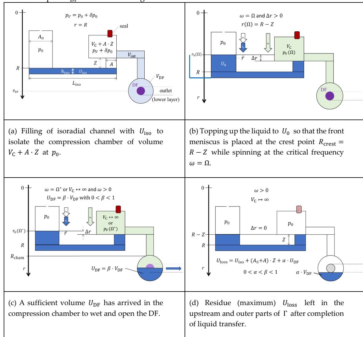
Figure 1. CP-DF siphon valving. The measures of the default geometry \Gamma (linearized display, not to scale) are compiled Table A1. The structure consists of an inlet reservoir of cross section A_0 = d_0 \cdot w_0 with depth w_0 and width w_0 which is connection through a (narrow) isoradial channel of volume U_{\text{iso}} = d_{\text{iso}} \cdot L_{\text{iso}} \cdot h_{\text{iso}} positioned at R to an inbound section of radial extension Z and cross section A = d \cdot w of depth d and width w . (For the sake of simplicity, d_0 = d_{\text{iso}} = d = 1 \text{ mm} is chosen in this rudimentary layout.) During retention, the outer part represents is gas-filled compression chamber, with a main compartment of volume V_{C,0} , isoradial and radial sections of aggregate volume V_{\text{int}} (with V_{\text{int}} \ll V_{C,0} ) connecting to a shallow round chamber of volume V_{\text{DF}}
