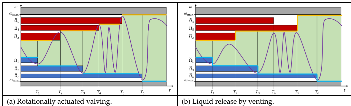
Figure 3. Multiplexing of concurrently loaded valves in frequency vs time domain. High- and low-pass valving takes place at points in time \{T_i\} . With each step i , a certain frequency corridor (green) that is available for LUOs rearranges. (a) For rotational actuation, reliable opening of valves \{i, j\} in a given step i is triggered by fully crossing their linked frequency bands \{\Omega_{i,j} \pm M \cdot \Delta\Omega_{i,j}\} . (b) In venting mode, the concurrently loaded valves serially release according to the order of opening their compression chamber, i.e., V_{C,0,i} \mapsto \infty and p_V \mapsto p_0 .
