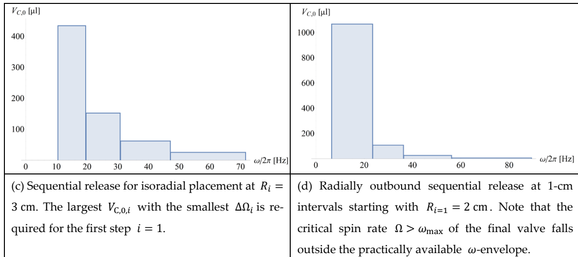
Figure 5. Distribution of bands in frequency space \omega with required volumes of the main compression chamber V_{C,0,i} for the different radial staggering and release scenarios portrayed in Figure 4. CP-DF siphon valves \{i,j\} to be released simultaneously, i.e., T_i = T_{i+1} , or sequentially, i.e., T_i < T_{i+1} ; the valves, which have similar geometries \Gamma_{i,j} of their liquid-occupied sectors and downstream compression volumes V_{C,0,i,j} , are placed isoradially, i.e., at R = 3 cm, or staggered over radial positions R = \{2,3,4,5\} cm. The reliability factor is M = 4 . (a) A set of radially staggered valves \{i,j\} with R_{i,j} > R_{i,j-1} has been tuned through their V_{C,0,i,j} to simultaneously burst in the same step i once \omega > \Omega_i + M \cdot \Delta\Omega_i with \Delta\Omega_i = \max\{\Delta\Omega_{i,j}\} . There are three representative cases for sequential actuation with \Omega_i - M \cdot \Delta\Omega_i > \Omega_{i-1} + M \cdot \Delta\Omega_{i-1} for successive steps i according to \Omega_i > \Omega_{i-1} . (b) For identical \Gamma_{i,j} and V_{C,0,i,j} , the valves will open according to their radially inbound order R_i < R_{i-1} . (c) For isoradial alignment R_i = R = \text{const.} , the valve with the largest V_C opens first: V_{C,i} < V_{C,i-1} . (d) Also, a radially outbound opening sequence R_i > R_{i-1} can be achieved, for which V_{C,i} needs to be drastically reduced along successive steps i to suppress premature release from by the high pressure p_\omega (2) at distal locations R , which comes at the expense of huge bandwidth \Delta\Omega (20).
