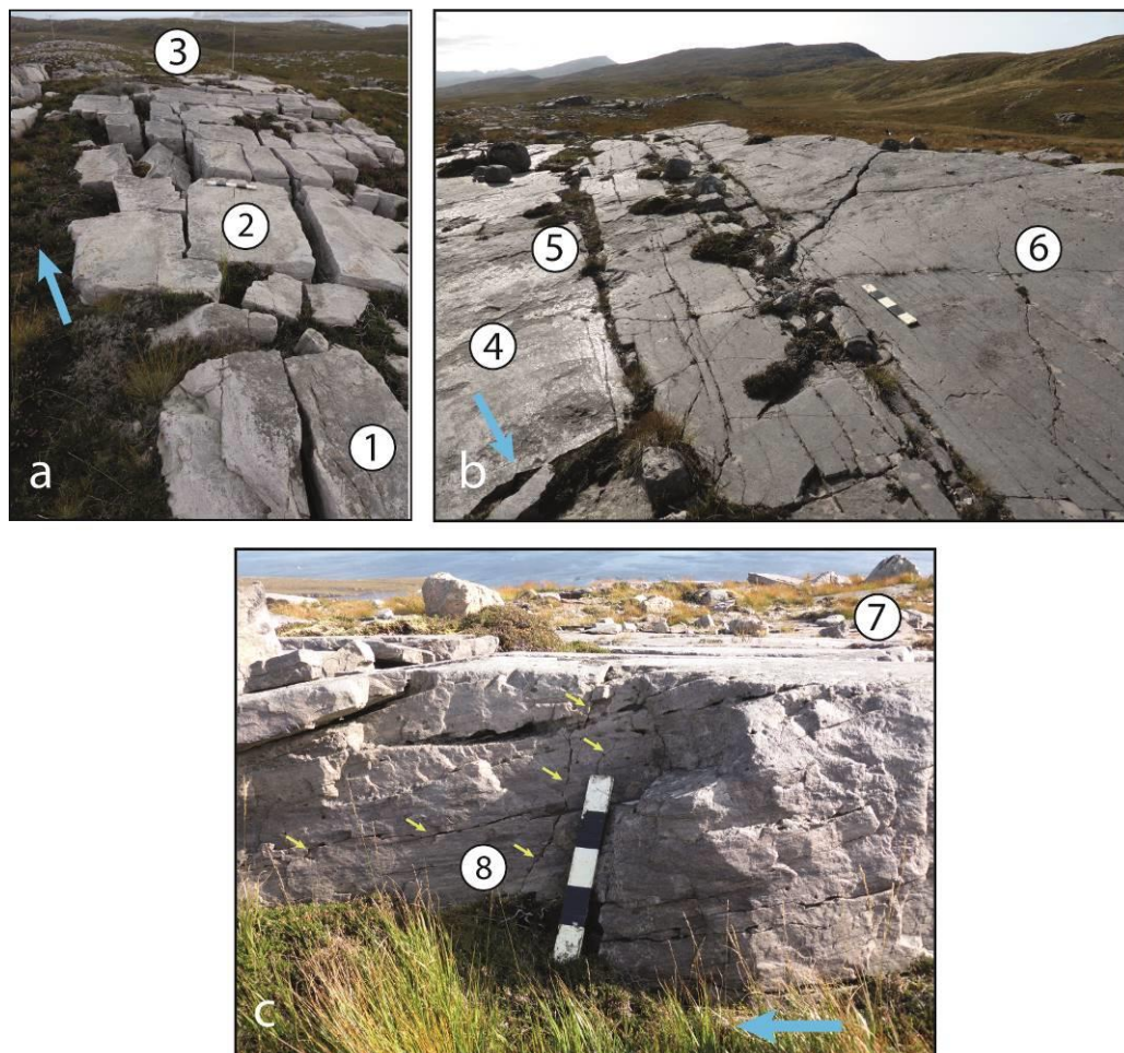
Figure 5. Fracture dilation and formation. View down-dip across a disrupted ~100 m long roche moutonnée (D4) at NC 4380 6327. The scale bar (circled) is 0.5 m long. (1) abraded top surface, (2) stoss side block loss (D6), (3) dilated joints (J1), (4) dilated bedding planes and joints (J1), (5) sites of block loss from flank and lee of hill (D2 and D6), (6) tail of rubble till (T6). For criterion codes, see Table 1.
