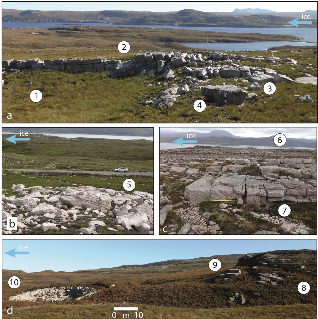
Figure 10. Glacial transport: tearaways, boulder spreads and lee side plucking. (a) Ripped rock surface at NC 441 637 with (1) basal décollement surface parallel to bedding (D3), (2) lateral cliff (D2) left after tearaway of rock sheet, with block collapse, (3) dilation of vertical fractures (J1) and (4) transported boulder, with 0.5 m scale bar. (b) Quartz-arenite boulder spread (T1) at NC 443 638.
