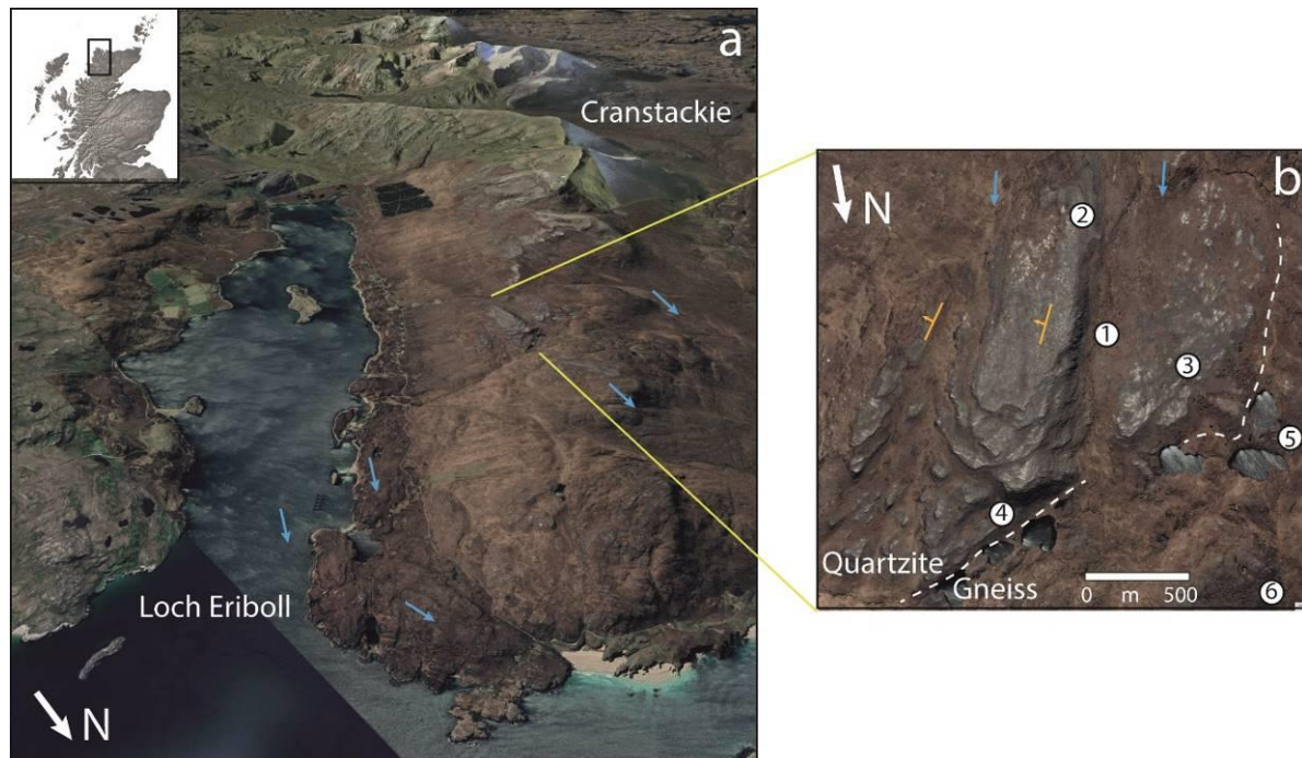
Figure 1. Topography and landforms around Loch Eriboll, NW Highlands. Images © CNS/Airbus, Google, Maxar Technologies a. Location and topography. Blue arrows indicate directions of ice flow. b. Structural landforms at Hill 314 (Figure 2). 1. strike-parallel valley, deepened by glacial erosion. 2. flank cliff facing up dip, with rounded edge. 3. Backslope, with glacially abraded surface. 4. Stepped face after lee-side glacial plucking. 5. Shallow rock basin developed after excavation of weathered gneiss on the sub-Cambrian unconformity. 6. Low gneiss dome. Dashed white line indicates the line of unconformity between the Lewisian gneiss and the overlying Basal Quartzite.
