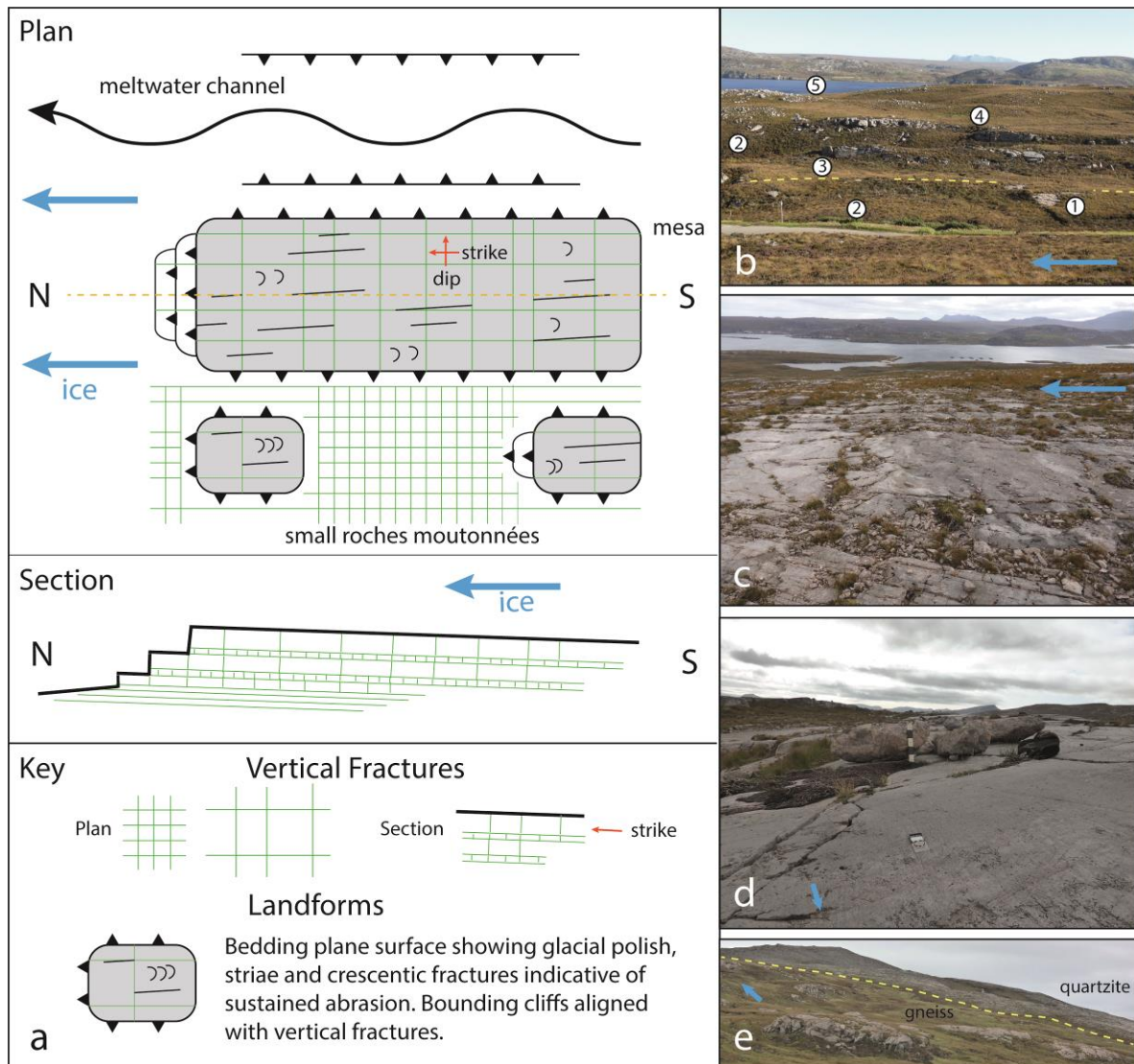
Figure 4. Plan and section model of the main structural and precursor glacial landforms developed in Cambrian quartz-arenite at Loch Eriboll. (a) Model of glacial erosion forms in relation to quartz-arenite structure and ice flow direction. (b) View looking SE from NC 438633 and down dip across structurally controlled homoclinal ridges with typical glacial erosion forms. (1) Gneiss unconformity surface at the base of the quartz-arenite. Plane of unconformity indicated by dashed line. (2) Meltwater channels. (3) Small cliff on plucked lee side of ridge. (4) Lateral cliff in thick quartz-arenite bed on edge of homoclinal ridge. (5) Roche moutonnée. (c) View down dip across an extensive quartz-arenite pavement on Hill 314. (d) Detail of bedding plane surface at NC 431638 viewed along strike showing striated surface and gneiss erratic boulders. Scale bar is 0.5 m long. (e) Different terrains on Precambrian gneiss and Cambrian quartz-arenite, with the line of unconformity shown. Boulder spreads are confined to the quartz-arenite. View N from Hill 314.
