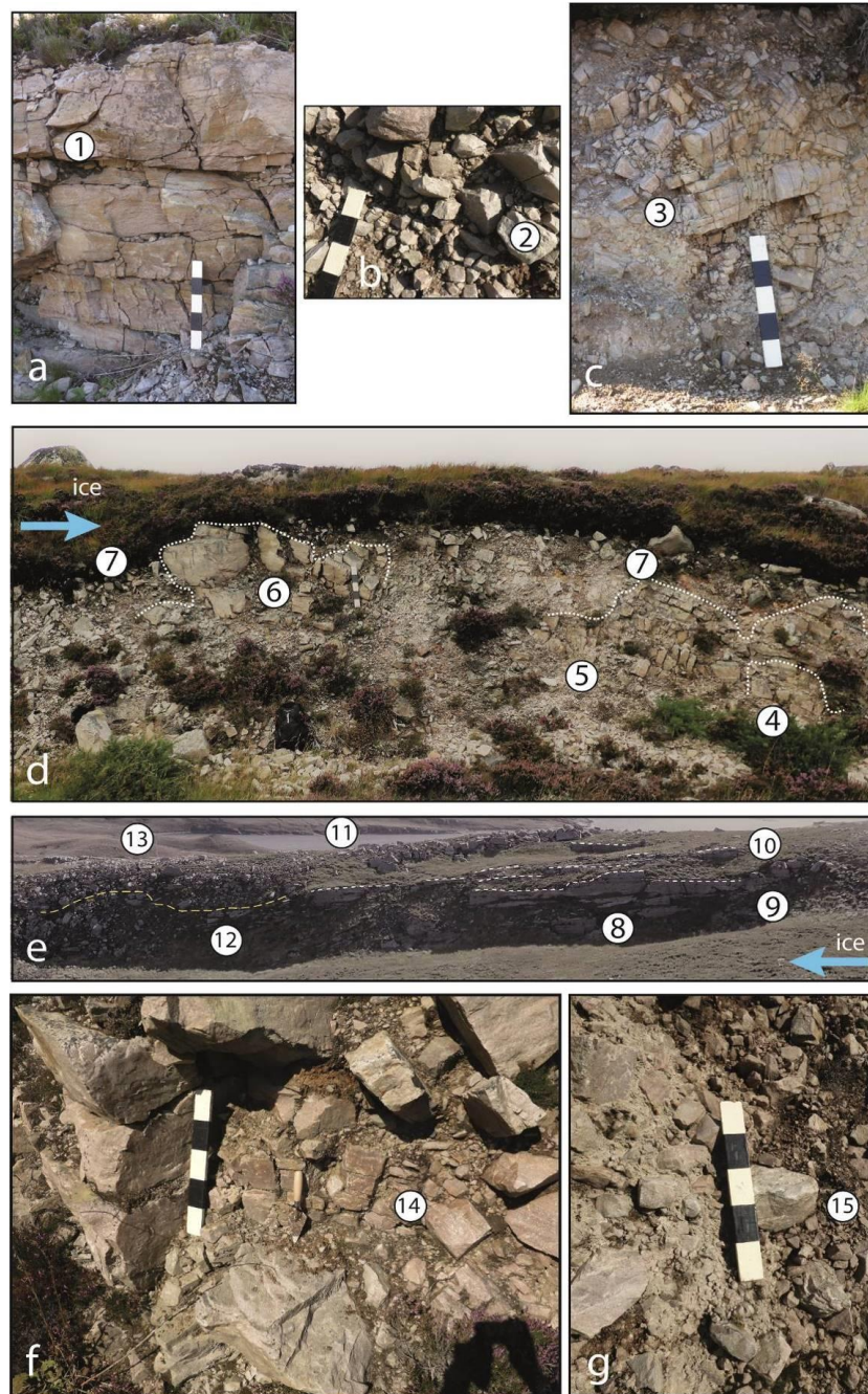
Figure 11. Transitions from breccia to rubble till. (a) Crackle breccia (J2) with sediment fill along horizontal fracture (1) at NC 425608. (b) Mosaic breccia (J2) without sediment infill at NC 395560. Rock mass structure still visible from fitting clasts (2). (c) Rubble breccia with displaced and rotated blocks (3) at NC 442625. (d) Roadside section at NC 443638 showing transitions between in situ rock (4), crackle and mosaic breccia (5), rubble breccia (6) and rubble till (7). The upper part of the rubble till (T6) has sparse gneiss erratics. (e) Relationships between rock, breccia and rubble till. View of a cliff face along strike on the side of a small meltwater channel at NC 442639. The quartz-arenite remains undisrupted at shallow (c. 2.5 m) depth in places (8) but disruption to mosaic and rubble breccias occurs nearby (9). Numerous décollement surfaces are seen (D3: dashed white lines) (10) where sheets of quartz-arenite have been removed. Thick quartz-arenite beds are disrupted, with formation of shallow boulder rubble breccia and surficial boulder spreads (11). Rubble till thickens on lee slopes, but the boundary between breccia and overlying rubble till is indistinct (dashed yellow line) (12). The ground surface carries a spread (T1) of small boulders (13). (f) Rubble till of angular boulders and cobbles with sandy matrix between clasts set within rubble breccia (14) at NC 4184 5983. (g) Monomict quartz-arenite rubble till with sandy matrix at NC 409581. Edge rounding on clasts after local transport (15).
