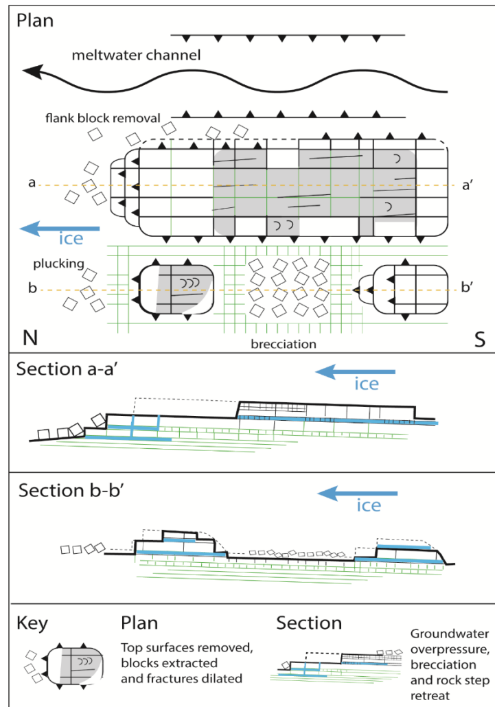
Figure 13. Model of the impacts of groundwater overpressure and glacial ripping on pre-existing glacial bedforms and surfaces in quartz-arenite at Loch Eriboll. Criteria from Table 1. Compare to Figure 4.
