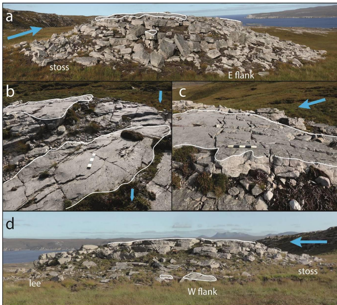
Figure 9. Disruption of a small roche moutonnée at NC 4312 6388. (a) Disintegration of quartz-arenite surfaces to 0.6 m depth on stoss and flank faces (D4). The scale bar is 50 cm long. (b) Intact polished and abraded upper surface (outlined in white) with intervening areas of slab loss (D6) with higher micro-roughness. (c) Abraded upper surface showing cracks (J4) developed after hydraulic jacking along the underlying bedding plane. (d) Northern flank of hill showing extensive block loss along the flank (D4) but limited plucking of the lee face.
