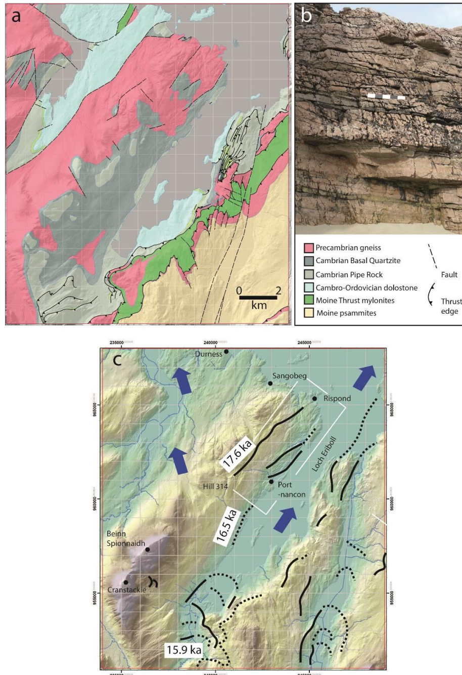
Figure 2. Geology and rock structure. (a) Geology and relief based on BGS maps. (b) Cambrian Basal Quartzite at Sangobeg (Figure 1c). The scale bar is 0.5 m long. (c) Topography, ice flow and dated ice limits.
