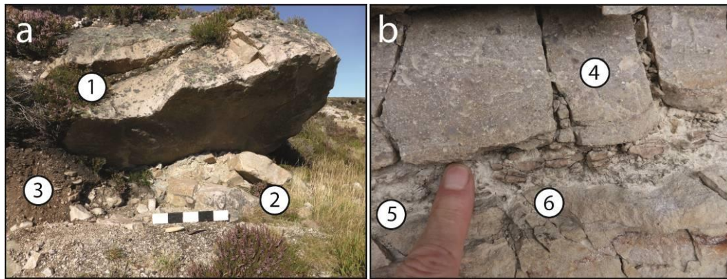
Figure 7. Open fractures and clastic sills (a) Dilated fractures (J1) in a disrupted thick bed of quartz-arenite at NC 4184 5993. (1) Fracture fill (J5) of quartz-arenite gravel, including both angular and sub-rounded pebbles. (2) Fracture filled by rubble breccia and sand matrix. (3) talus. (b) Dilated bed of silty sandstone and fracture fill at NC 4398 6213. (4) Crackle breccia (J2) with fragmentation along block edges. (5) Fill of laminated medium-grained sand. (6) Brecciated silty sandstone, with detachment and rotation of rock fragments and admixture with sand.
