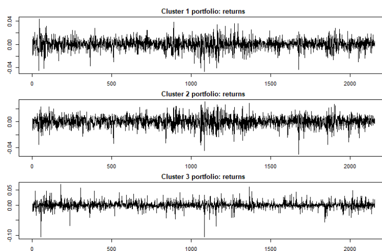
Figure 7. Returns of the C = 3 clustered portfolios (with M = 360 )
