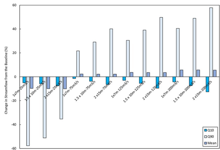
Figure A2 The change in the Q10, Q90 and mean simulated streamflow from the baseline with the inclusion of check dams of various density and dimensions (Table A1).
