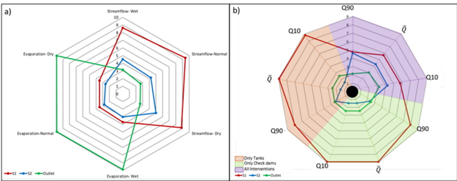
Figure 9. a) The percent reduction in total annual simulated streamflow and increase in total annual simulated evaporation (%) with the inclusion of interventions for S1, S2 and the basin outlet in wet (2005), normal (1998) and dry (2002) years. b) The effect of all the interventions (tanks, check dams and bunds), check dams only and tanks only on high flows (Q10), low flows (Q90) and mean flows ( \bar{Q} ) flows across S1, S2 and the basin outlet (Table 1, Figure 1).
