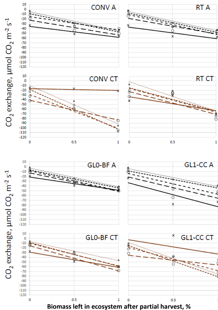
Figure 7. The Gross Ecosystem Production (GEP) in response to 0, 50 or 100 % of the aboveground plant biomass left in the three columns of similar origin in each climate treatment. Mons (top) and Auzéville-Tolosane (bottom). Each trend line represent a measuring day that correspond to an increase in temperature. The lines indicate timing of measurements: the smaller dots or dashes the earlier the measurements, and the more solid the later the measurements. For further information about the treatment abbreviations, see Table 1 and Figure 2.
