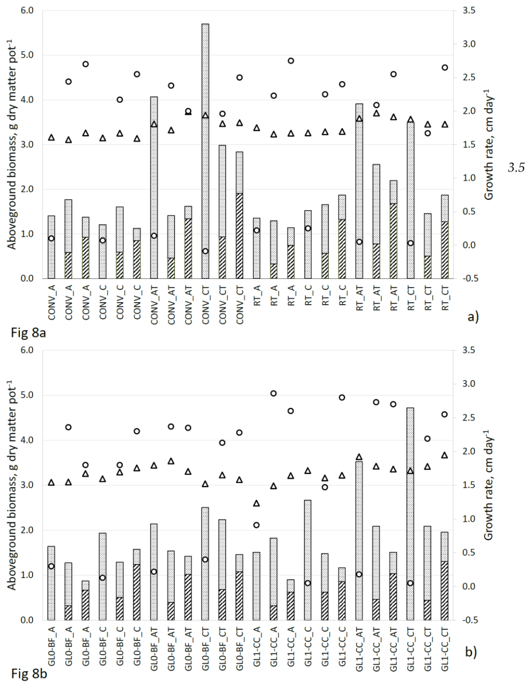
Figure 8. The biomass from the individual soil columns Mons (top) and Auzesville-Tolosane (bottom). The bars reflect if the biomass has been harvested or not. The obliquely hatched is the first round of harvest and the dotted bars indicate the final harvest. Red triangles indicates the barley growth rate in cm day -1 at the time from sowing to partial harvest, and the blue circles indicate the growth rate from partial harvest to final harvest
