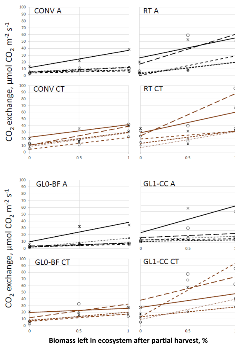
Figure 6. The Ecosystem Respiration (ER) in response to 0, 50 or 100 % of the aboveground plant biomass left in the three columns of similar origin in each climate treatment. Mons (top) and Auzville-Tolosane (bottom). Each trend line represent a measuring day that correspond to an increase in temperature. The lines indicate timing of measurements: the smaller dots or dashes the earlier the measurements, and the more solid the later the measurements. For further information about the treatment abbreviations, see Table 1 and Figure 2.
