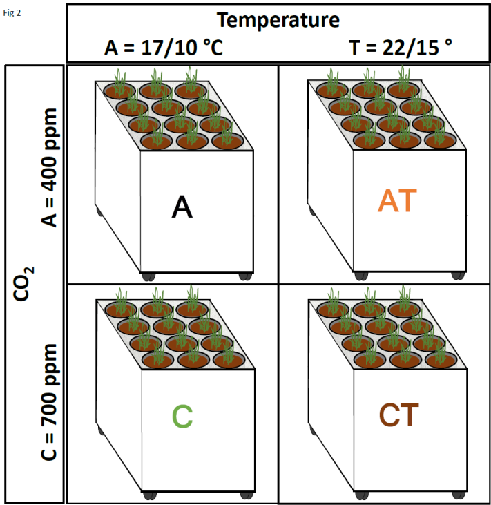
Figure 2. The climate treatments' compositions of temperature and CO 2 -concentration with the low (A and C) and high (AT and CT) temperatures resembling the common values at the geographical origin of the soils influenced by ambient (A) and increased (C) atmospheric CO 2 -concentrations, respectively.
