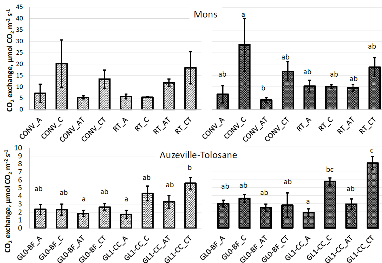
Figure 5. Respiration measured on the Mons (top) and the Auzeville-Tolosane (bottom) soils, without plants: light color (left) before sowing and dark color (right) after sowing. Letters indicate cases of no significant difference. For further information about x-axis treatment abbreviations see Table 1 and Figure 2.
