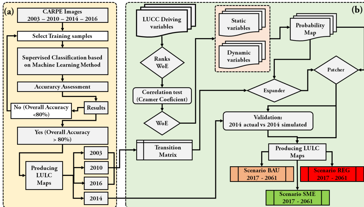
Figure 2. Workflow of the study: (a) Land use and land cover (LULC) classification; (b) Modeling of deforestation. Abbreviations: CARPE, The Central Africa Regional Program for the Environment; WoE, Weights of Evidence; LUCC, Land use and cover changes; LULC, Land use and land cover.
