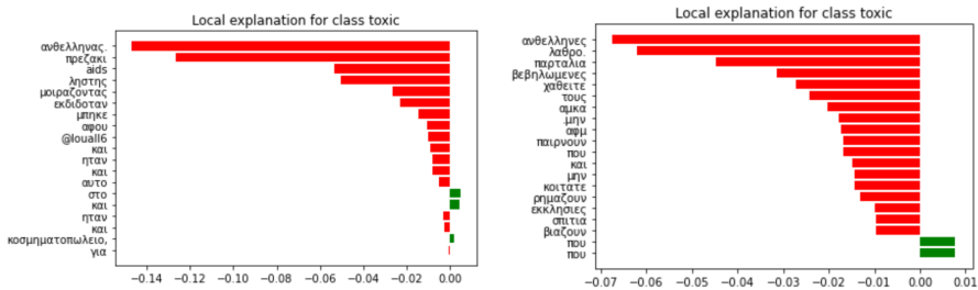
Figure 3. Words contributing to toxic prediction
