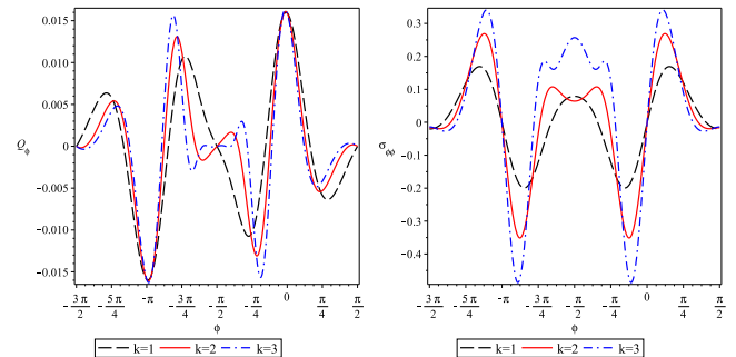
FIG. 7: Shear force for different radius a = 3k[m] . Left: Shear force Q_\phi ; Right: Stress \sigma_1 .
