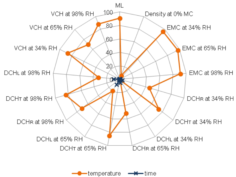
Figure 2. The percentual influence of temperature and modification time on the mass loss (ML), density ( \rho ), equilibrium moisture content (EMC) and dimensional changes (DCH) of black poplar thermally modified in nitrogen atmosphere.
