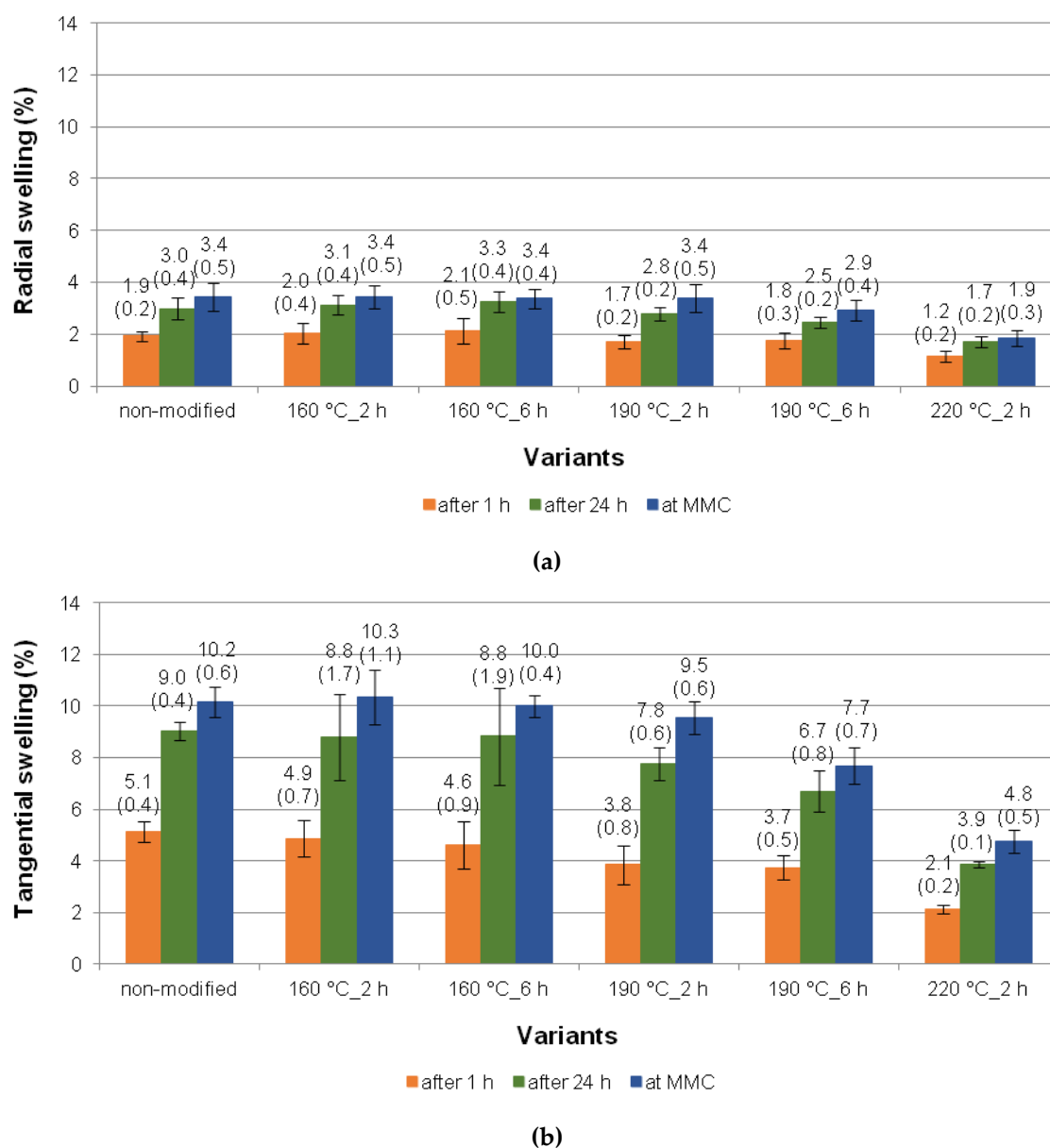
Figure 5. Swelling in the radial (a) and tangential (b) directions of black poplar thermally modified in nitrogen atmosphere (error bars - standard deviation ( \pm SD)).
