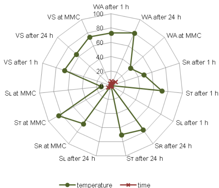
Figure 7. The percentual influence of temperature and modification time on the water absorption (WA), linear swelling (S) and volumetric swelling (VS) of black poplar thermally modified in nitrogen atmosphere.
