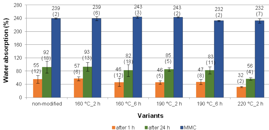
Figure 4. Water absorption (WA) of black poplar thermally modified in nitrogen atmosphere (error bars - standard deviation ( \pm SD)).
