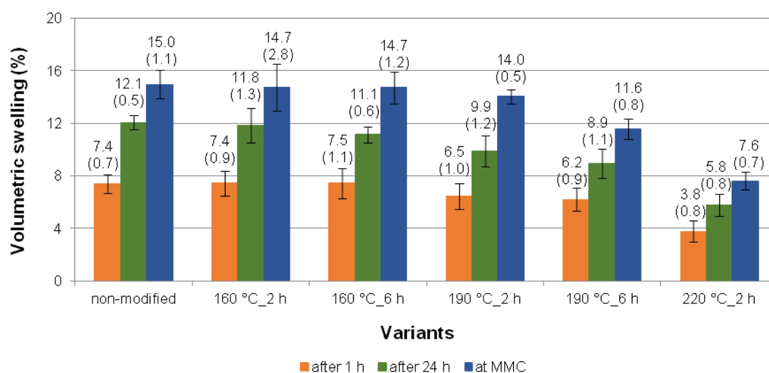
Figure 6. Volumetric swelling (VS) of black poplar thermally modified in nitrogen atmosphere (error bars - standard deviation ( \pm SD)).
