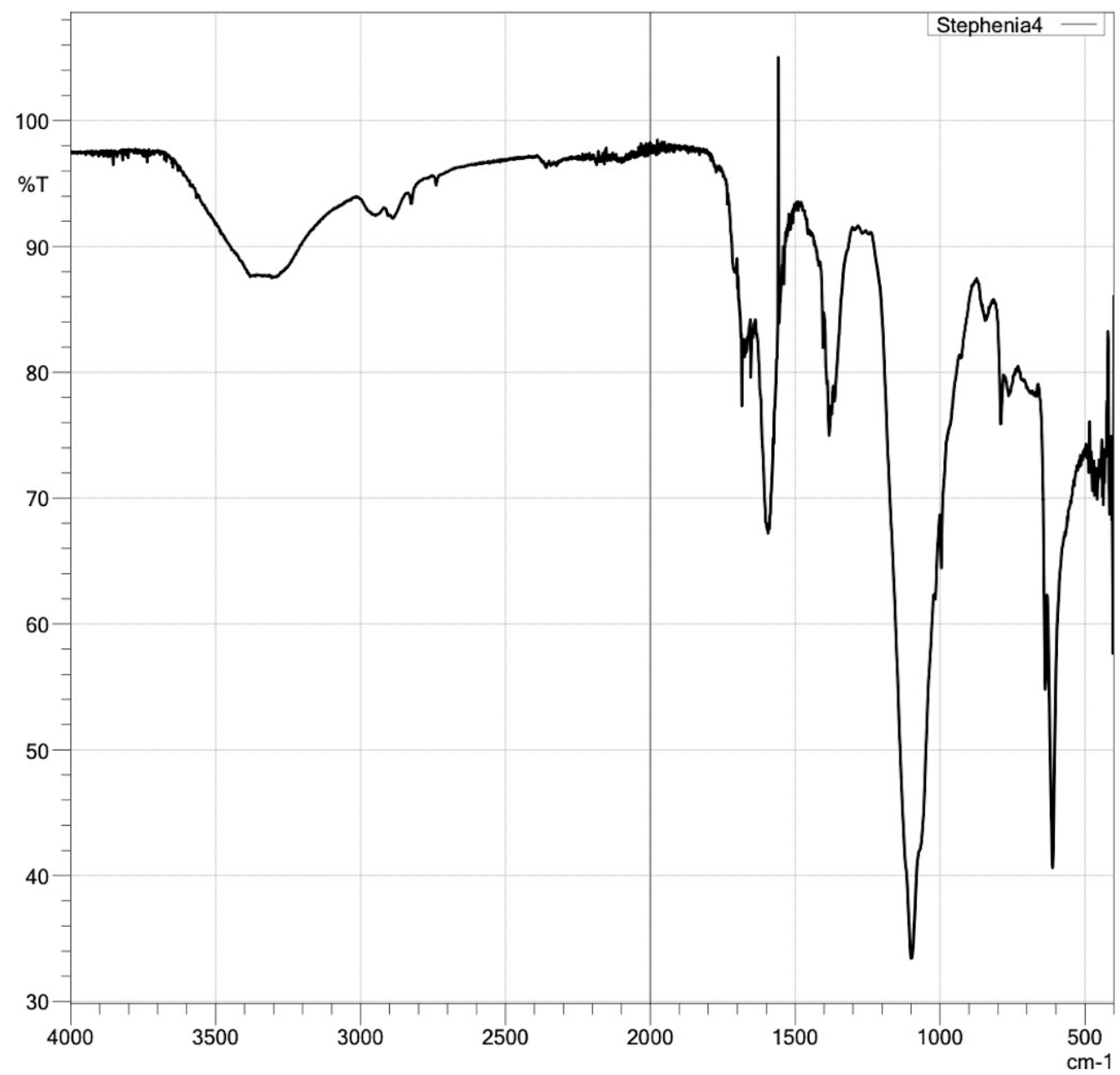
Figure S1. FT-IR chromatogram of oroxyquinone
