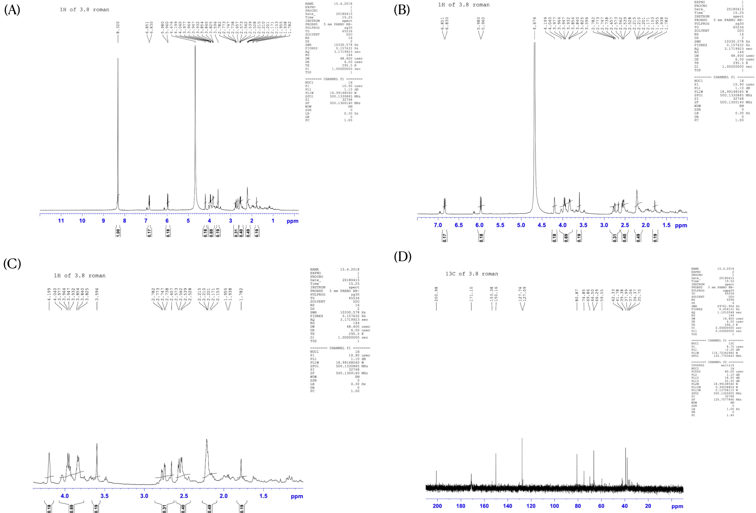
Figure S3. NMR chromatograms of oroxyquinone: A-C; 1 H, D; 13 C
