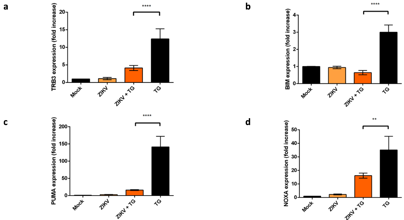
Figure 5. Transcriptional activity of CHOP-dependent genes
