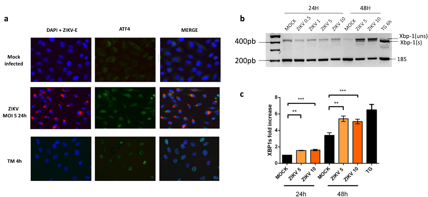
Figure 2. UPR inducible Transcription Factors, ATF4 and Xbp-1(s) are up-regulated in A549 cells infected with ZIKV
