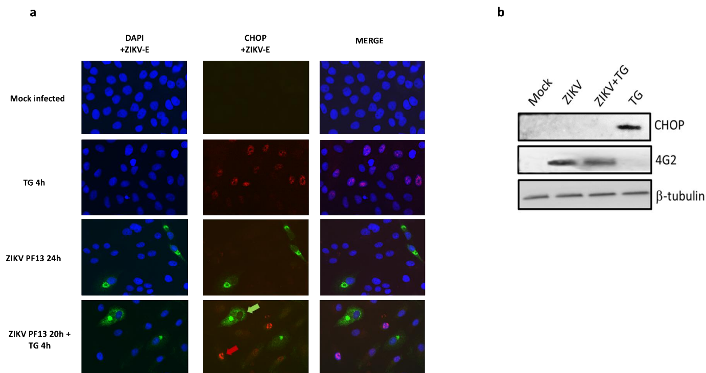
Figure 4. ZIKV inhibits CHOP protein expression in the infected cells.
