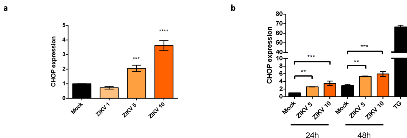
Figure 3. CHOP expression is upregulated at the transcriptional level in ZIKV infected cells.
