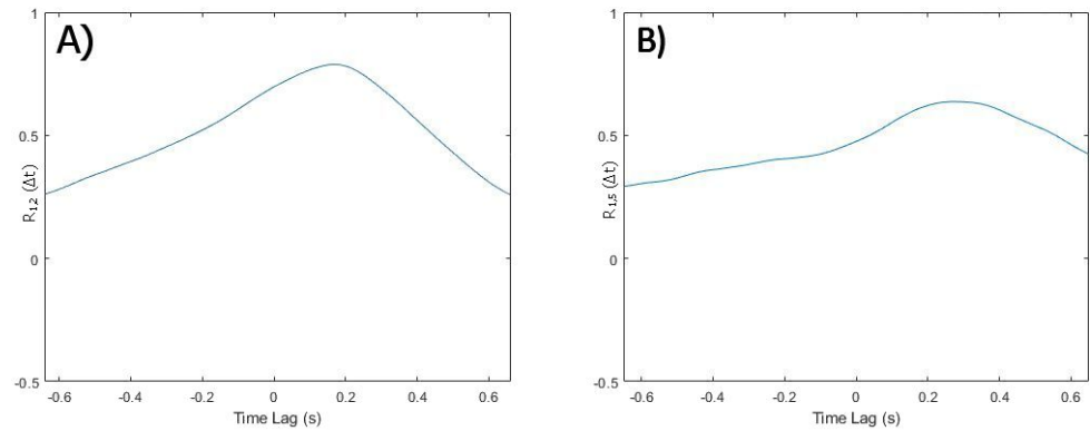
Figure 6. Typical profiles of the cross-correlation function around the peak for tunnel flow speed at 20cm/s A) CC of whiskers w1 & w2, peak value of 0.78 B) CC of whiskers w1 & w5, peak value of 0.62. The greater time delay in B) is due to the lower velocity, as discussed above.
