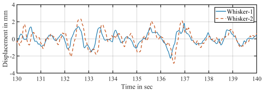
Figure 5. Fluctuating tip-motion of a pair of two whiskers in the same horizontal plane, showing similar characteristic jerk motion, off-set from each other by the convection time taken for vortices to travel the distance between both (mean component subtracted)
