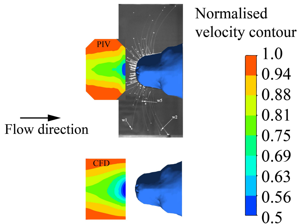
Figure 4. Bow-wake region in front of the snout from experimental flow field measurement compared to the CFD flow field (displayed as color-coded contours of constant streamwise velocity).
