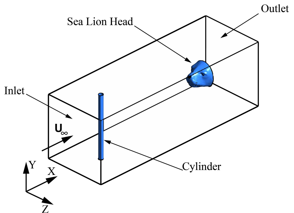
Figure 2. Sketch of the CFD domain and the flow configuration similar to the experiment. The domain extends 0.4m in Y and Z directions and 1.2m in X direction.
