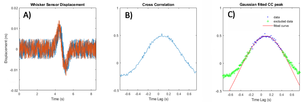
Figure 7. Synthetic jerk-pulse with added random noise and its CC profile. A) jerk signal with an SNR of 2.6 in original (red) and time-shifted with 0.1s (blue), noise addition is random and independent in both signals. B) CC of the noisy signals, showing erratic fluctuations near the peak. C) Gaussian curve fit in the peak region with a clear maximum at the expected time-lag.
