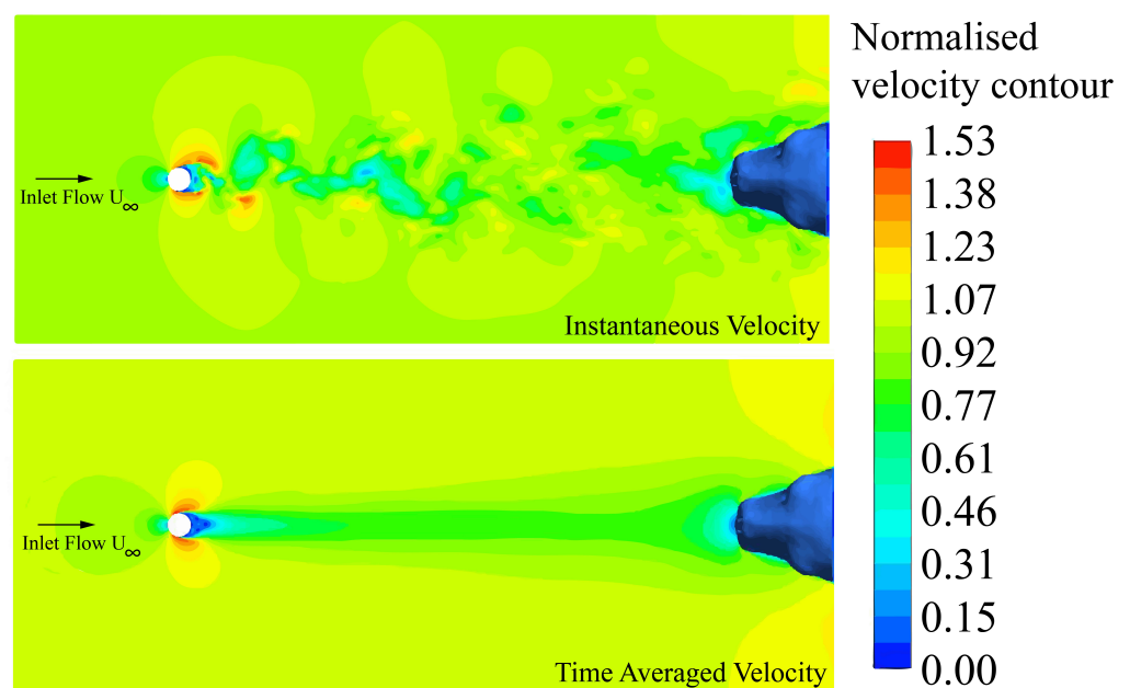
Figure 3. Velocity field through the test section from CFD Simulation (displayed as color-coded contours of constant streamwise velocity). Top: Instantaneous velocity field, Bottom: Time-averaged flow pattern.
