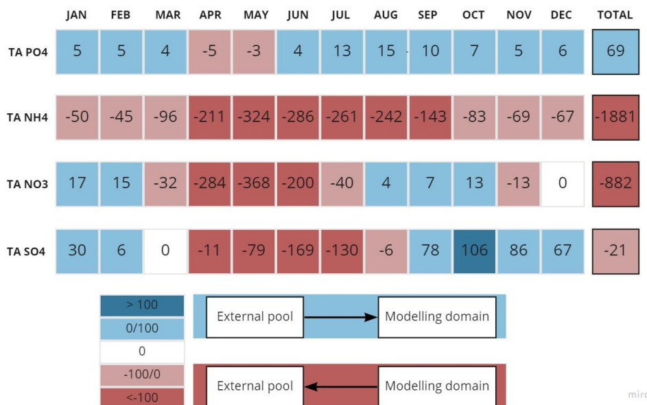
Figure R1. Scenario 1. The fluxes of TA components integrated through the water column (between the modeling domain and the external pool), in \text{mM m}^{-2} per month and year for the 'Total' column. Positive values represent alkalinity flux from the external pool to the modeling domain, negative - alkalinity outflows from the modeling domain to the external pool.
