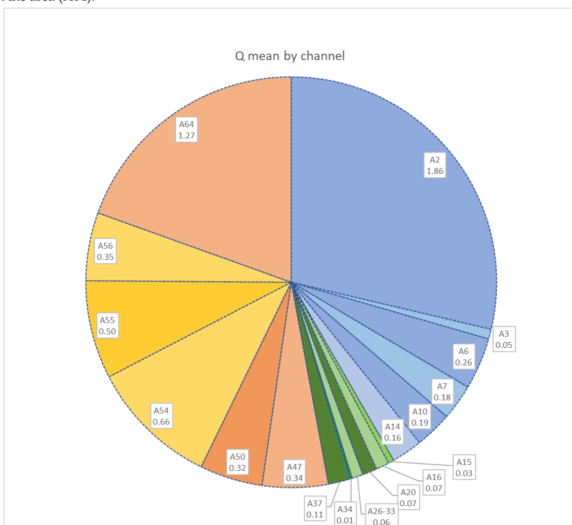
Figure 5. Average flow for each canal, grouped by the origin of the water inflow to the lagoon: in blue are the inflows from the River Turia; in green those coming from the RCJ and in yellow-orange those coming directly from the River Júcar.
