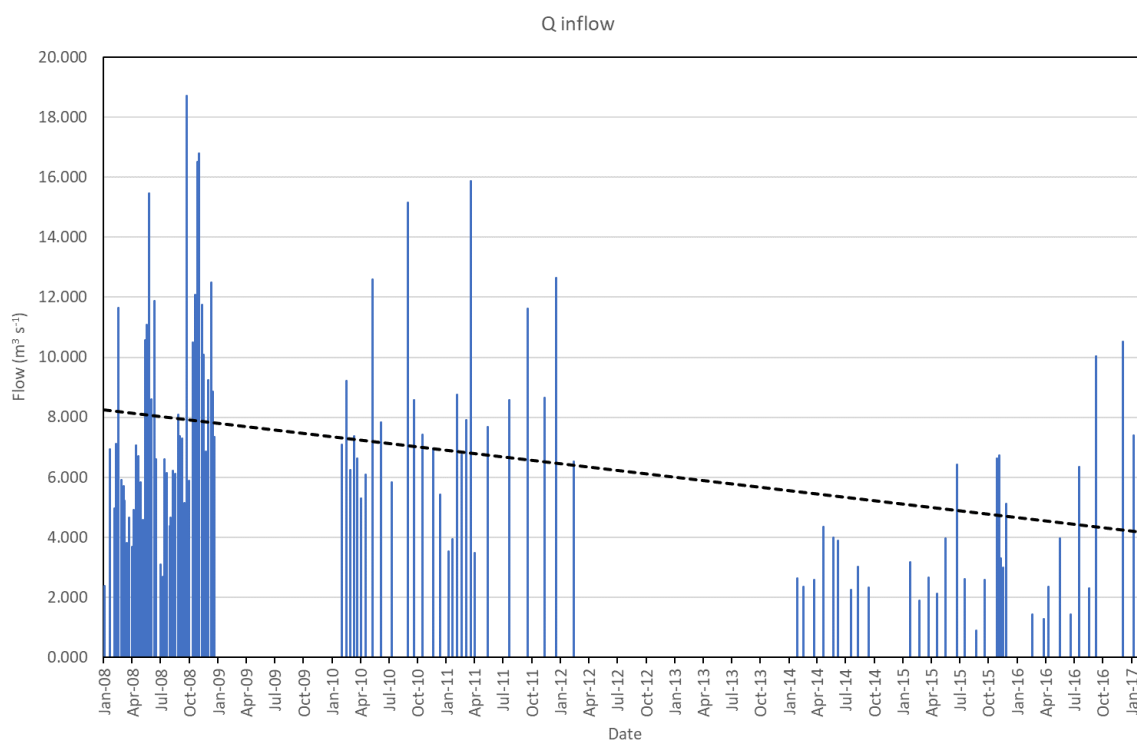
Figure 2. Inflow to the Albufera in each of the sampling dates. The dotted line indicates the downward trend.
