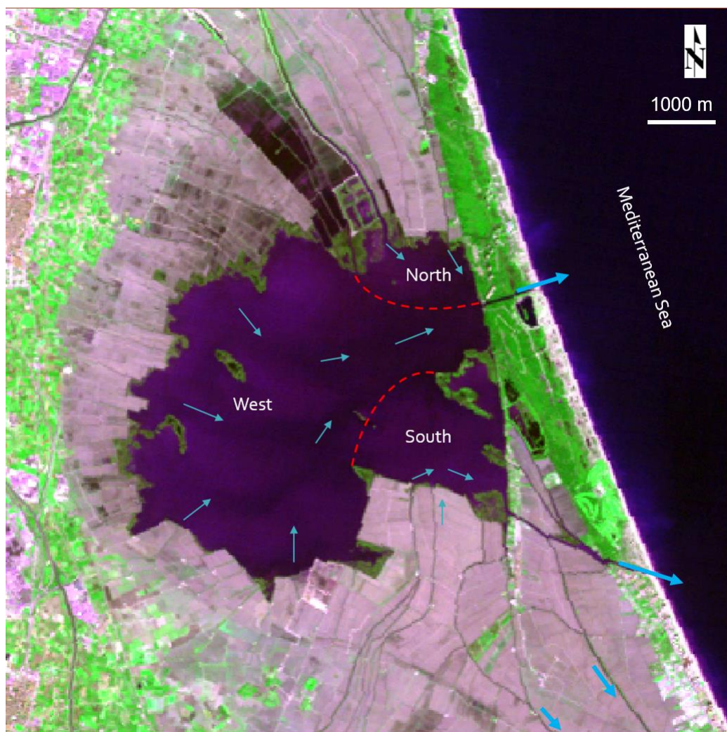
Figure 7. Distribution in zones and water circulation in the Albufera elaborated from the bathymetry of the lagoon and the observations in the lagoon itself. Landsat-5 base image in false natural color from March 14, 2010: Dark areas indicate greater depth (over 1.2 m) and light areas less depth (over 0.6 m).
