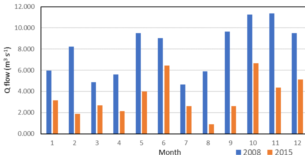
Figure 3. Average inflow in each month, estimated in two different years: in blue year 2008 which presented high values; in orange year 2015 with low values.
