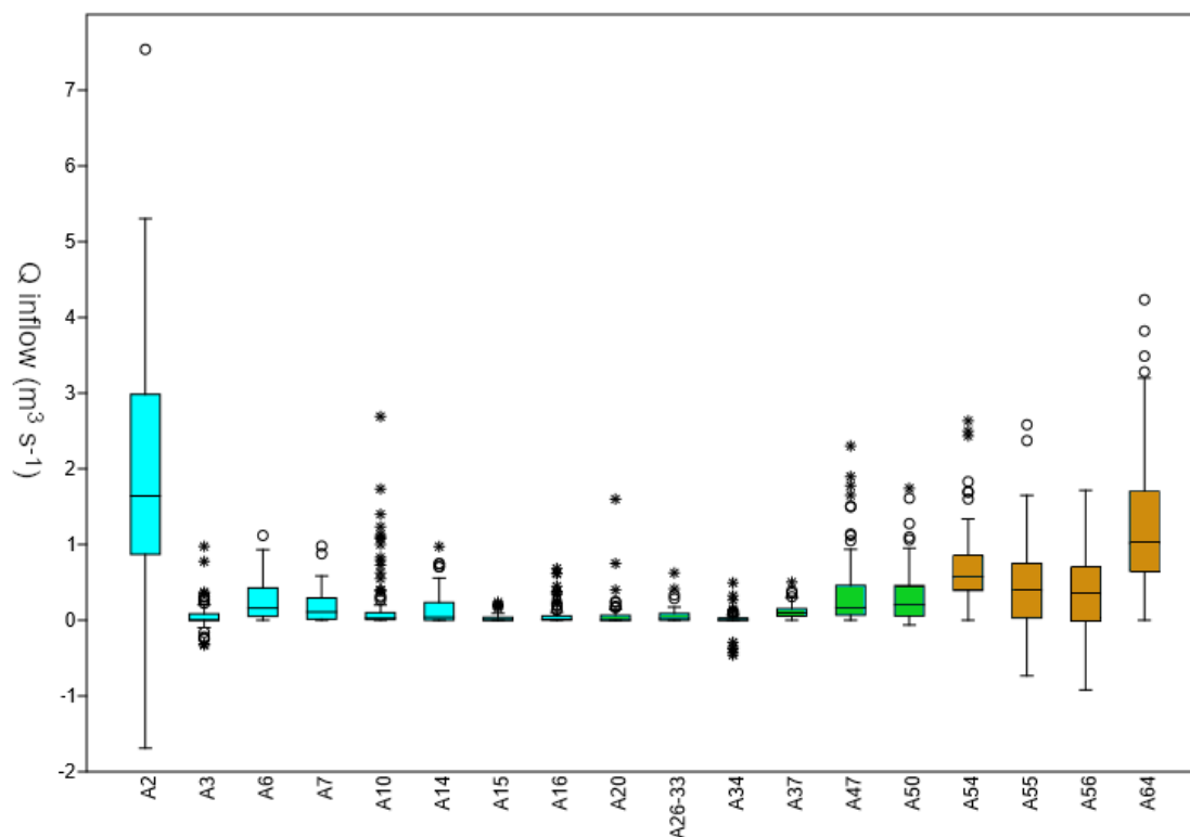
Figure 4. Average inlet flow for each of the most important ditches that inflow to the Albufera. Those identified with A2, A3, A34, A55 and A56 sometimes have reverse flow and instead of water entering
