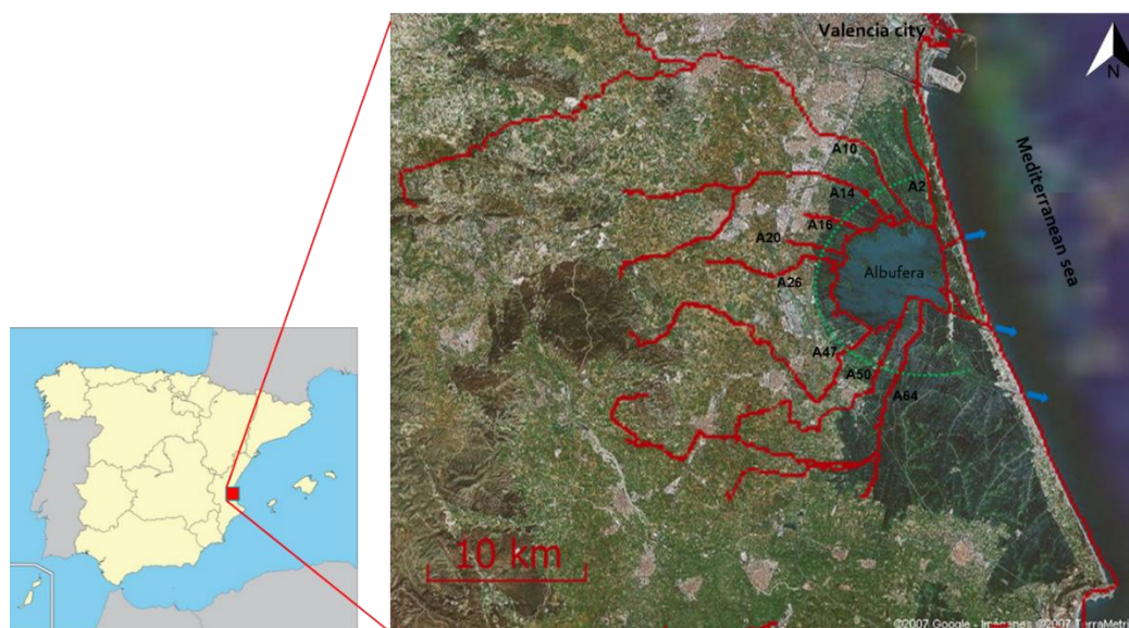
Figure 1. Situation of the Albufera of Valencia in the Iberian Peninsula. It is indicated with red lines the natural courses affluent to the lagoon and the code used in the study. The unmarked canals correspond to irrigation ditches in the rice fields. The blue arrows indicate the location of the three communication canals between the lagoon and the Mediterranean Sea. The discontinuous green line indicates the area of polders. Base image of Google Earth 2007.
