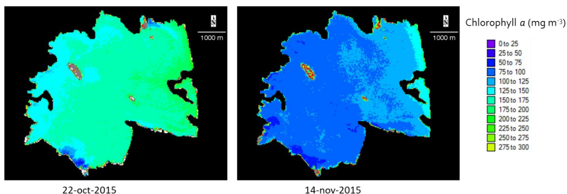
Figure 9. Measurement of chlorophyll a during autumn 2015 using Landsat-8 satellite images in the Albufera of Valencia on a previous date (October) and during the process of renewal by water supply from the west area (November).
