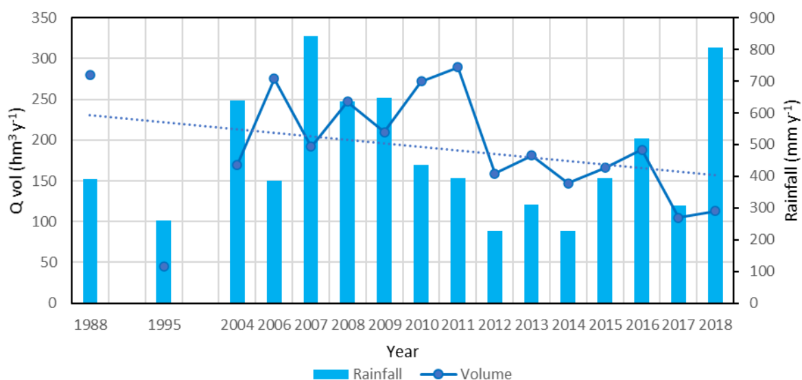
Figure 6. Annual contributions to the Albufera de Valencia showing the trend line and accumulated annual rainfall.
