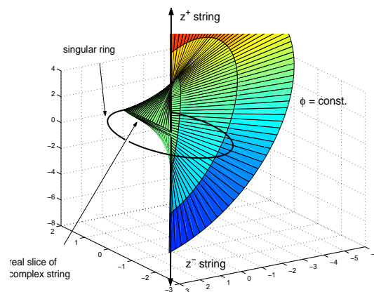
Figure 3: Deformations of the Kerr coordinate \phi = const. caused by dragging of space in angular direction near the Kerr singular ring.
