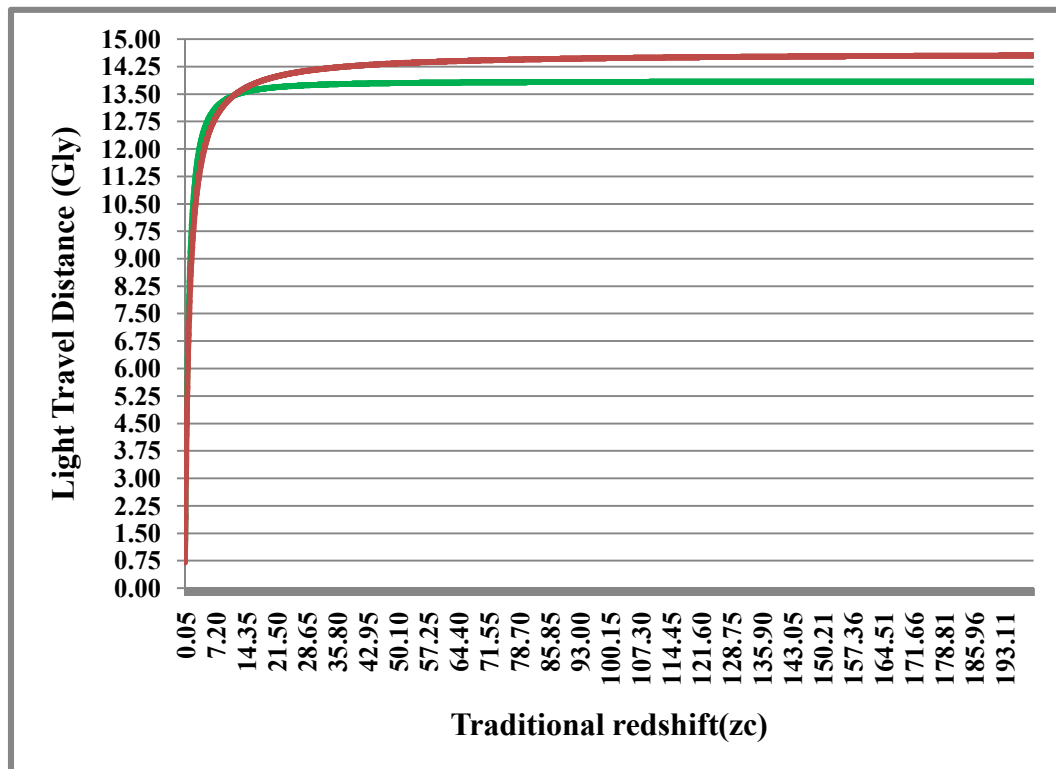
Figure 2: Comparison of standard and estimated light travel distance
