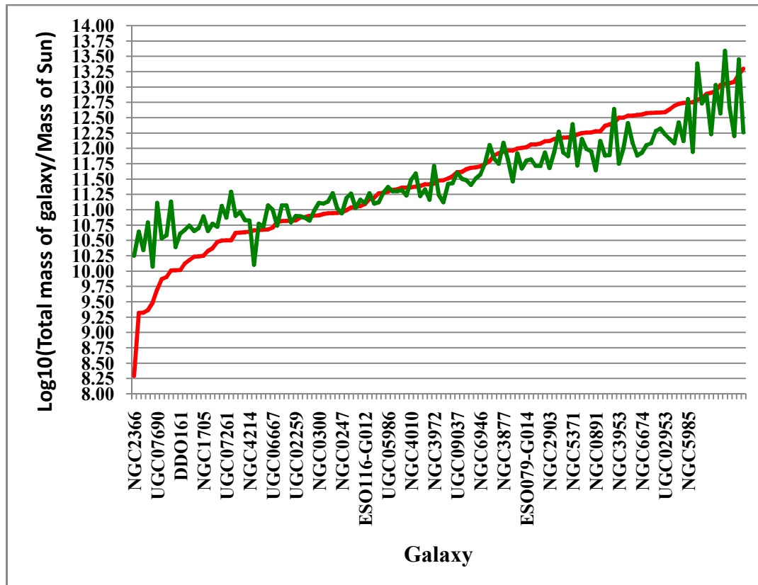
Figure 1: To compare estimated total mass of galaxy with NFW model
