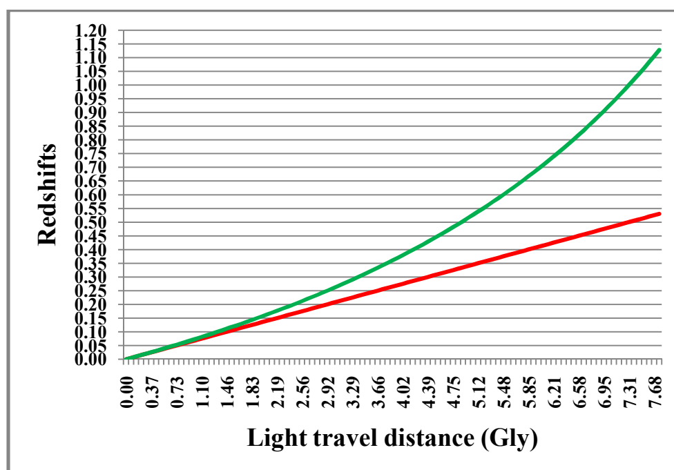
Figure 3: Comparison of standard and re-defined redshifts
