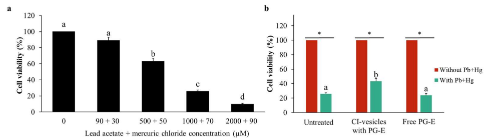
Figure 6. – Viability (determined by the MTT assay) of HaCaT cells incubated for 24 h with different combinations of lead acetate and mercuric chloride ( \mu\text{M} ) (a) and treated for 24 h with cauliflower inflorescence vesicles (CI-vesicles) with pomegranate extract (PG-E) or free PG-E previous to the application of heavy metals (1000 \mu\text{M} lead acetate + 70 \mu\text{M} mercuric chloride) (b). The results were normalized as a function of the control cytotoxicity. Data are means \pm SE (n = 6). Different letters indicate significant differences between groups and *, significant differences compared to the respective control ( p < 0.05 ).
