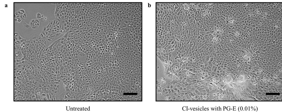
Figure 5. – Phase contrast microscopy images of HaCaT cells: untreated (a) and treated for 24 h after reaching 60-70% confluence with cauliflower inflorescence vesicles (CI-vesicles) containing pomegranate extract (PG-E) at a concentration of 0.01% (b). Scale bars = 100 \mu m.
