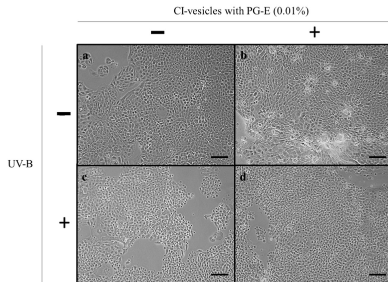
Figure 8. - Phase contrast microscopy images of HaCaT cells without cauliflower inflorescence vesicles (CI-vesicles) and UV-B treatment (a), with CI-vesicles and without UV-B treatment (b), without CI-vesicles and with UV-B treatment (c) and with CI-vesicles and UV-B treatment (d). Scale bars = 100 \mu\text{m} .
