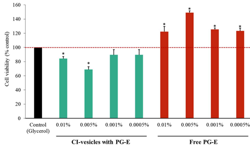
Figure 4. – Viability of HaCaT cells incubated for 24 h with different concentrations of pomegranate extract (PG-E), encapsulated in cauliflower inflorescence vesicles (CI-vesicles) or free, as determined by the MTT assay. The results were normalized as a function of the glycerol cytotoxicity. Data are means \pm SE (n = 6). *p < 0.05, significantly different compared to the control group.
