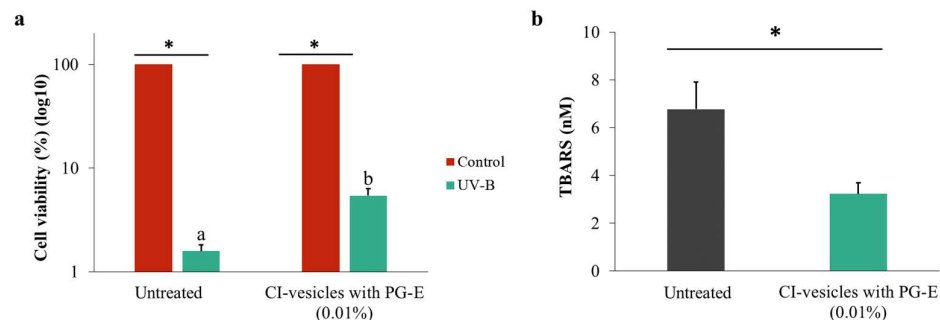
Figure 7. – Viability of HaCaT cells after UV-B exposure, determined by the MTT assay. The results were normalized as a function of the control cytotoxicity (a). TBARS (nM) released into the culture medium by HaCaT cells (b). The HaCaT cells were exposed to UV radiation after treatment for 24 hours with cauliflower inflorescence vesicles (CI-vesicles) with pomegranate extract (PG-E) (0.01%). Data are means \pm SE (n = 6). Different letters indicate significant differences between groups. *, significant differences compared to the respective control (p < 0.05).
