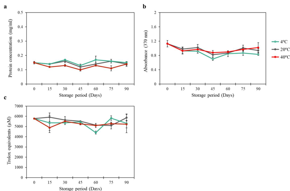
Figure 2. - Protein (mg/ml) stability (a), colour (absorbance at 370 nm) stability (b) and antioxidant activity (μM Trolox Equivalents (TE)) (c). Measurements were carried out over 90 days, at 4°C (blue), 20°C (grey) and 40°C (red), for cauliflower inflorescence vesicles (CI-vesicles) with encapsulated PG-E. Data are means ± SE (n = 3).
