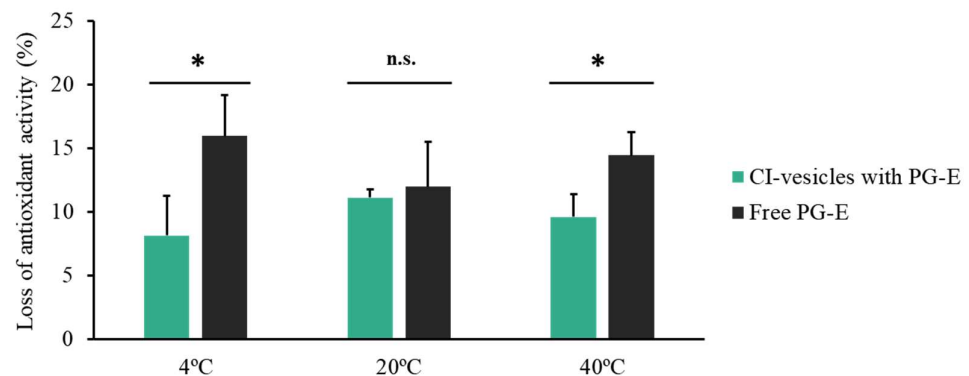
Figure 3. – Loss of antioxidant activity (%) with respect to the initial time for pomegranate extract (PG-E), encapsulated in CI-vesicles or free, after 90 days of storage at 4°C, 20°C or 40°C. Data are means \pm SE (n = 3). *, significant differences compared to the respective control ( p < 0.05 ). n.s., not significant.
