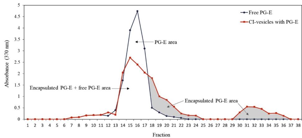
Figure 1. – Absorbance (370 nm) of each fraction obtained after passing through a Sephadex column samples of free PG-E (blue line) and CI-vesicles with encapsulated PG-E (red line). The grey area indicates the proportion of PG-E encapsulated in CI-vesicles.
