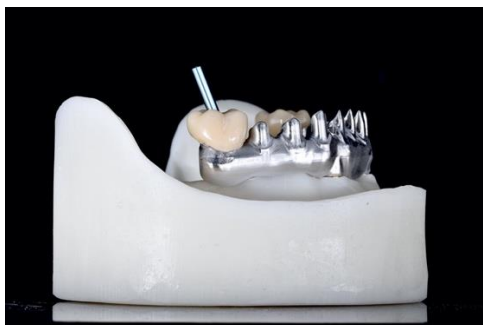
Figure 3. CAD/CAM Cr-Co Milled Framework
