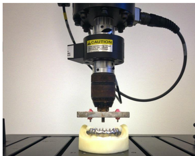
Figure 4. Electrodynamic testing machine (MTS-Acumen 1) simulating masticatory cycles on the implant supported prosthesis.
