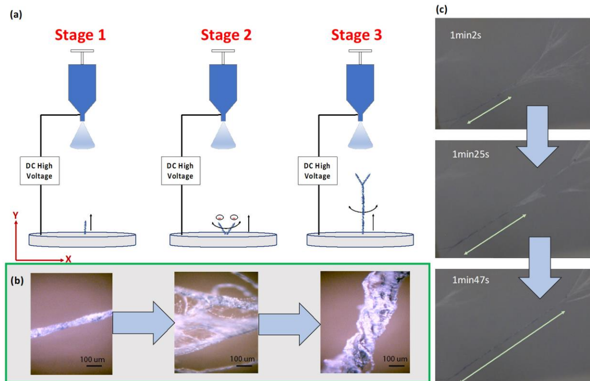
Figure 1. (a) Schematic diagram of nanofiber yarn formation. Stage 1: Individual standing fibers populate the collector plate and lengthen. Stage 2: Fibers bundles twist from electrostatic and mechanical forces to form yarn with neighboring fibers. Stage 3: Newly spun nanofibers attach to the growing yarn structure and continue to twist about the longitudinal axis. (b) Structural transformation from a single fiber to a yarn, demonstrating collection of single fibers into an organized structure in stage 2 and 3. (Scale bar: 50 ) (c) Time lapse sequence of stage 3 nanofiber yarn formation at 62, 85 and 107 seconds.
