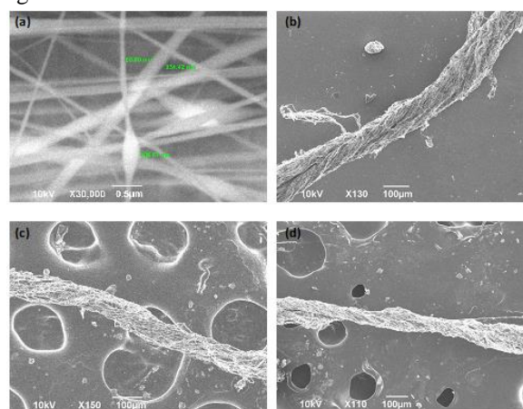
Figure 4. SEM pictures of the PEDOT/PVA structure (a) without treatment (b) with treatment obtained from the electrostatic fabrication method. (c) Nanoyarn Material B [see Table 1] after electrospinning for 10 min. (d) Nanoyarn Material B after electrospinning for 20 min.
