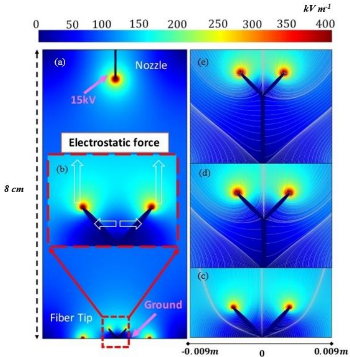
Figure 2. Electric field lines in the region between the needle and the collector. (a) Normalized electric field distribution at stage 2 of fabrication showing model configuration. The black straight line represents the charged tip of the needle. The two ‘rice’ shapes represent the two standing fiber tips attached to the grounded collecting plate. (c-e) Electric field lines formed near fiber tips in (c) stage 2 and (d, e) stage 3.
