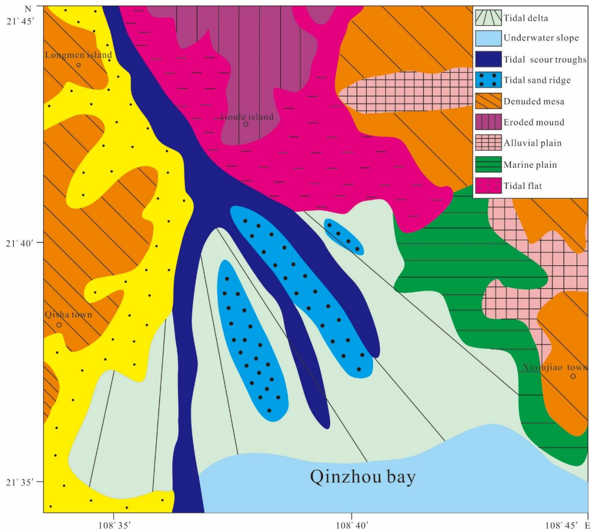
Figure 4. Coastal zone and submarine geomorphology in the research area
