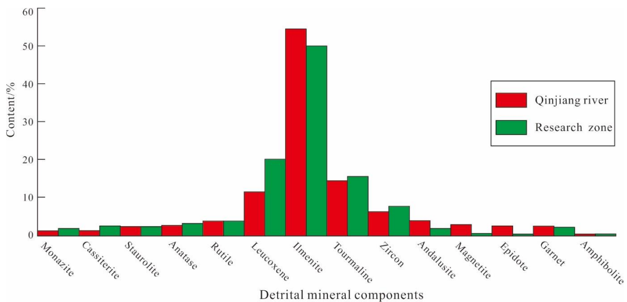
Figure 6. Comparison of terrestrial heavy mineral contents of surface sediments between outer Qinzhou Bay and the Qinjiang River
