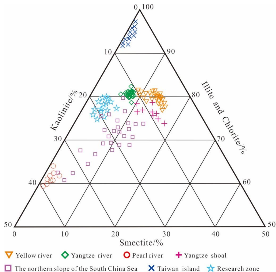
Figure 7. Diagram indicating the contents of three major clay minerals in the sampled sediments
