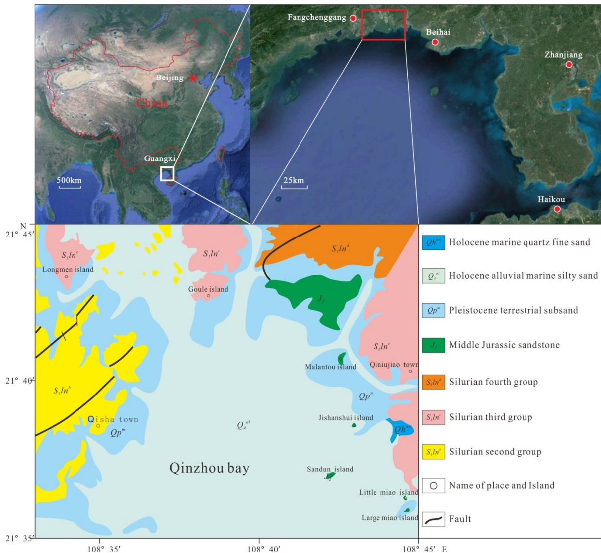
Figure 1. Diagram of regional structures and stratum structures in the research area
