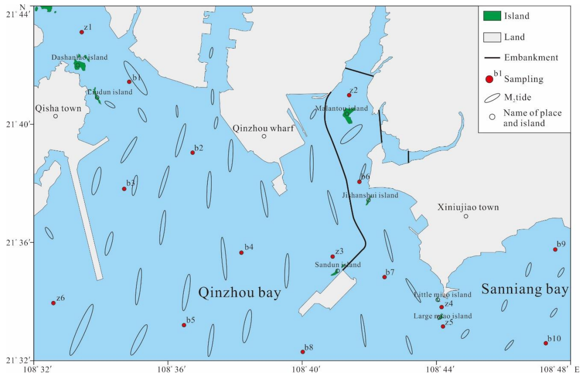
Figure 2. Distribution of sampling sites in the research area
