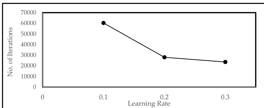
Figure 3. No. of iterations for coverage vs. Learning rate
