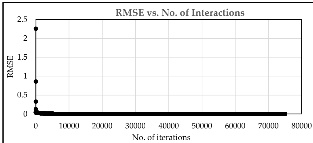
Figure 2. Root Mean Square Error (RMSE) vs. No. of Iterations
