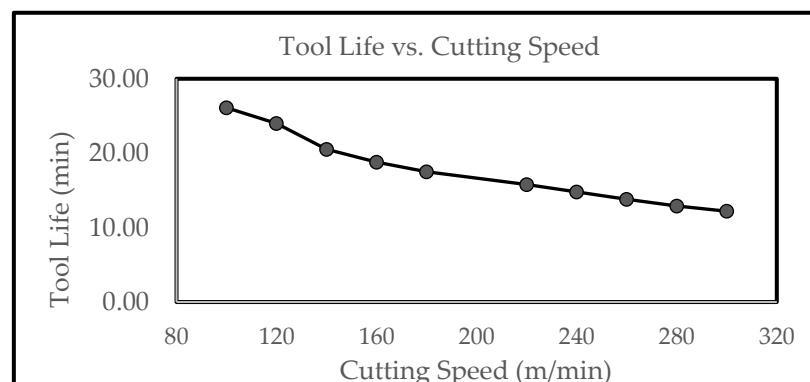
Figure 1. Cutting Speed vs. Tool life of Ti [C,N] mixed ceramic cutting insert
