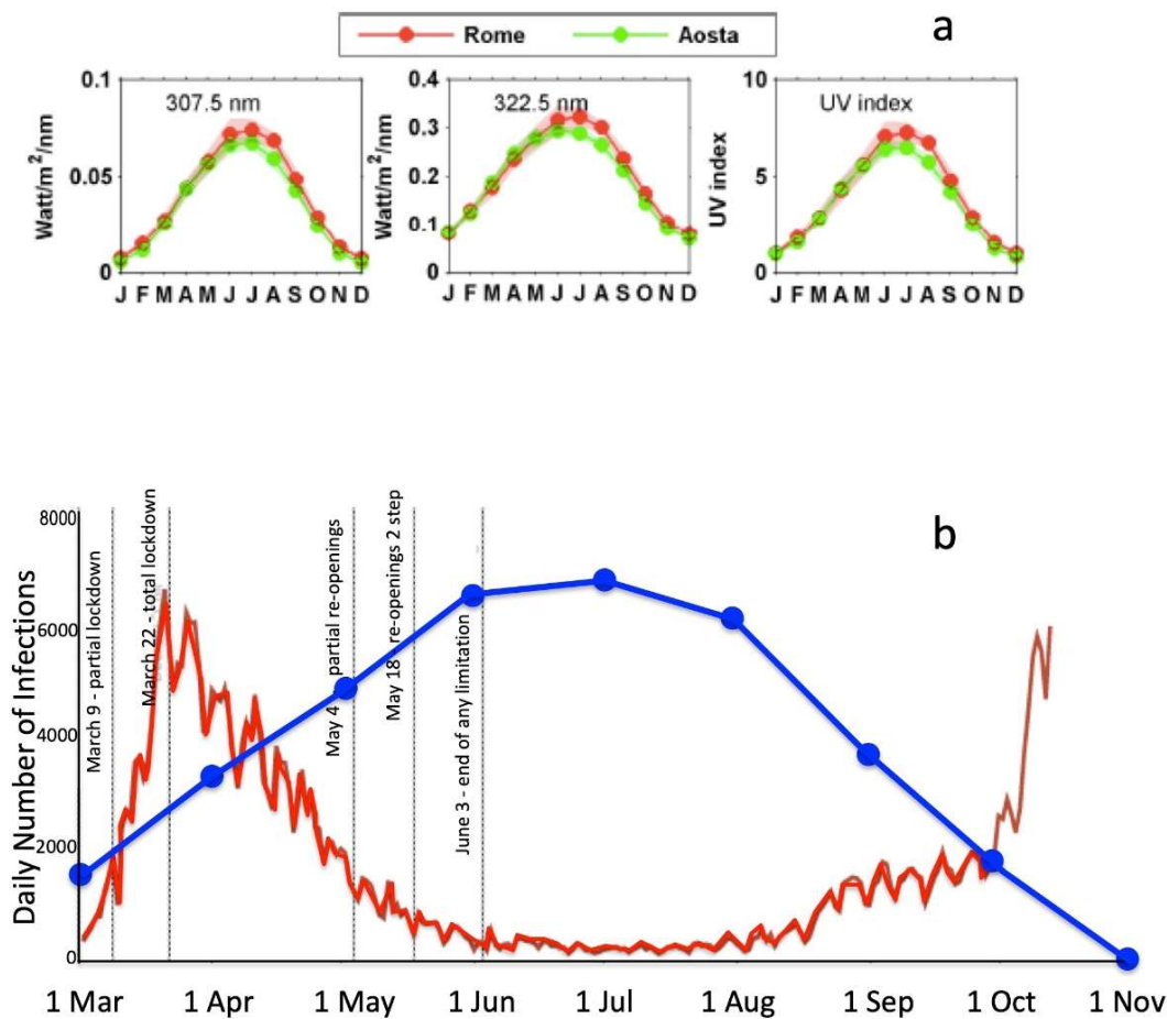
Fig.3 a) From left to right: climatologies of the irradiance at 307.5 nm, 322.5 nm, and the UV index at two stations in Italy: Aosta, Northern Italy, Rome, Central Italy, in the period 2006–2015. Shaded envelopes correspond to the standard deviation of the climatological values and the average ratios (redrawn from [21]). b) Comparison of the official daily infection curve in Italy from March to mid-October (red line) with the average (2006-2015) UV intensity curve recorded at Rome station (as shown in a), in the period March to November. Note the clear anti-correlation of the two curves, with minimum infection corresponding with maximum UV intensity in the summer months.
