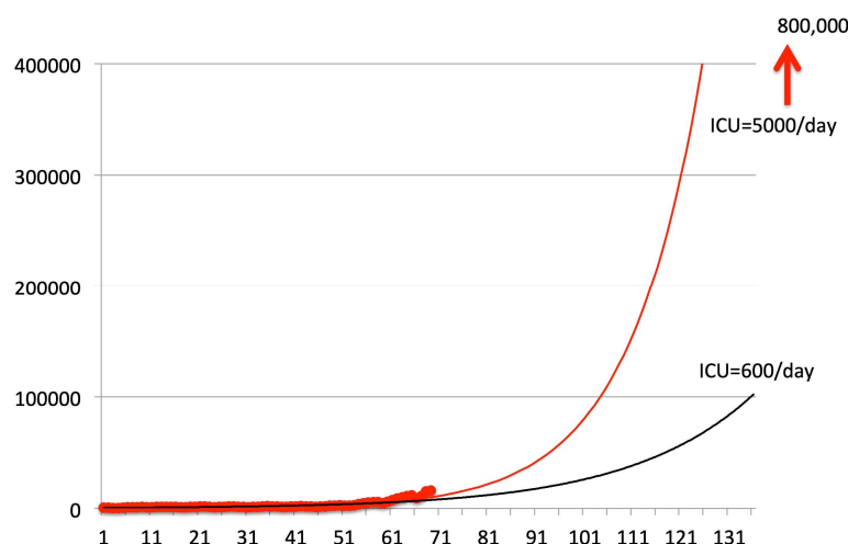
Fig.4 Extrapolated exponential curves for daily infection data since August 15th to October 23 rd (red circles). The best fitting exponential curve for all data is shown by the black line; red line shows the best fitting curve using only data since September 15 th to October 23 rd .
