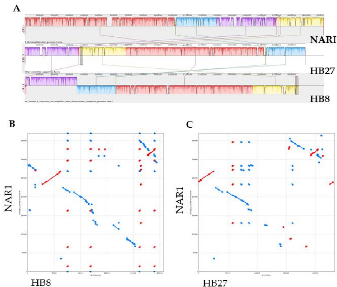
Figure 2. Synteny of TthNAR1 replicons with other Tth strains. A) Alignment of (up to down) Tth strains NAR1, HB27 and HB8 chromosomes with Mauve (no connection lines). The sequence has been divided in four section colours corresponding to syntenic regions to facilitate the visualization. Dotplots of TthNAR1 370 kbp megaplasmid against pTT27 megaplasmids found in HB8 (B) and HB27 (C).
