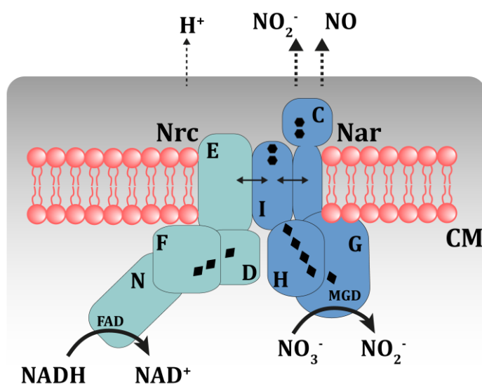
Figure 4. A putative nitrate respirasome in TthNAR1. This scheme shows the likely structure of the nitrate respirasome, included the Nrc NADH dehydrogenase complex and the nitrate reductase. Activity of the complex will separate protons. Interactions detected by two-hybrids assays are indicated as double arrowheads lines. Heme groups are indicated as black hexagons and iron sulfur clusters as diamonds. The role of the NarC component of the NR as electron transporter towards NOR and NOS enzymes is indicated as discontinuous arrows.
