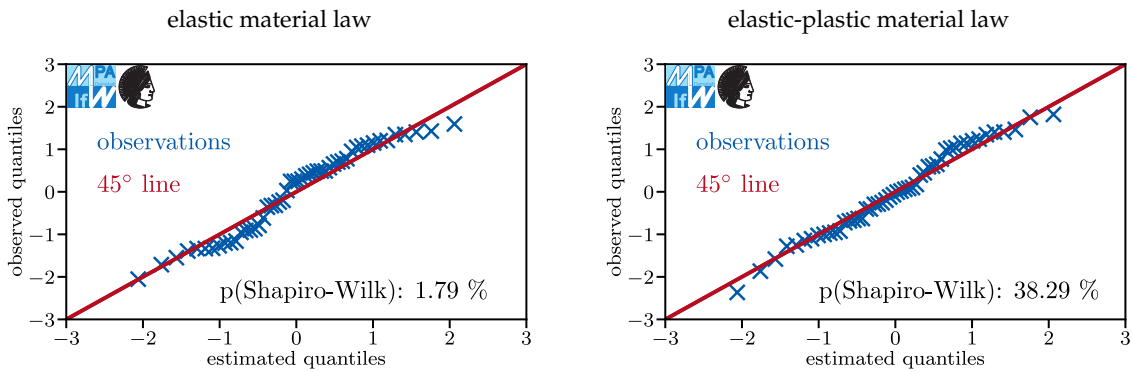
Figure 20. Quantile-quantile plots for 50CrMo4 specimens in laboratory air; 919 MPa ultimate tensile strength; K_t = 1 .
