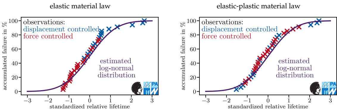
Figure 17. Estimated and observed accumulated failure rates for 50CrMo4 specimens in laboratory air; 919 MPa ultimate tensile strength; K_t = 2.06 .
