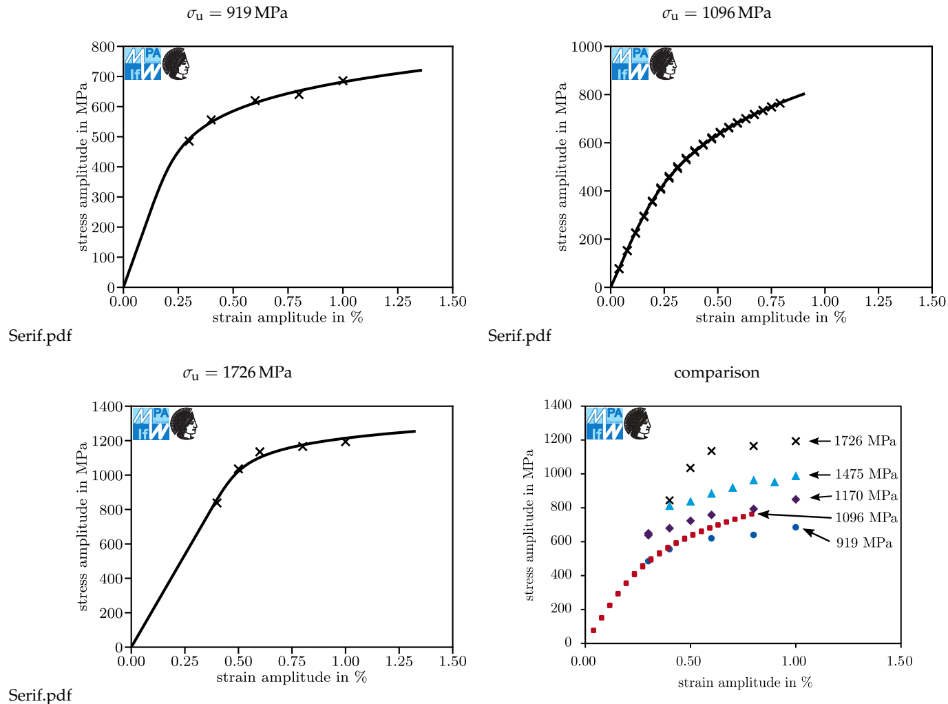
Figure 6. Cyclic stress strain curves. First row: 919 MPa and 1096 MPa ultimate tensile strength. Second row: 1726 MPa ultimate tensile strength (left) and comparison of batches with 919 MPa, 1096 MPa, 1170 MPa, 1475 MPa and 1726 MPa ultimate tensile strength.
