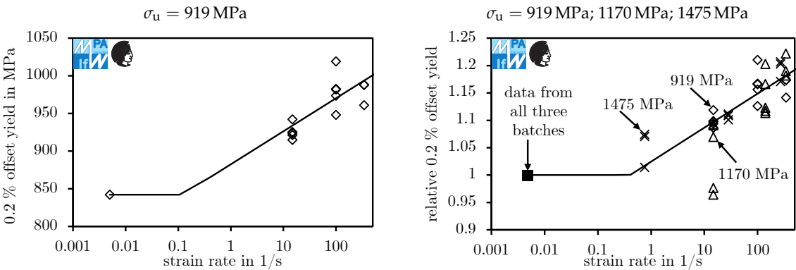
Figure 5. 0.2% offset yield depending on the strain rate, for the 919 MPa ultimate tensile strength (left) and for the batches 919 MPa, 1170 MPa and 1475 MPa (right).
