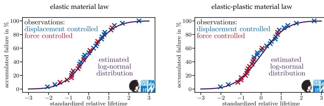
Figure 18. Estimated and observed accumulated failure rates for 50CrMo4 specimens in laboratory air; 1096 MPa ultimate tensile strength; K_t = 1.2 .
