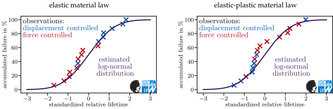
Figure 15. Estimated and observed accumulated failure rates for 50CrMo4 specimens in laboratory air; 919 MPa ultimate tensile strength; K_t = 1.75 .
