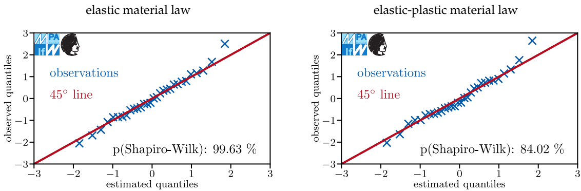
Figure 24. Quantile-quantile plots for 50CrMo4 specimens in laboratory air; 1096 MPa ultimate tensile strength; K_t = 1.2 .
