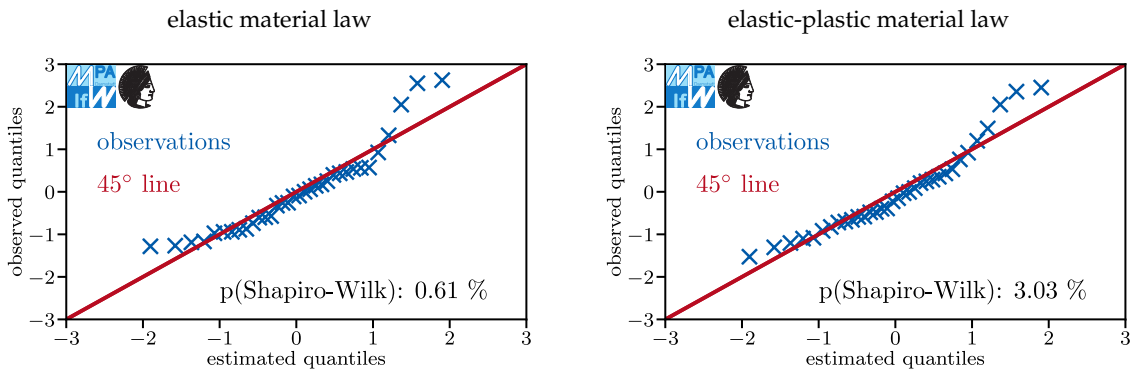
Figure 23. Quantile-quantile plots for 50CrMo4 specimens in laboratory air; 919 MPa ultimate tensile strength; K_t = 2.06 .
