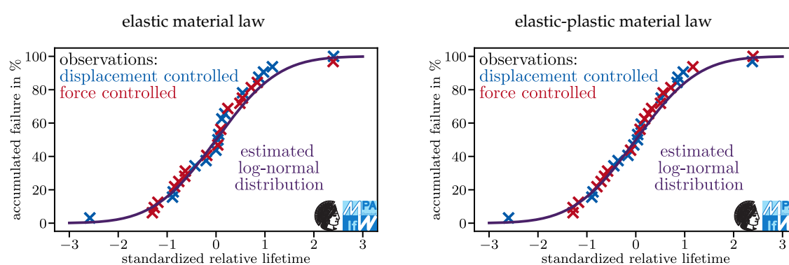
Figure 19. Estimated and observed accumulated failure rates for 50CrMo4 specimens in laboratory air; 1726 MPa ultimate tensile strength; K_t = 2.06 .
