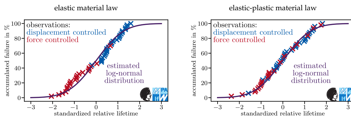
Figure 14. Estimated and observed accumulated failure rates for 50CrMo4 specimens in laboratory air; 919 MPa ultimate tensile strength; K_t = 1 .
