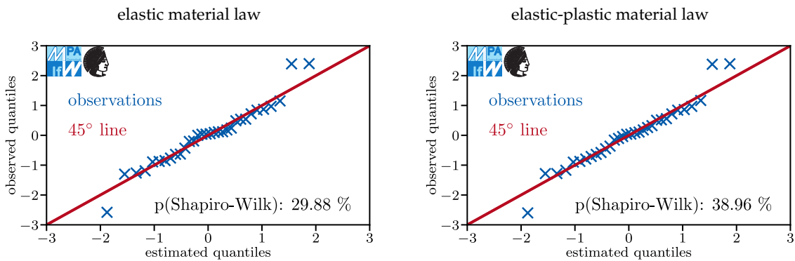
Figure 25. Quantile-quantile plots for 50CrMo4 specimens in laboratory air; 1726 MPa ultimate tensile strength; K_t = 2.06 .
