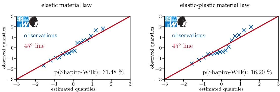
Figure 21. Quantile-quantile plots for 50CrMo4 specimens in laboratory air; 919 MPa ultimate tensile strength; K_t = 1.75 .
