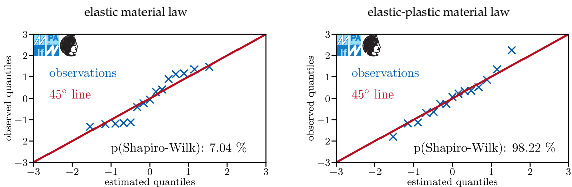
Figure 22. Quantile-quantile plots for 50CrMo4 specimens in argon; 919 MPa ultimate tensile strength; K_t = 1.75 .
