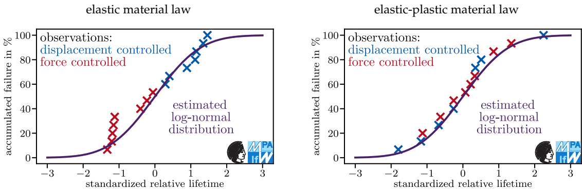
Figure 16. Estimated and observed accumulated failure rates for 50CrMo4 specimens in argon; 919 MPa ultimate tensile strength; K_t = 1.75 .
