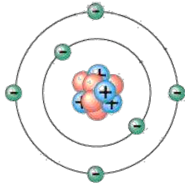
Carbon atom
