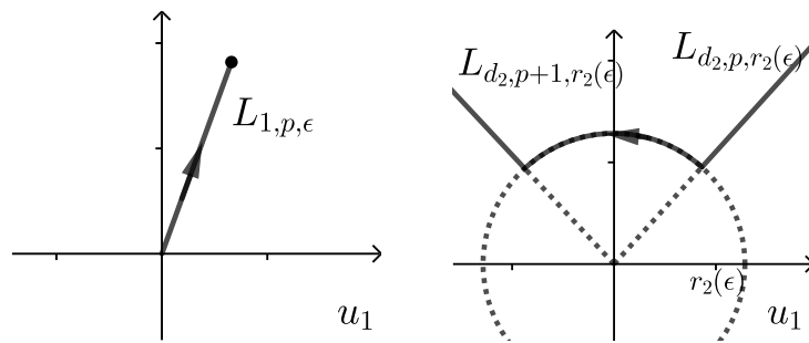
Figure 2: Deformation of the integration path. Case 1
