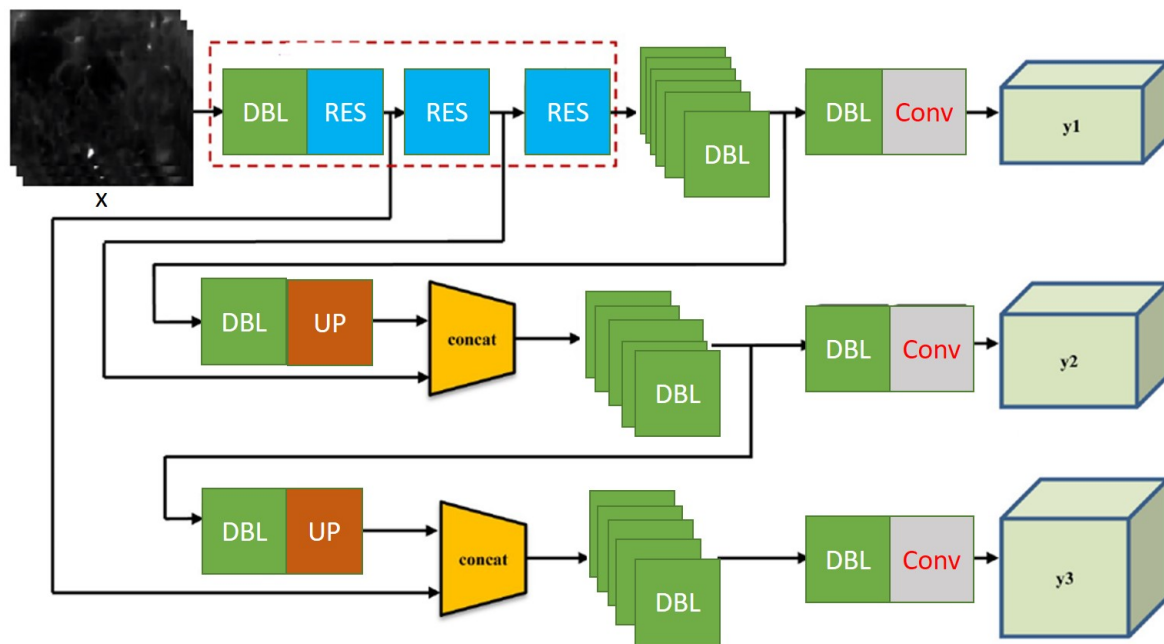
Figure 3. YOLOv3 architecture with input image size 416 \times 416 and 3 types of feature map ( 13 \times 13 \times 3 , 26 \times 26 \times 3 and 52 \times 52 \times 3 ) as output; (B) DBL is Darknet conv2D BN Leaky composed of one convolution layer, one batch normalisation layer and one leaky relu layer.; ResUnit includes two "DBL" structures followed by one "add" layer leads to the residual-like unit, "ResBlock" has several "ResUnit" with one zero-padding layer and "DBL" structure forward generates a residual-like block, "ResBlock." is the module element of Darknet-53.
