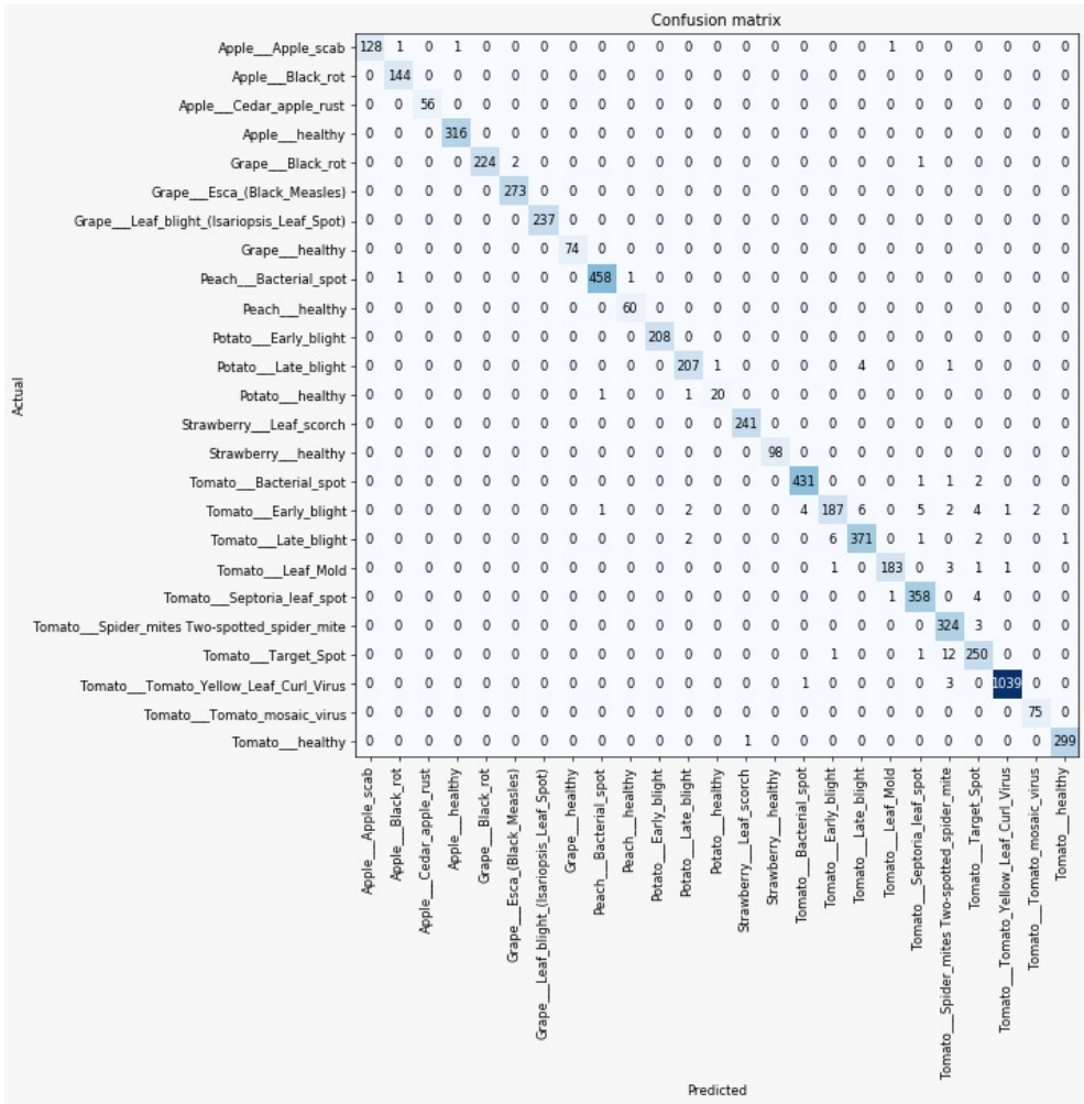
Figure 11. Confusuion Matrix for 80 -20 % Data Split.
