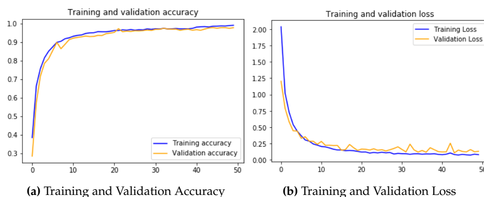
Figure 10. Training and Validation Graphs
