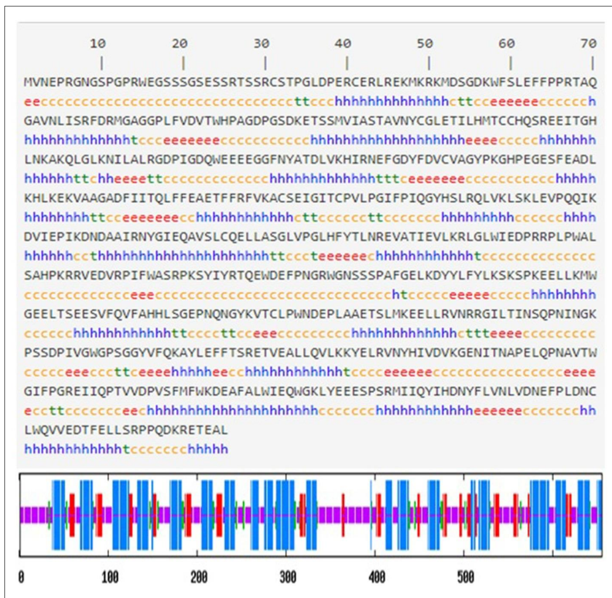
Supplementary figure 4. Predicted secondary structure of Bos taurus MTHFR. The long vertical zone: Alpha helix (h); The middle vertical zone: Extended strand (e); The short vertical zone: Random coil (c). The secondary structure was predicted by SOPMA online software
