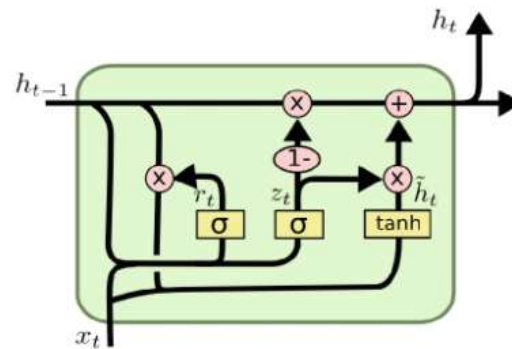
Figure 7 Gated Recurrent Unit
