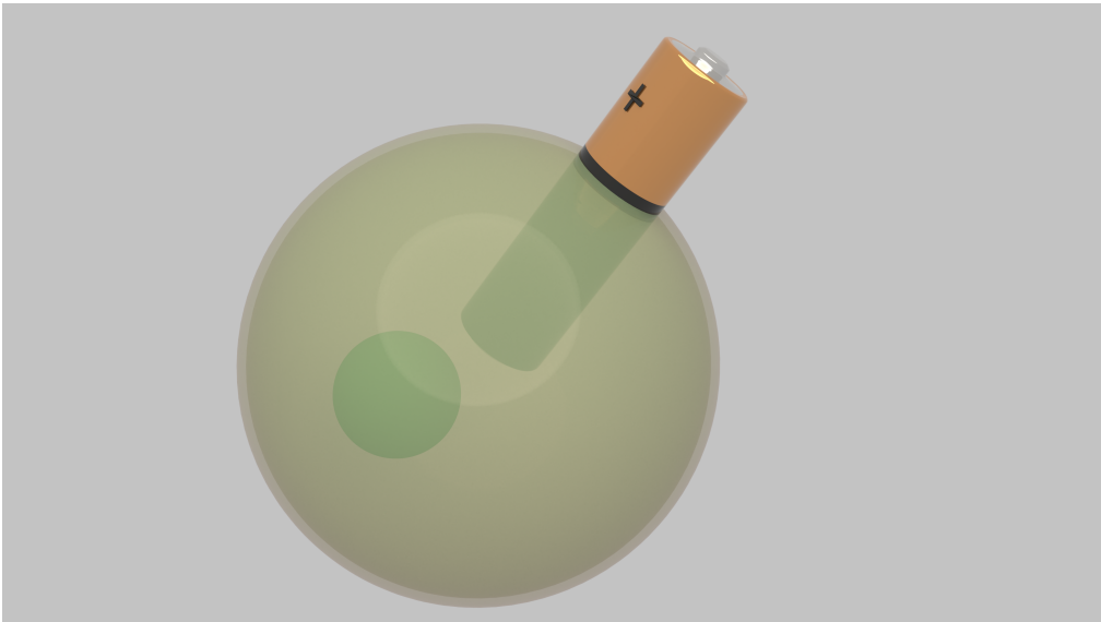
Figure 2. Example of a "cell" in a real situation. As the measuring devices are no longer electrically connected, the properties are no longer accessible and no more necessarily electrical. If there are any, then the forces involved are chemical, electrostatic, coulombic and mechanical.
