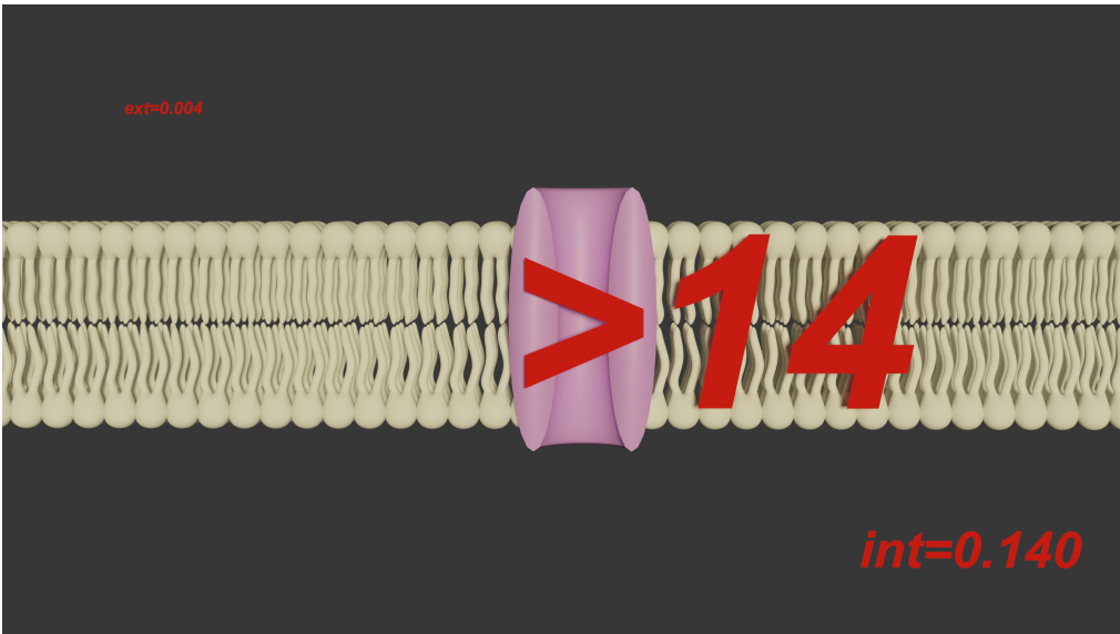
Figure 5. Membrane concentration profile. Considering the different concentrations present, the ion channel always has the highest concentration. Indeed, it is stated that diffusion takes place through these channels. In such a case, the membrane concentration profile shows that it is not possible for diffusion to take place as the theory would suggest. The concentration in the ion channel is at least 14 moles: such a concentration defies chemists and biologists.
