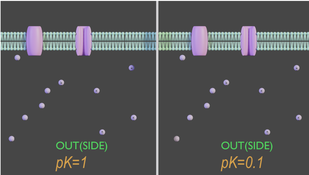
Figure 4. Permeability and charge imbalance. If there is a charge difference between the two sides of the membrane then the permeability has no influence on the potential difference. The computation remains the same and the permeability can in no way change the electrical value of the charge.
