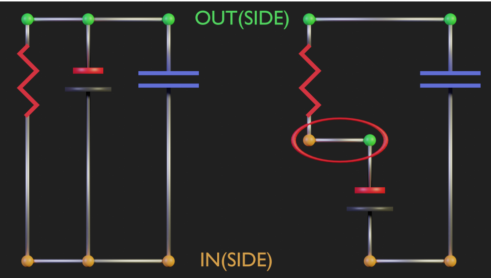
Figure 3. Comparison of electrical circuits. The circuit on the left is made and connected with the anatomical definitions and locations of the "electrical components". The model on the right is the famous HH model. There is a big problem because it connects components with wrong anatomical localization of some "terminals". This leads to a short circuit (red circle) with all the consequences that can be expected.
