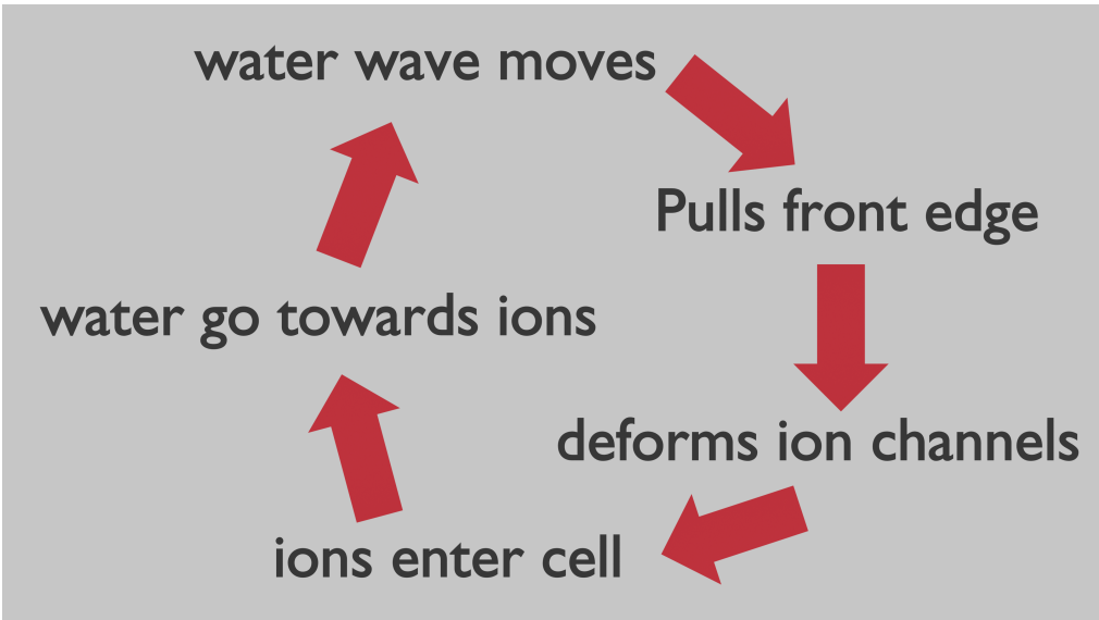
Figure 6. Action potential propagation cycle. Once the threshold is exceeded, the amount of water mobilized is sufficient to deform the membrane at the rising front of the action potential. The membrane is then stretched to deform the ion channels and allow the entry of ions. This results in a movement of water towards the incoming ions and a pressure drop at the falling front. The cycle is then repeated.
