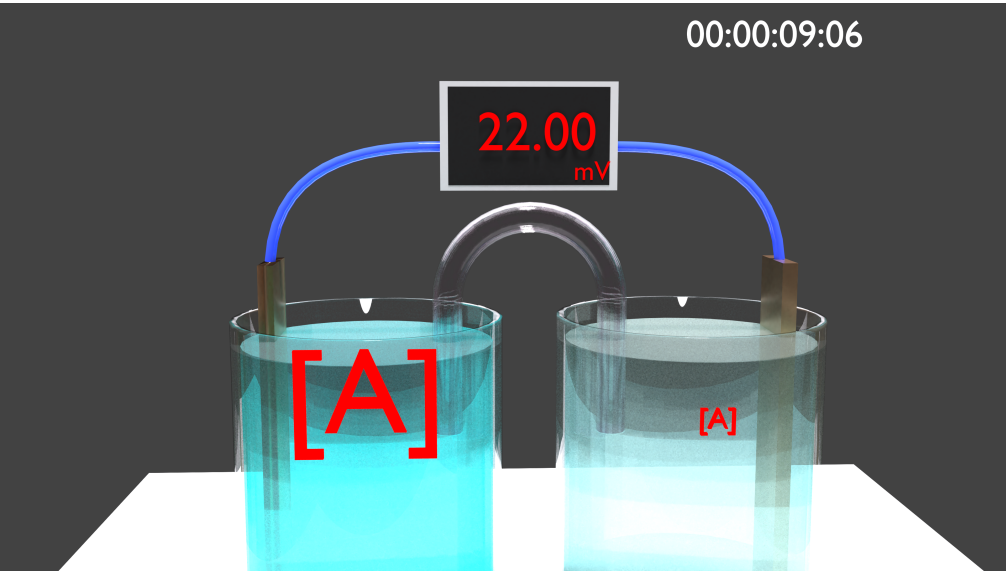
Figure 1. Example of an electrochemical cell. There is a potential because there are chemical reactions at the interfaces and the compartments are connected to each other by an external electric circuit and an ionic circuit is thus created in the electrolytes.
