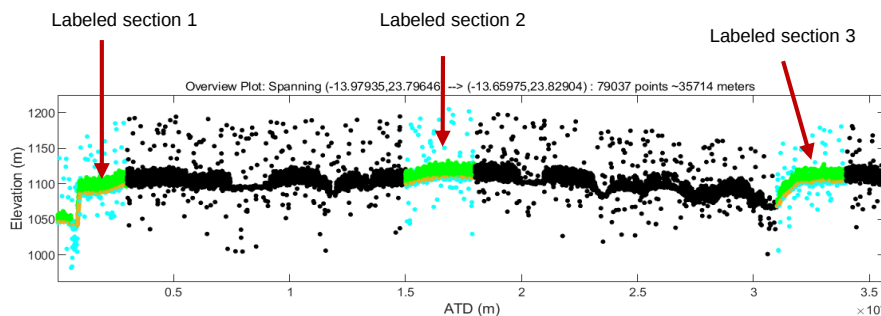
ATL03 data with sections of labeled data
