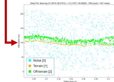
Sample labeled ATL03 data over forested area in eastern Texas
