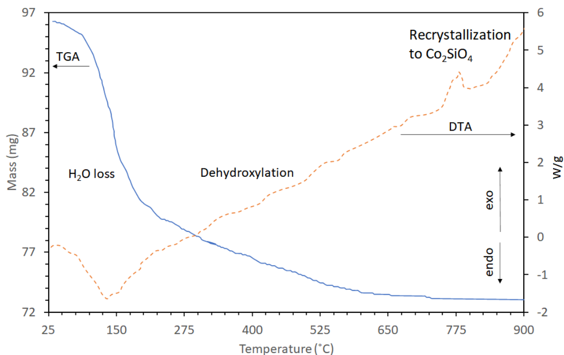
Figure 9. Thermogravimetric (TGA) and differential thermal analysis (DTA) of Co-saponite (Al 3+ exchanged). Modified from Figure 1 [44].
