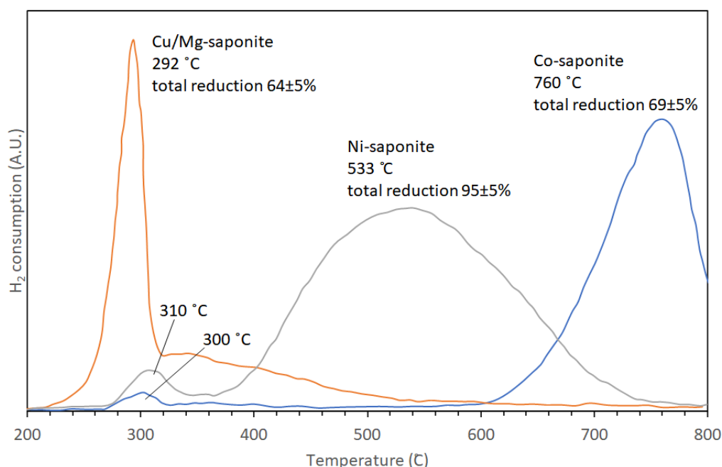
Figure 12. Temperature-programmed reduction profiles of Cu-, Ni-, and Co-containing saponites. Modified from Figure 6 in [44].
