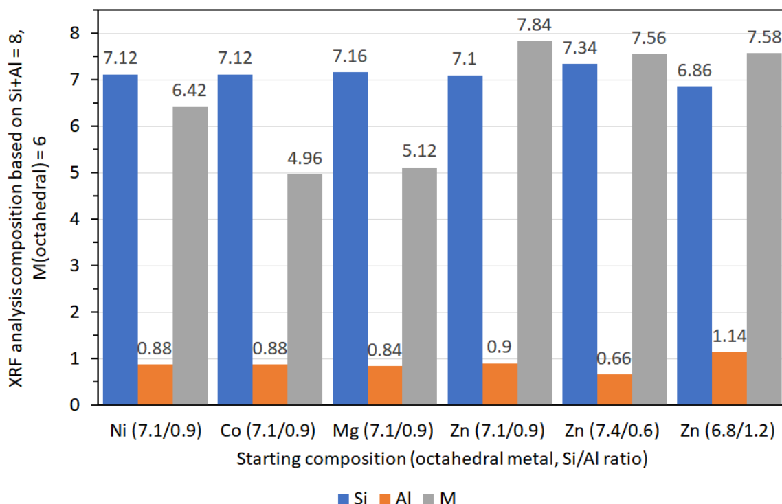
Figure 8. XRF analyses of different M-saponites (M=Ni, Co, Mg, Zn) and Zn-saponite with different Si/Al ratios. Results based on Table 5 of [24].
