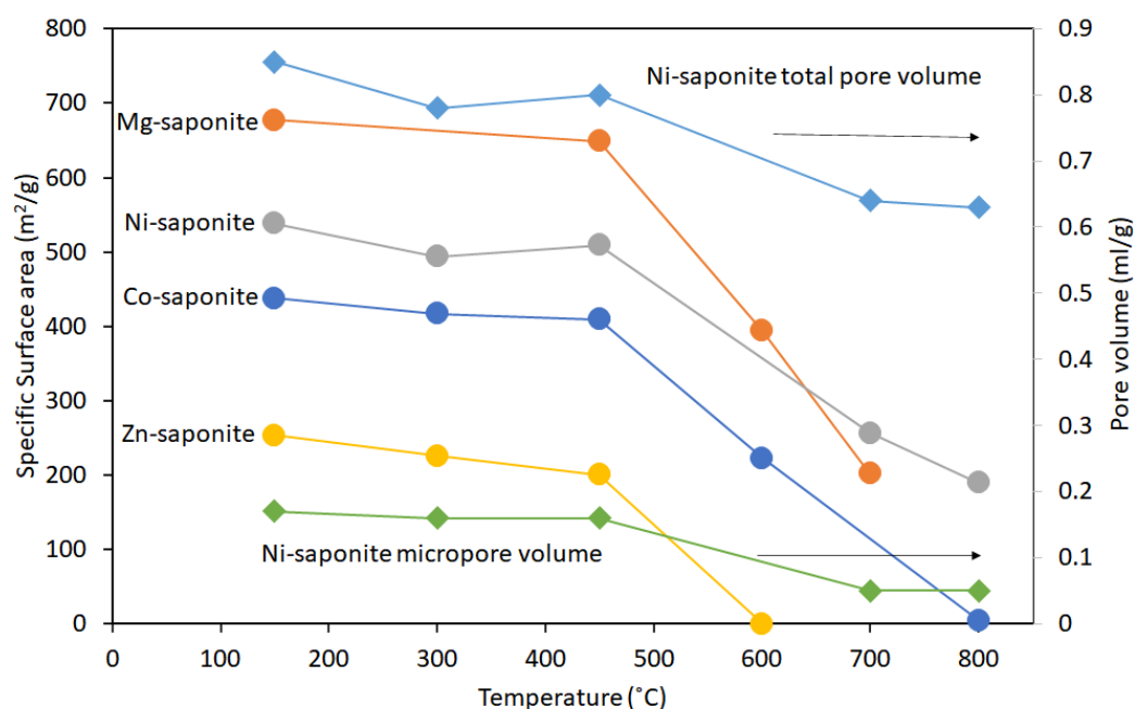
Figure 11. BET surface area and pore volume as function of calcination temperature of M-saponites (M=Mg, Ni, Co, Zn). Modified from Figure 3 in [44].
