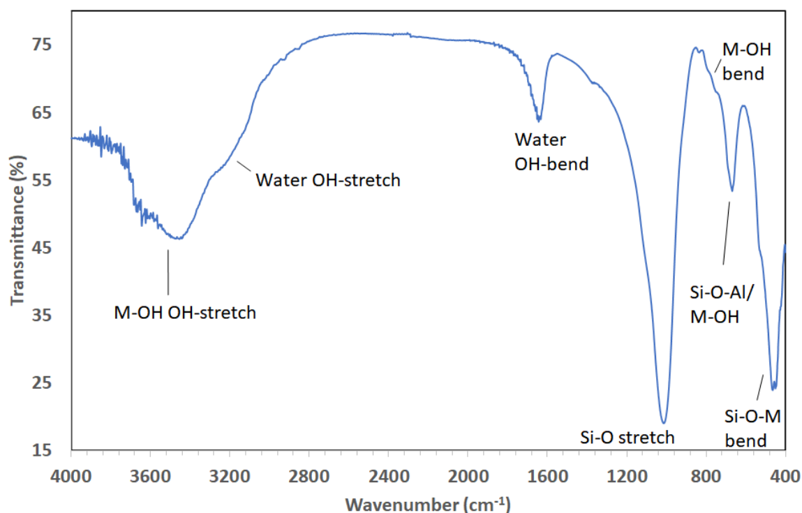
Figure 3. Typical IR spectrum of a synthetic Mg-saponite synthesized in 20 hours with 72.1 g urea. The IR spectrum was collected using a Perkin Elmer (1600 series) spectrometer in transmission mode using 256 scans at 4 \text{cm}^{-1} resolution using a KBr tablet (5 mass% sample).
