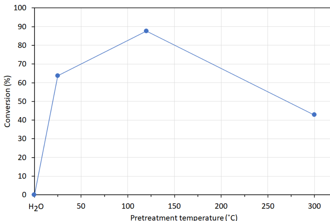
Figure 15. The influence of the hydration state of 0.2 wt% Zn-saponite (Si/Al ratio 7.89) on the catalytic activity. H 2 O means wet saponite sample. Reaction conditions: temperature 160 °C, duration 0.25 h, benzene/propylene molar ratio ~ 7. Modified from Figure 5 in [50].
