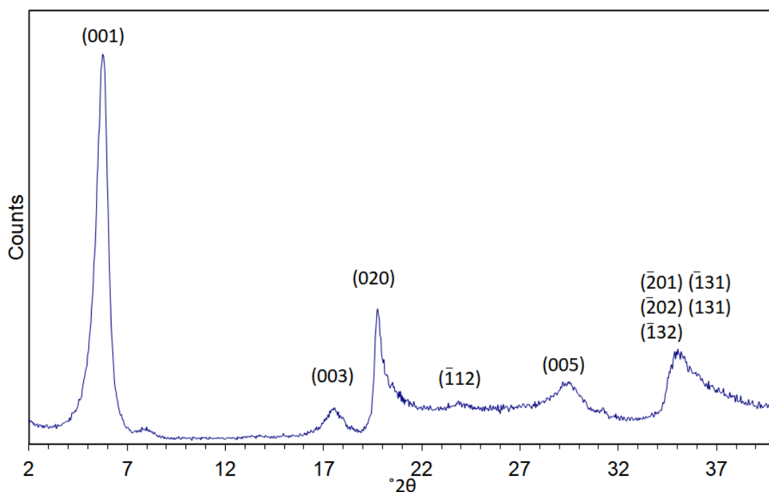
Figure 2. Typical X-ray diffraction pattern of a synthetic Zn-saponite synthesized for 20 hrs with 72.1 g urea. Based on data from [27]. Note: no vertical axis was given in the original publication.
