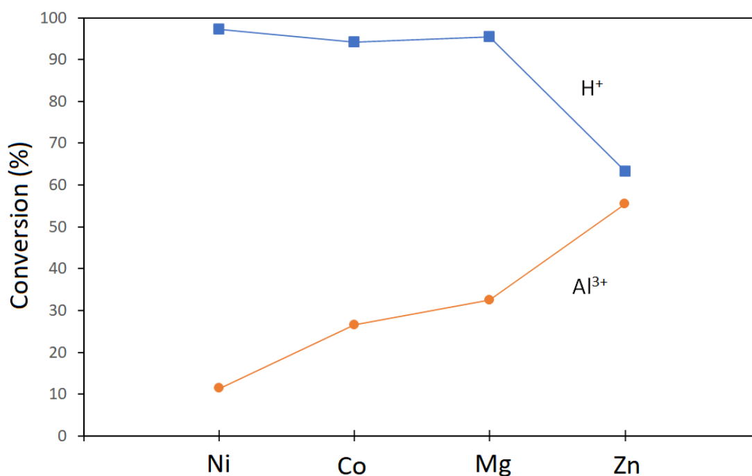
Figure 16. The influence of the composition of the octahedral sheet ( \text{Ni}^{2+} , \text{Co}^{2+} , \text{Mg}^{2+} , and \text{Zn}^{2+} ) with (blue) \text{H}^+ - and (orange) \text{Al}^{3+} -exchanged saponites (Si/Al ratio 7.89) on the catalytic performance. \text{H}^+ -saponites: 1.5 wt% catalyst at 190 °C and 2 h, \text{Al}^{3+} -saponites: 0.2 wt% catalyst at 160 °C for 0.25 h. Modified from Figure 6 in [50].
