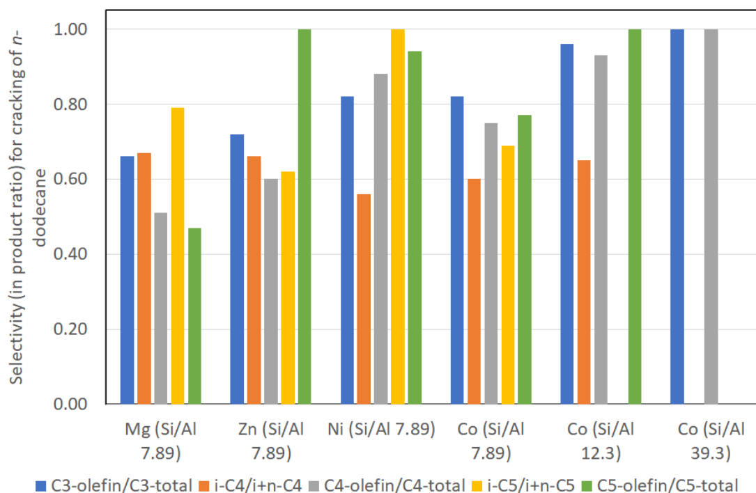
Figure 13. Selectivity expressed in product ratios for the cracking of n-dodecane. C = paraffin, i = iso, n = normal, total = total amount of olefins and paraffins. This figure is based on Table 2 of Vogels et al. [50].
