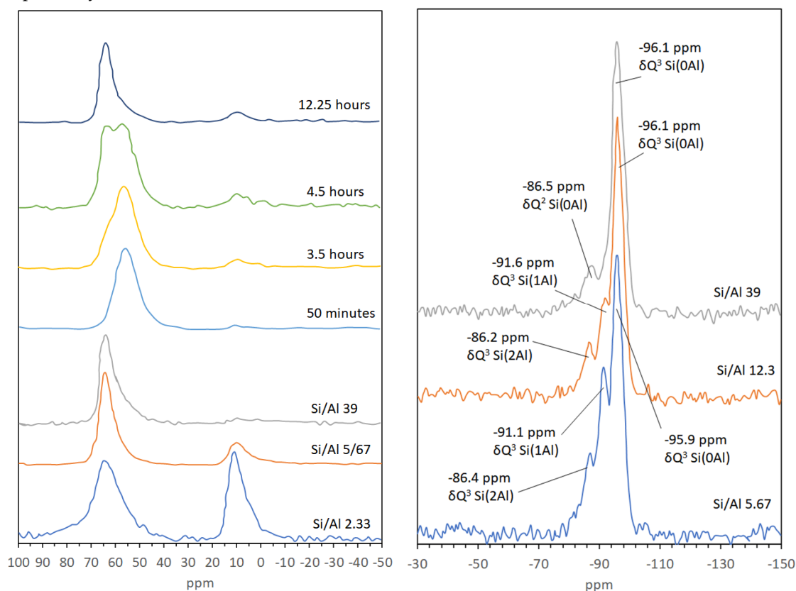
Figure 4. MAS-NMR of Zn-saponite with varying Si/Al ratio and varying synthesis time. ^{27}\text{Al} MAS-NMR (left) was performed at 130.321 MHz with a pulse length of 1 \mu\text{s} and a pulse interval of 1 second and chemical shifts ( \delta ) reported in ppm relative to [\text{Al}(\text{H}_2\text{O})_6]^{3+} . ^{29}\text{Si} MAS-NMR (right) was performed at 99.364 MHz with a pulse length of 6.5 \mu\text{s} and a pulse interval of 40s and chemical shifts ( \delta ) reported in ppm relative to [(\text{CH}_3)_4\text{Si}] . Modified from [27].
