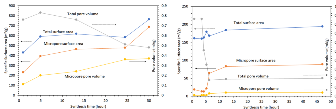
Figure 7. BET total and micropore surface area and pore volume of Mg- (left) and Zn-saponite (right) as function of synthesis time. These results are calculated based on Figure 5 in [27].
