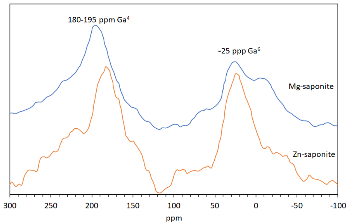
Figure 5. ^{71}\text{Ga} MAS-NMR of gallium substituted Mg- and Zn-saponite performed at 152.531 MHz with a pulse length of 2.0 \mu\text{s} and a pulse interval of 0.5 s and chemical shifts ( \delta ) reported in ppm relative to [\text{Ga}(\text{H}_2\text{O})_6]^{3+} . Modified from [45].
