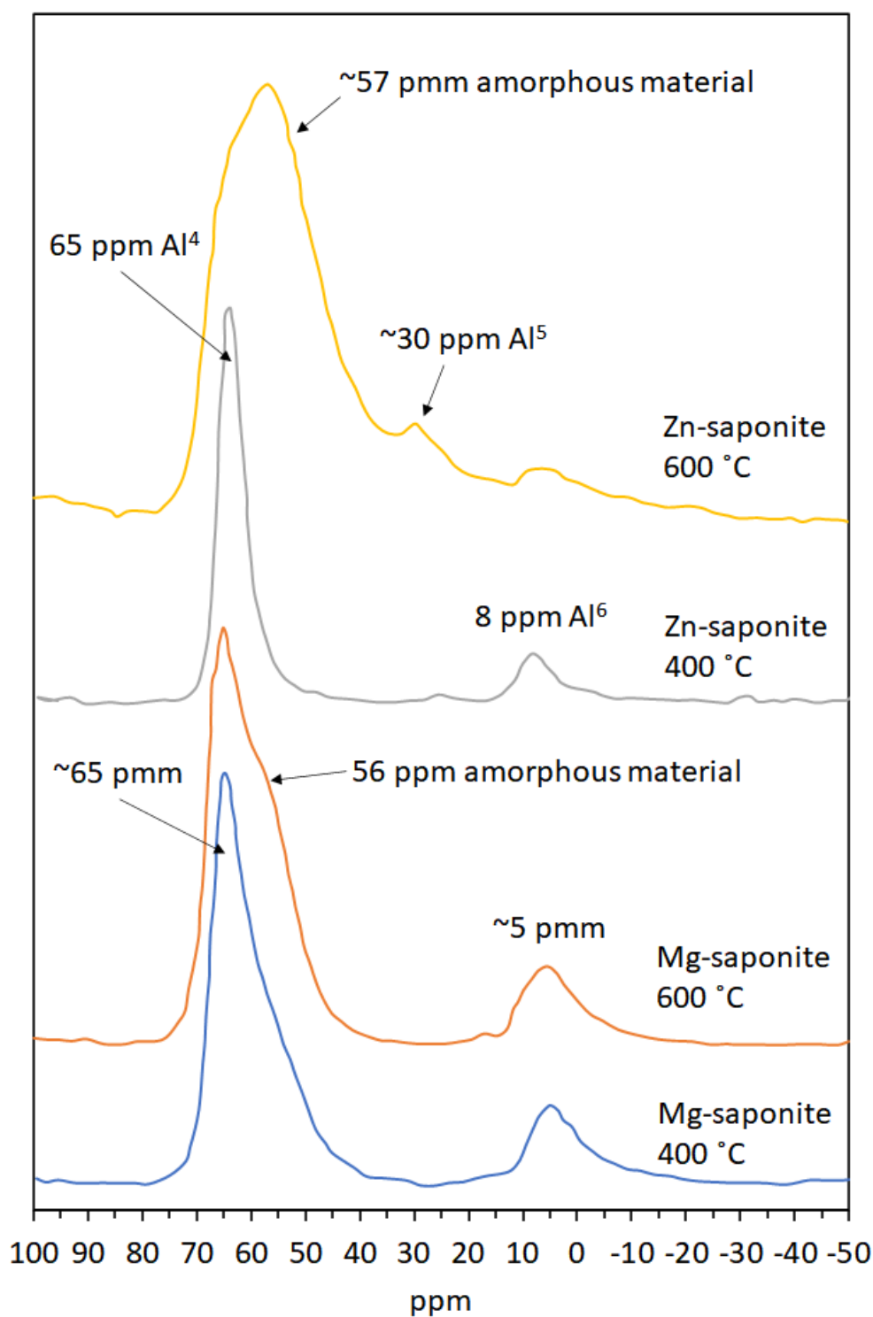
Figure 10. ^{27}\text{Al} MAS-NMR of Mg- and Zn-saponite thermally treated for 4 hours at 400 and 600 °C. Redrawn from Figure 2 in [44].
