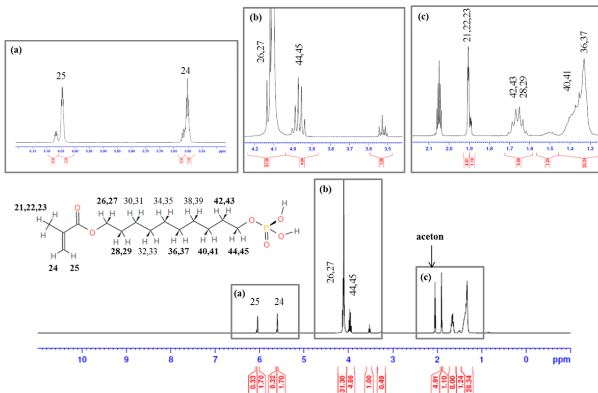
Figure 1. ^1\text{H} NMR spectrum of MDP.
