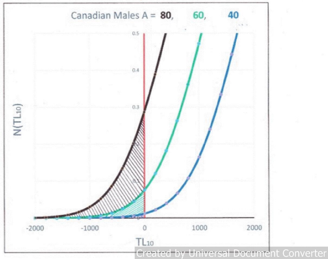
Fig 3: Number of individuals in the population/100K vs. their measured telomere length for ages=40, 60, and 80 years.
