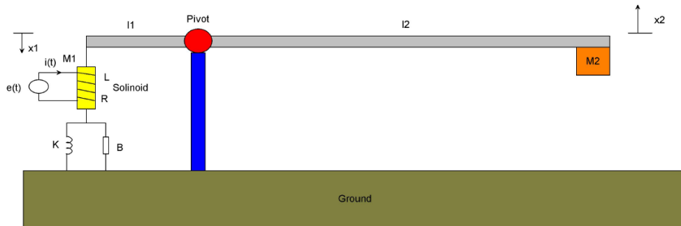
Figure 1 Vehicle boom barrier gate system design
