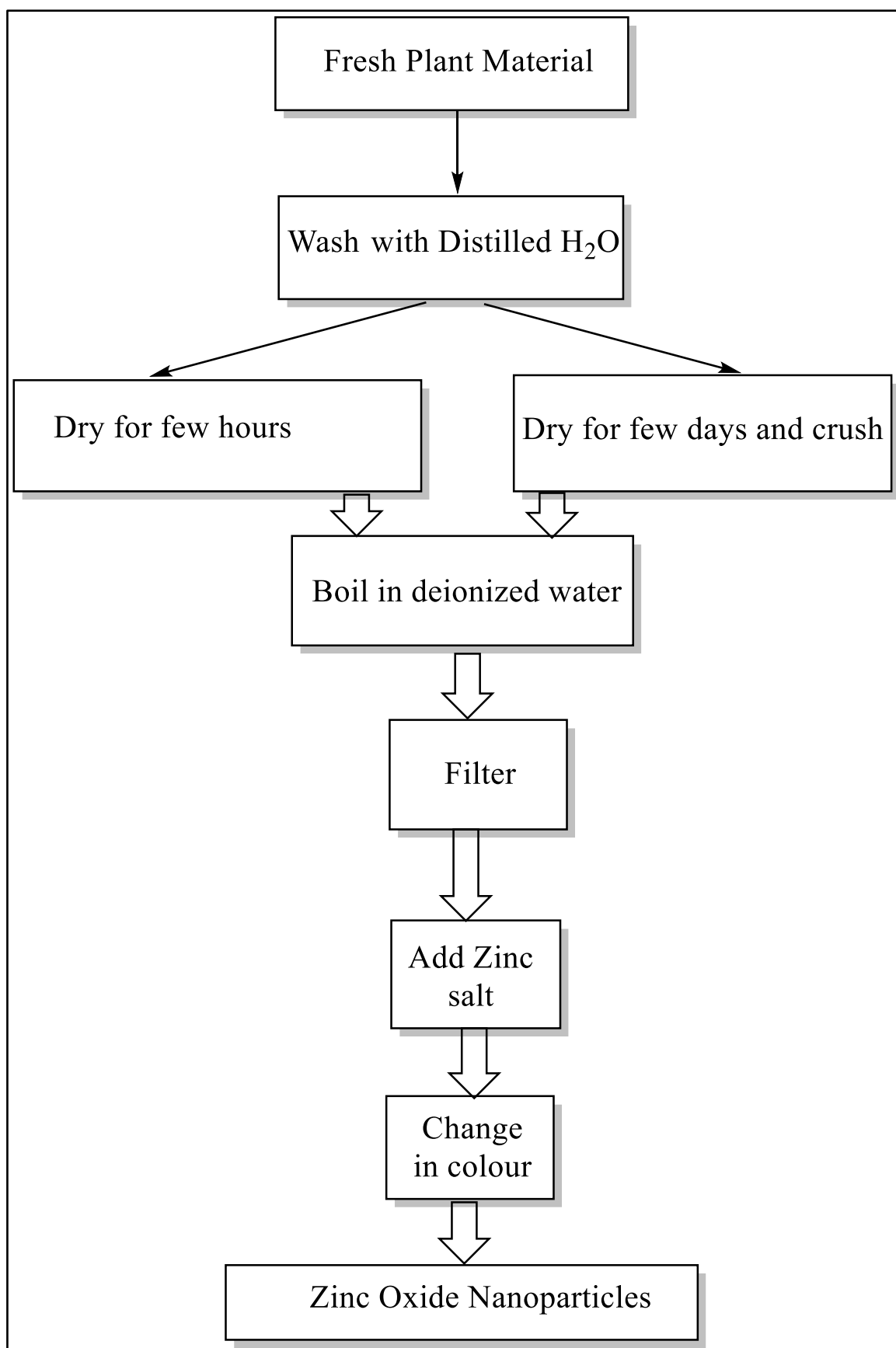
Figure 8: Protocol for Plant-Based-Green-Synthesis of ZnO NPs
