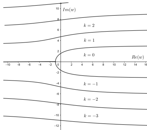
Figure 5: Branches of Lambert W function
