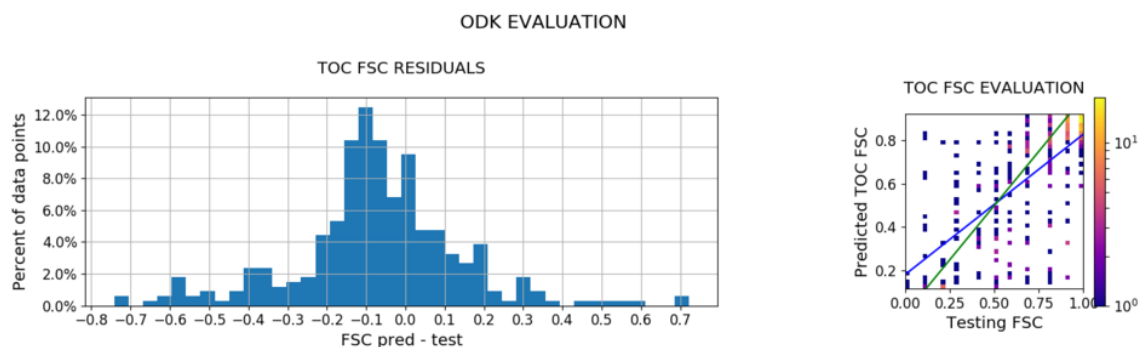
Figure 10. Results of the evaluation of the FSC using ODK data. Blue line: Linear regression between the predicted and the testing FSC sets. Green line: 1:1 line. The colour bar indicates the number of samples by bin.
