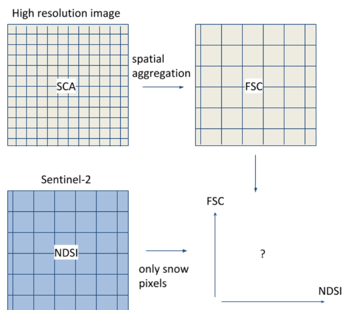
Figure 1. Schematic of the method used to determine the NDSI-FSC relationship. In this study the spatial aggregation is done using the average of all contributing pixels unless there is at least one no-data value, then the FSC pixel is set to no-data
