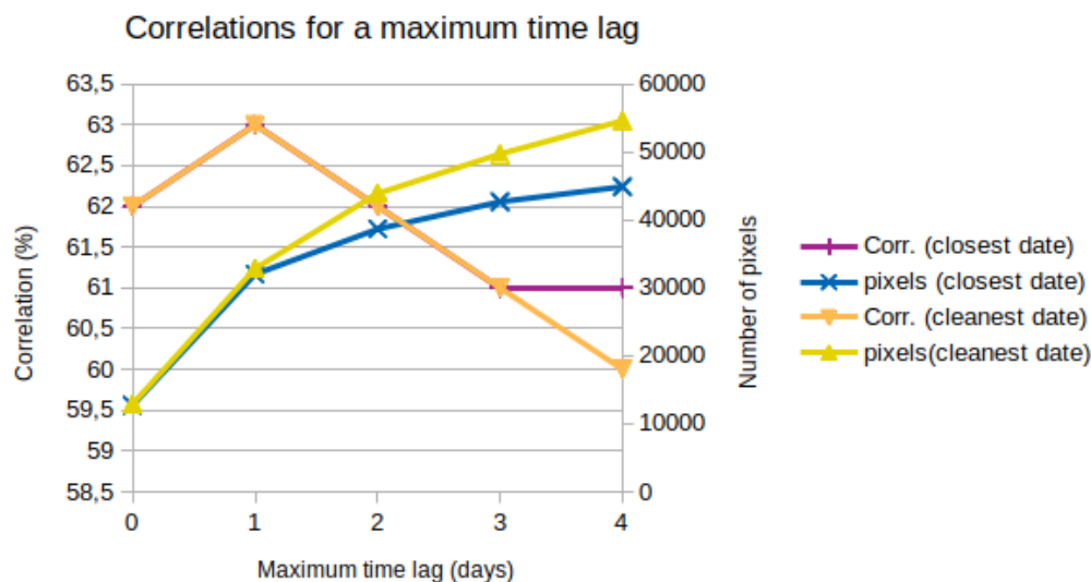
Figure 9. Evolution of the correlation coefficient between Sentinel-2 NDSI and Izas FSC and evolution of the number of pixels as a function of the time lag (plus or minus) for the 'cleanest' and 'closest' approaches.
