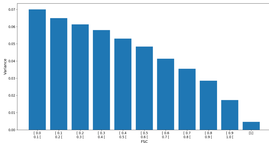
Figure 11. Variance of the residuals of the FSC retrievals from the Pléiades validation dataset (Sect. 3.1)
