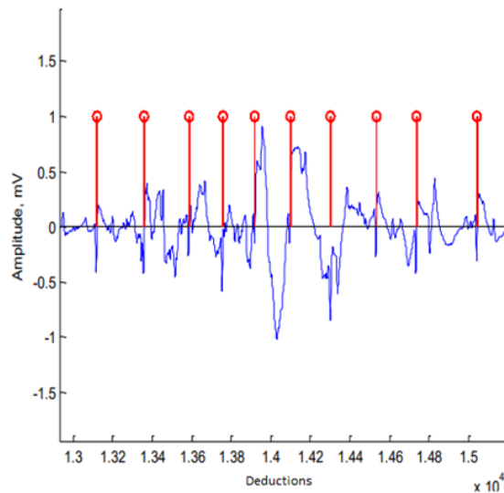
Figure 1. The registered electrocardiogram (ECG) signal and algorithm according to the maximum systole moments determined using the derivative value .
