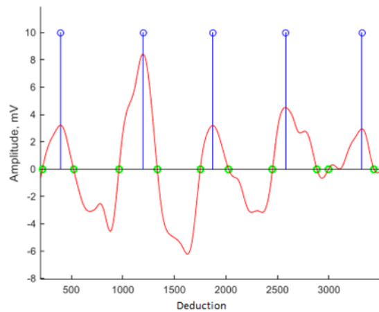
Figure 2. The cow breathing signal with algorithm-detected expiration moments.
