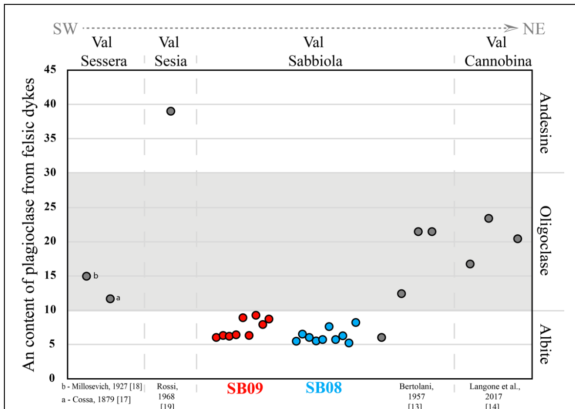
Figure 5. Anorthite content (An mol%) of plagioclase within corundum-bearing felsic dykes reported in different valleys of the of the IVZ, arranged from SW to NE. The red and blue circles show the composition of plagioclases for SB09 and SB08 dykes, respectively. The grey circles show the composition of plagioclases for other felsic dykes recognized in IVZ.
