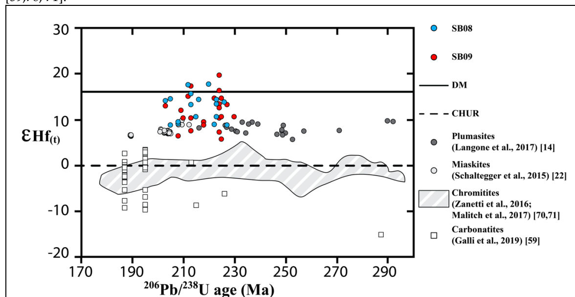
Figure 10 \epsilon\text{Hf}_{(t)} values from several magmatic bodies from IVZ. \epsilon\text{Hf}_{(t)} values are recalculated to the individual spot analysis ^{206}\text{Pb}/^{238}\text{U} ages.
