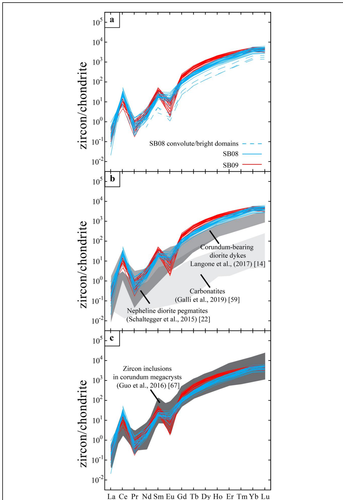
Figure 9. CI chondrite normalized REE patterns of zircon from SB09 and SB08 dykes (a), comparison with REE pattern of zircons of felsic dykes and carbonatites of the IVZ (b) and zircon included within corundum megacrysts in alkali basalts (c). Carbonaceous Ivuna (CI) normalization values are from McDonough and Sun [69].
