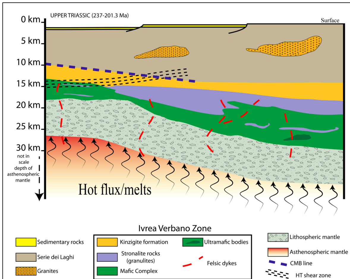
Figure 12 Schematic sketch of the IVZ lithospheric section at Upper Triassic showing the intrusion of felsic dykes in the middle/lower crustal levels. Black arrows indicate the hot flux/melt upraising from asthenosphere in an extensional tectonic regime.
