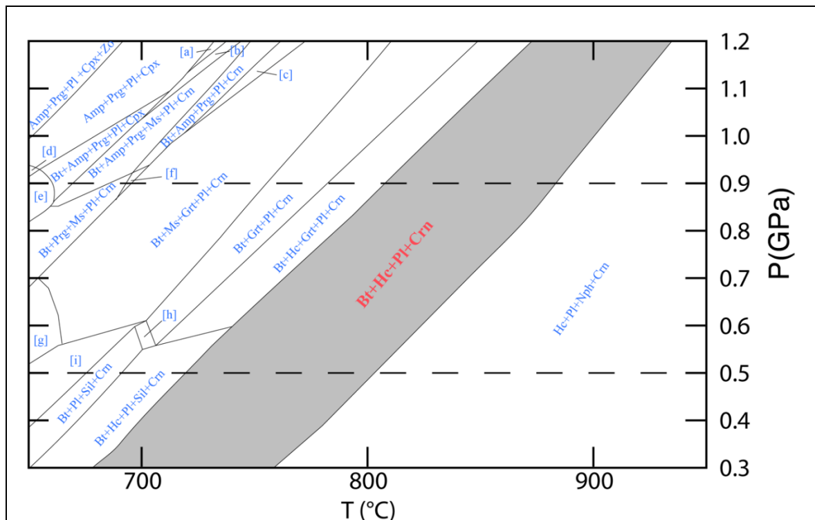
Figure 11 P-T pseudosection calculated for the chemical composition provided by Bertolani [13] for the plumasitic dyke recognized in Val Sabbiola, along the road to Montata village, which location and mineral assemblage correspond to our anorthosite SB08. The grey field corresponds to the mineral assemblage of SB08 rock. The dashed line indicates the pressure conditions estimated for the emplacement of the Mafic Complex during Carboniferous-Permian interval [72]. In the small stability field we reported the letters to indicate the mineral assemblage in those fields: [a]: Amp+Prg+Pl+Cpx+Crn; [b]: Bt+Amp+Prg+Pl+Cpx+Crn; [c]: Bt+Amp+Ms+Grt+Pl+Crn; [d]: Amp+Prg+Ms+Pl+Cpx; [e]: Bt+Amp+Prg+Ms+Pl+Cpx; [f]: Bt+Ms+Pl+Crn; [g]: Bt+St+Ms+Pl+Crn; [h]: Bt+Gt+Pl+Sil+Crn; [i]: Bt+Ms+Pl+Sill+Crn. Abbreviations after Whitney and Evans [27].
