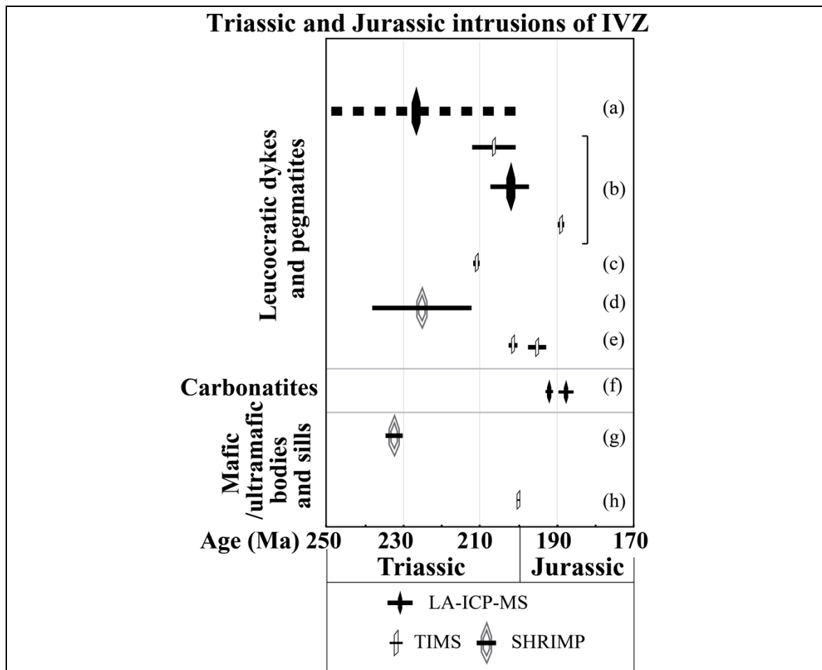
Figure 2. Schematic diagram showing U–Pb data from magmatic intrusions in the IVZ in the time span from Triassic to Jurassic. References: (a) [14]; (b) [22]; (c) [64]; (d) [20]; (e) [62]; (f) [59]; (g) [60]; (h) [57].
