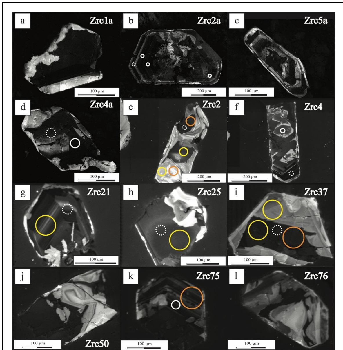
Figure 7 SEM-CL image of zircon grains for sample SB08. The spot analyses are reported as circles. : White dotted and solid circles refer to U–Pb concordant and discordant data, respectively; yellow and orange circles refer to trace element and Lu–Hf spot analyses.
