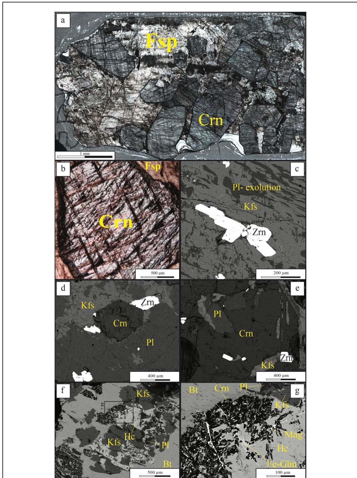
Figure 3. a) Scan of SB09 thin section (80µm thick) showing the magmatic/pegmatitic texture of the sample. b) photograph of an euhedral crystal of corundum. c) SEM-BSE image showing K-feldspar crystal with plagioclase exsolution and inclusions of zircon cluster. d) SEM-BSE image of the mineral assemblage consisting of plagioclase, K-feldspar, corundum and zircon. e) SEM-BSE image of zircons, K-feldspar and plagioclase inclusions within corundum. f) SEM-BSE image of poikilitic biotite hosting spinels, K-feldspar and plagioclase. g) Detail of f) showing reaction along the contact between biotite and hercynite consisting of corundum, magnetite and Fe-gahnite.
