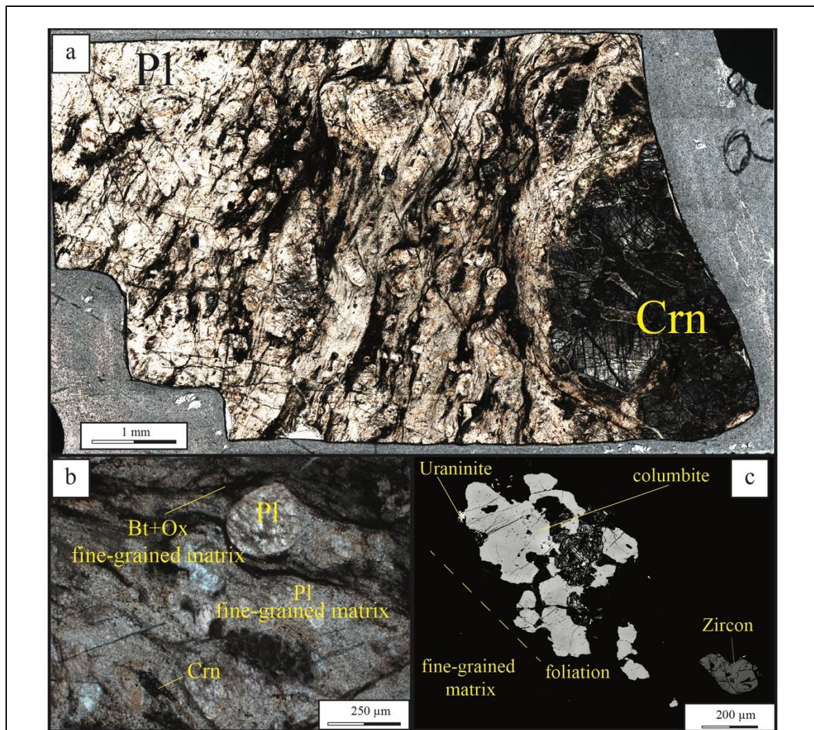
Figure 4. a) Scan of SB08 thin section (80µm thick) showing the porphyroclastic texture. b) Microphotograph of plagioclase porphyroclasts embedded within the fine-grained matrix consisting mainly of plagioclase, oxide, biotite and corundum. c) SEM-BSE image acquired with high contrast and low brightness showing columbite, zircon and uraninite within the fine-grained matrix.
