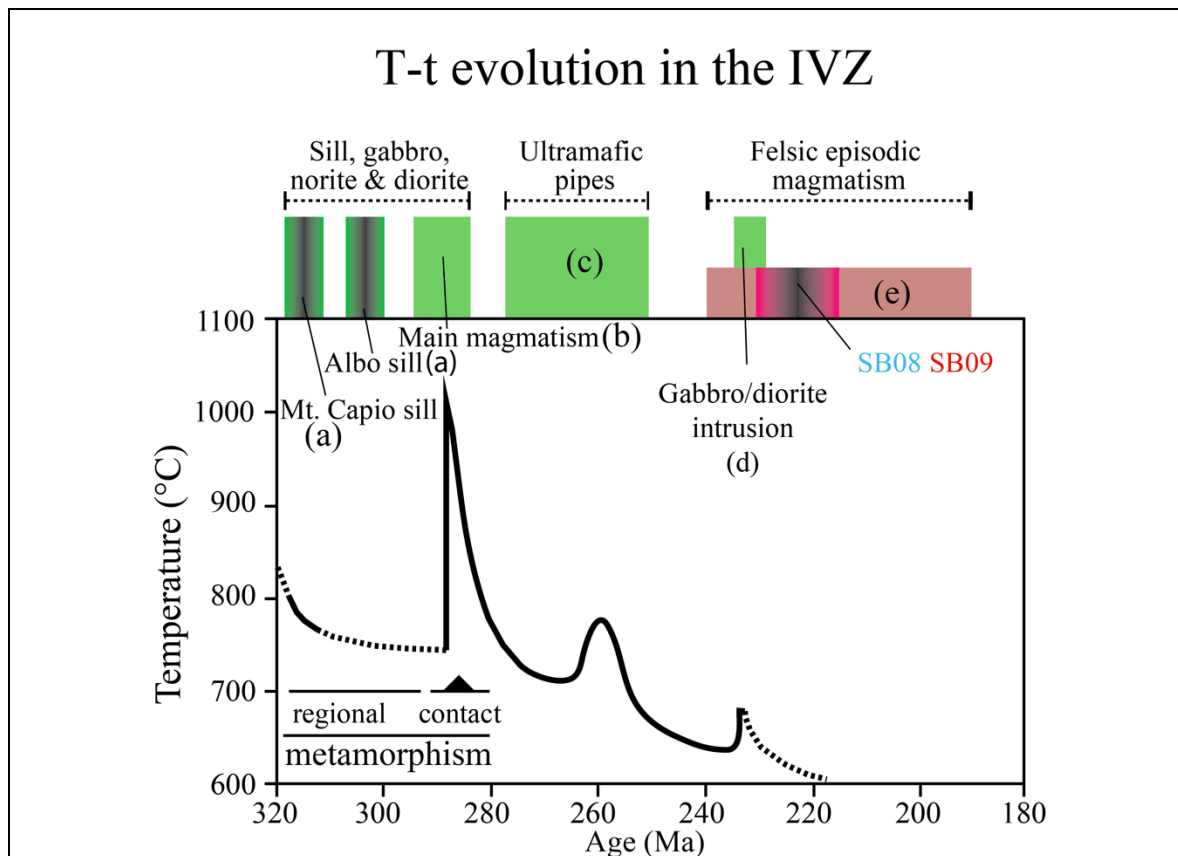
Figure 13 Temperature and time (T-t) plot for the central and southern part of IVZ, modified after Ewing et al., [51,115] and Klötzli et al. [53]. The black line indicates T-t evolution of high-grade metamorphic rocks. Magmatic events occurred in the IVZ from Permian to Jurassic are also shown at the top of the T-t plot. Green and pink boxes refer to zircon ^{206}\text{Pb}/^{238}\text{U} age data from mafic/ultramafic and felsic compositions, respectively. References: (a) [53]; (b) [49]; (c) [51,56,58] (d) [60]; (e) [14,20,22,62]. The intrusion age for the studied felsic dykes are also shown.
