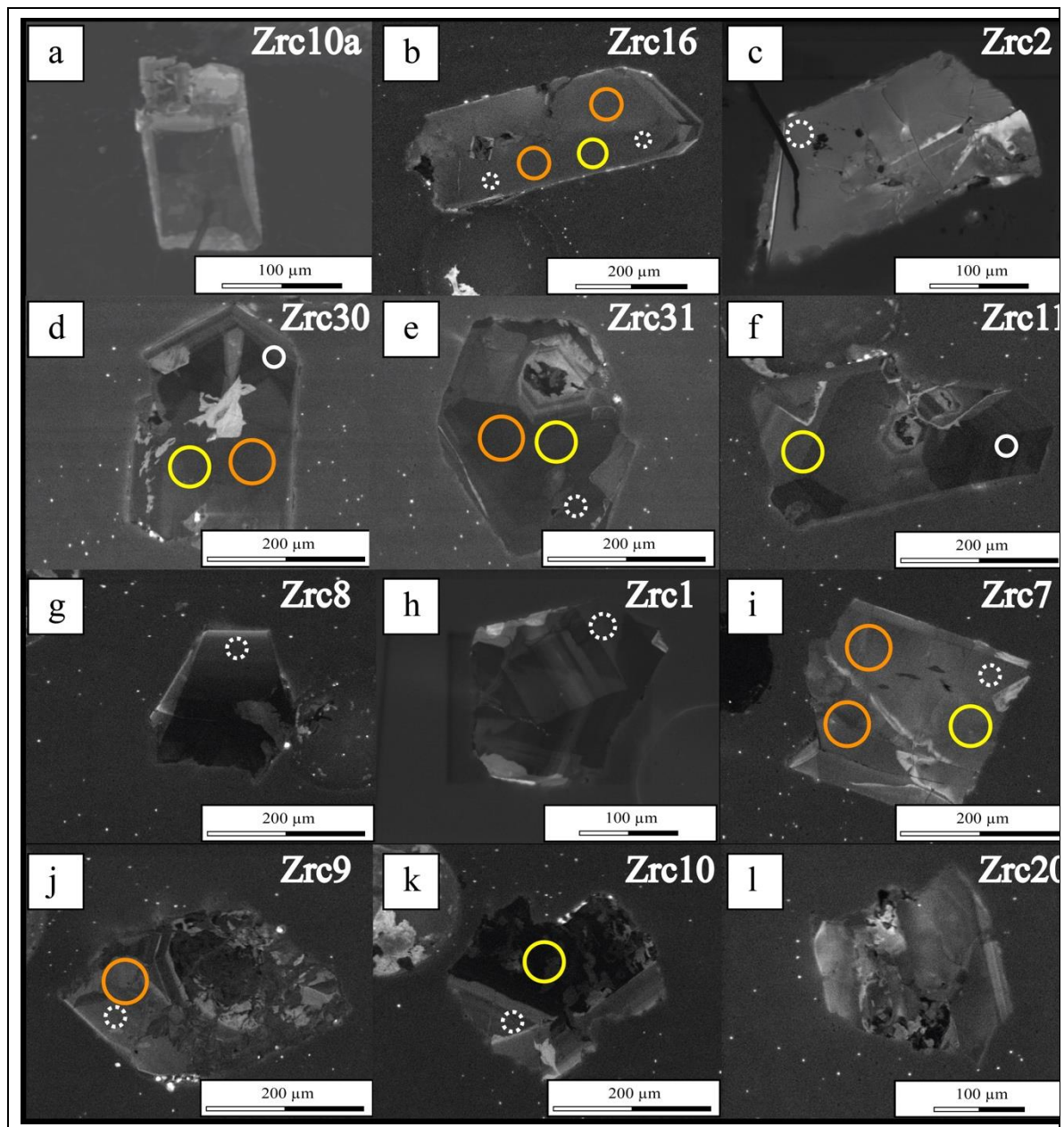
Figure 6 SEM-CL image of zircon grains for sample SB09. The spot analyses are reported as circles. : White dotted and solid circles refer to U–Pb concordant and discordant data, respectively; yellow and orange circles refer to trace element and Lu–Hf spot analyses.
