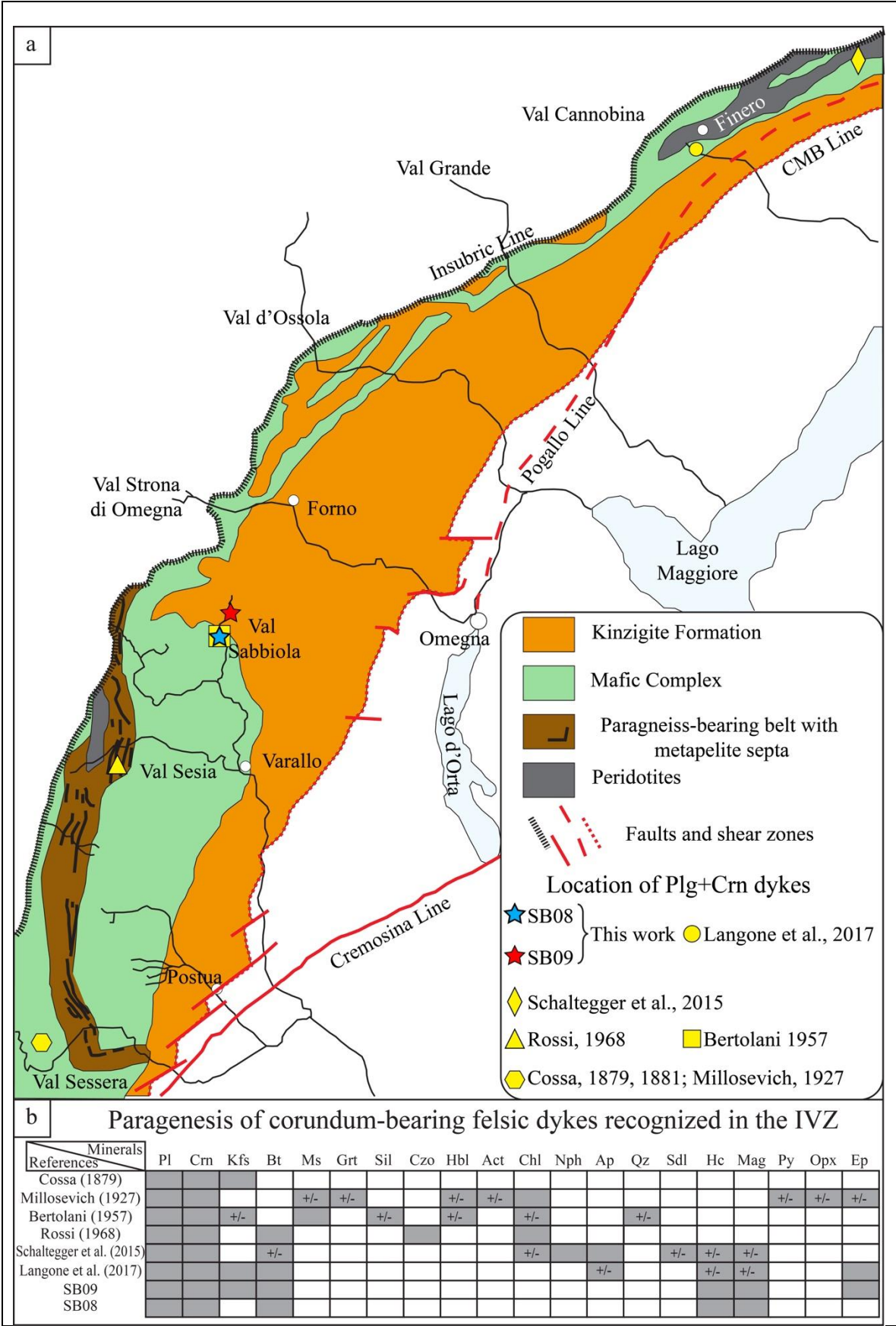
Figure 1. a) Geologic map of the Ivrea-Verbano Zone (modified after, Zingg [25] and Sinigoi [26]). The map shows the location of corundum-bearing dykes of the IVZ. b) Schematic table showing the mineral assemblages described for the felsic dykes in different samples and localities of the IVZ. Grey
