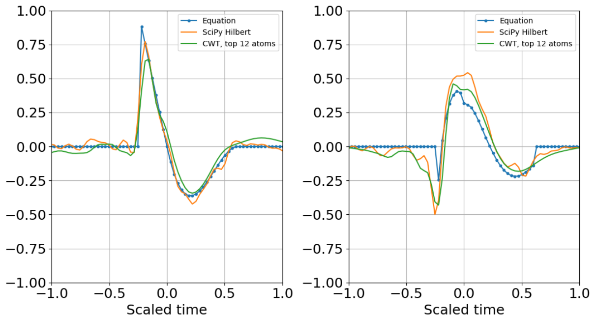
Figure 10. Superposition of largest coefficients per band within 4 bits of the peak SNR entropy. (a) Real part; (b) Imaginary part. Dimensionality is further reduced by applying the cutoff.
