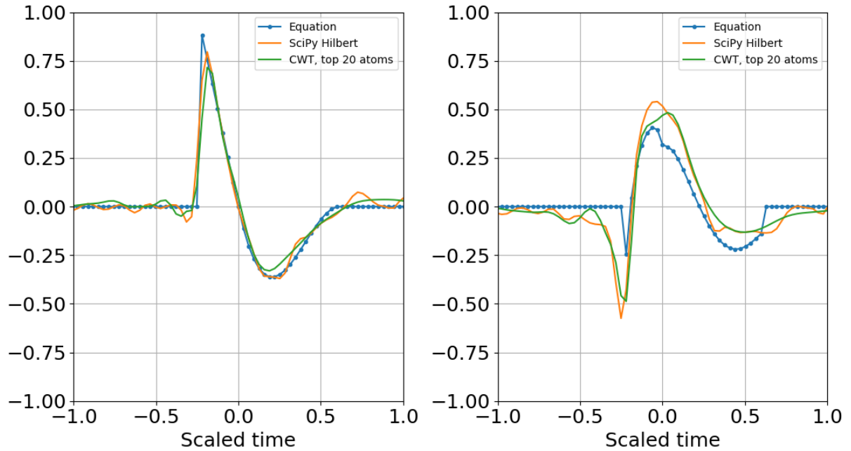
Figure 9. Superposition of largest SNR entropy coefficients per band using all twenty 1/3 octave bands. (a) Real part; (b) Imaginary part. The noise standard deviation is one bit below the signal's. Dimensionality is reduced to the number of coefficients and their corresponding time shifts.
