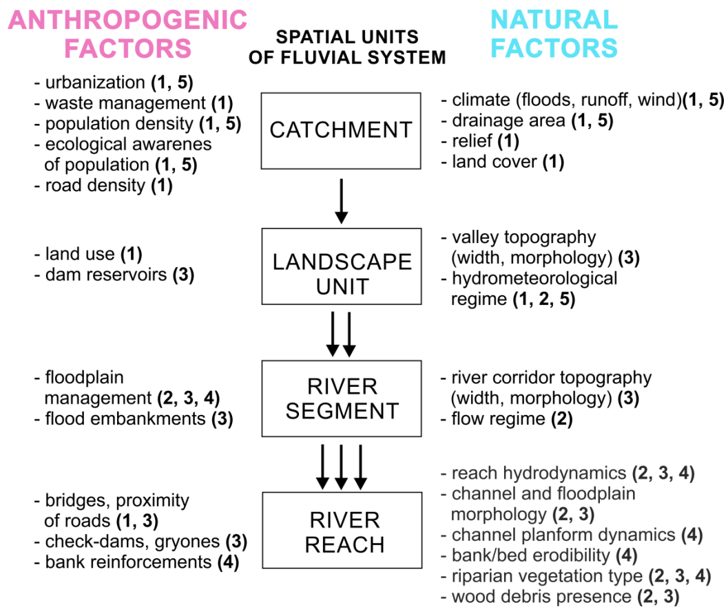
Figure 2. A scheme of anthropogenic and natural factors controlling particular phases of the macroplastic route in different spatial units of a fluvial system. 1 – input; 2 – transport; 3 – storage; 4 – remobilization; 5 – output. Arrows indicate the increasing number of controls on the fate of macroplastic debris from larger to smaller spatial units of a fluvial system.
