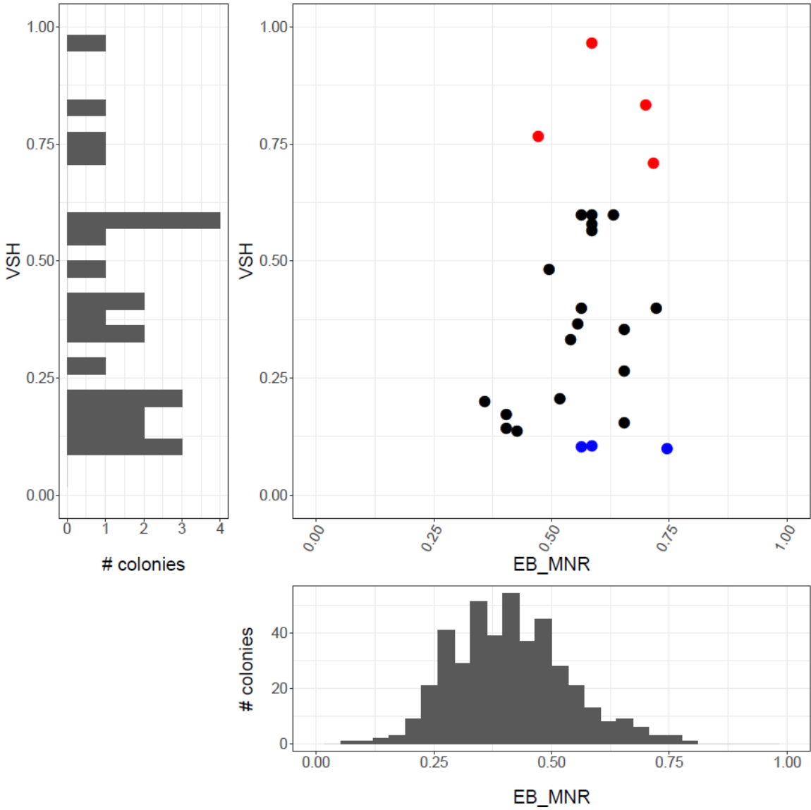
Figure S1. Scatterplot of VSH for EB_MNR values for the 26 colonies used to estimate correlation between these traits. Red points are the colonies with (significantly) high VSH and the blue points with (significantly) low VSH values. The histograms represent the distribution, in number of colonies, of VSH and EB_MNR.
